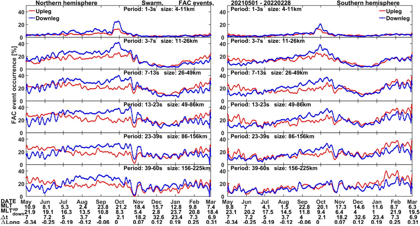
919 Figure 4. The same format as Figure 3, but for the occurrence frequency of positively detected 920 static FAC structures.
