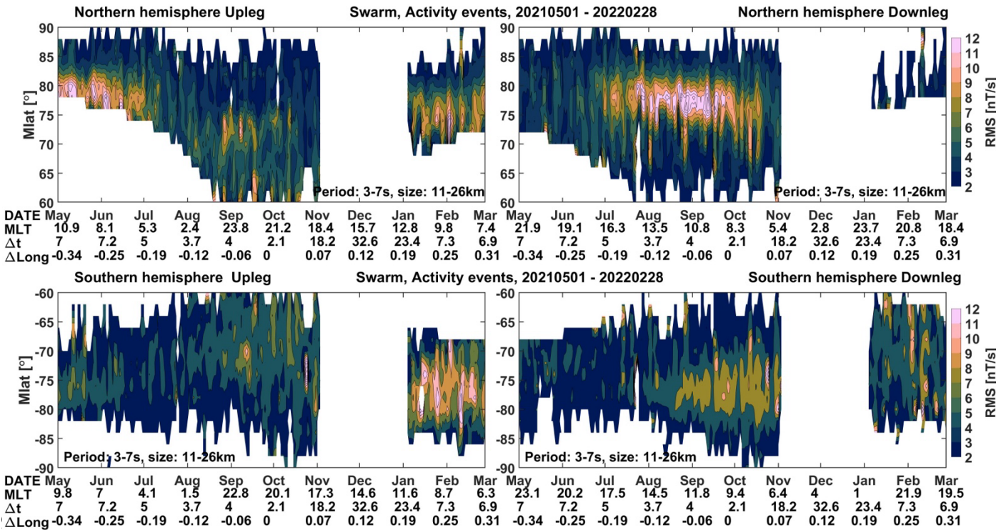
978 Figure 12. The same as Figure 9, but the amplitudes of all the events within the range of 979 d_{cross} < 6 km and \Delta t < 18 s are shown.
