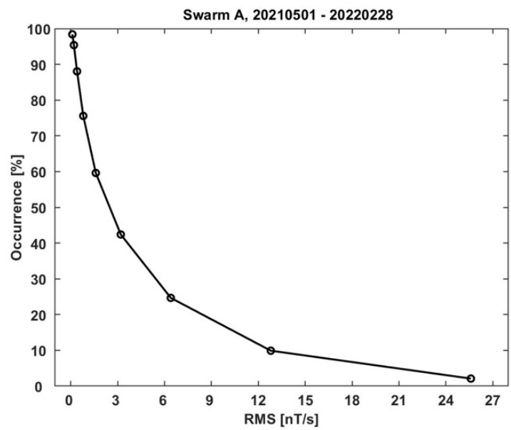
902 Figure 2. Occurrence distribution of transverse magnetic signature variations in the auroral region 903 with amplitudes above a certain RMS value. Here, signals in the period range 1- 60 s (4 - 220 km 904 along-track scale size) have been considered. For our FAC study amplitudes, RMS > 2 nT/s, are 905 required. With that, about 50% of the signals are taken into account.
