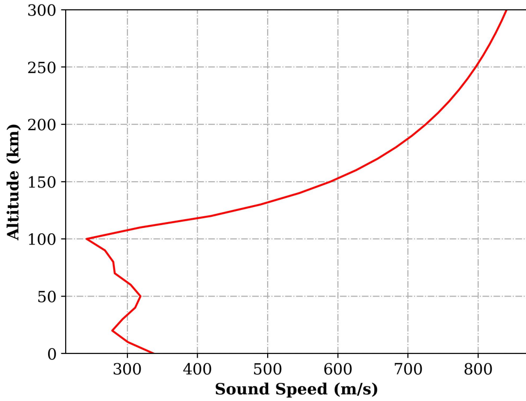
Figure S1: Sound speed profile at the epicentre for the day of earthquake
