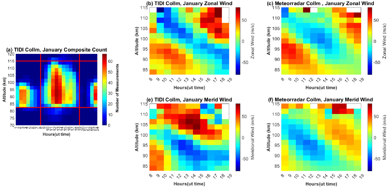
Figure 2. Comparison of TIDI and MR winds. Left panel: Number of successful TIDI measurements of the time of the day and altitude with the longitude and latitude bin where the MR is located. central panels: TIDI zonal and meridional daily composite winds, respectively. right panels: Zonal and meridional daily composite MR winds for Collm.
