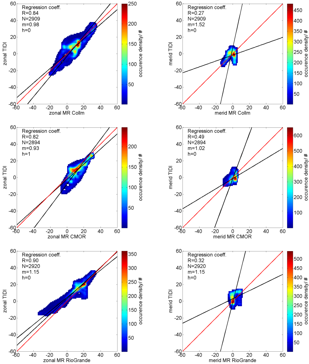
Figure 5. Correlation and density plots comparing the zonal mean zonal and meridional TIDI winds to the MR climatologies within the latitude bin for all mid-latitude stations COL, CMOR, and TdF (RioGrande). The red line denotes the ideal correlation. There are two fitting curves included in black. The red line is just to guide the reader to the 1 to 1 correlation. The black lines are the slopes to the data for both linear fits considering always the other variable as independent. The h describes the t-test result. h=1 indicates the null-hypothesis was rejected, h=0 reflects the acceptance of the null-hypothesis.
