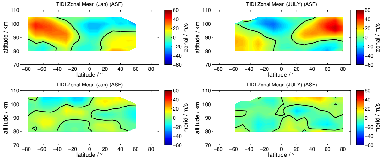
Figure 7. Latitudinal cross-section of zonal mean zonal winds and meridional winds from TIDI for January (left panel) and July (right panel).
