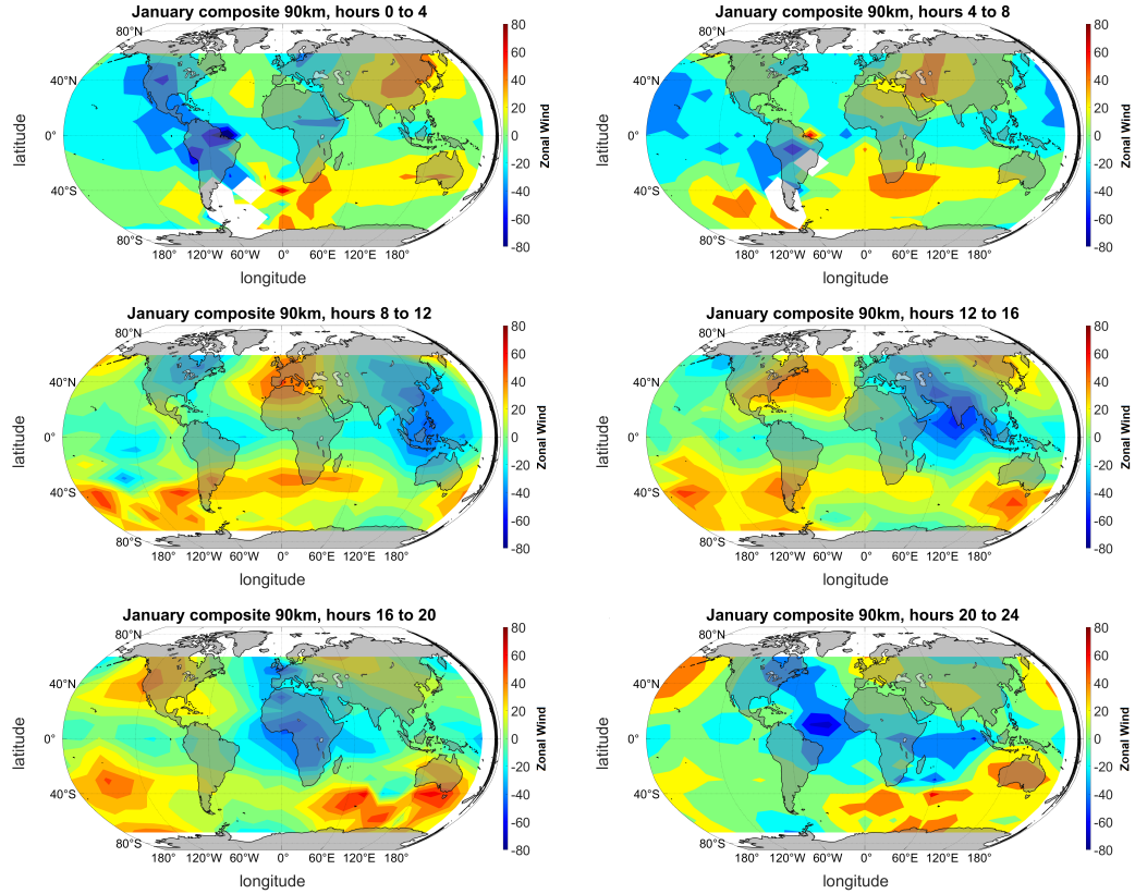
Figure 9. These pictures represent zonal winds for the composite month of January. These pictures are compiled based on 60-day averages using the quality criteria derived in this paper.
