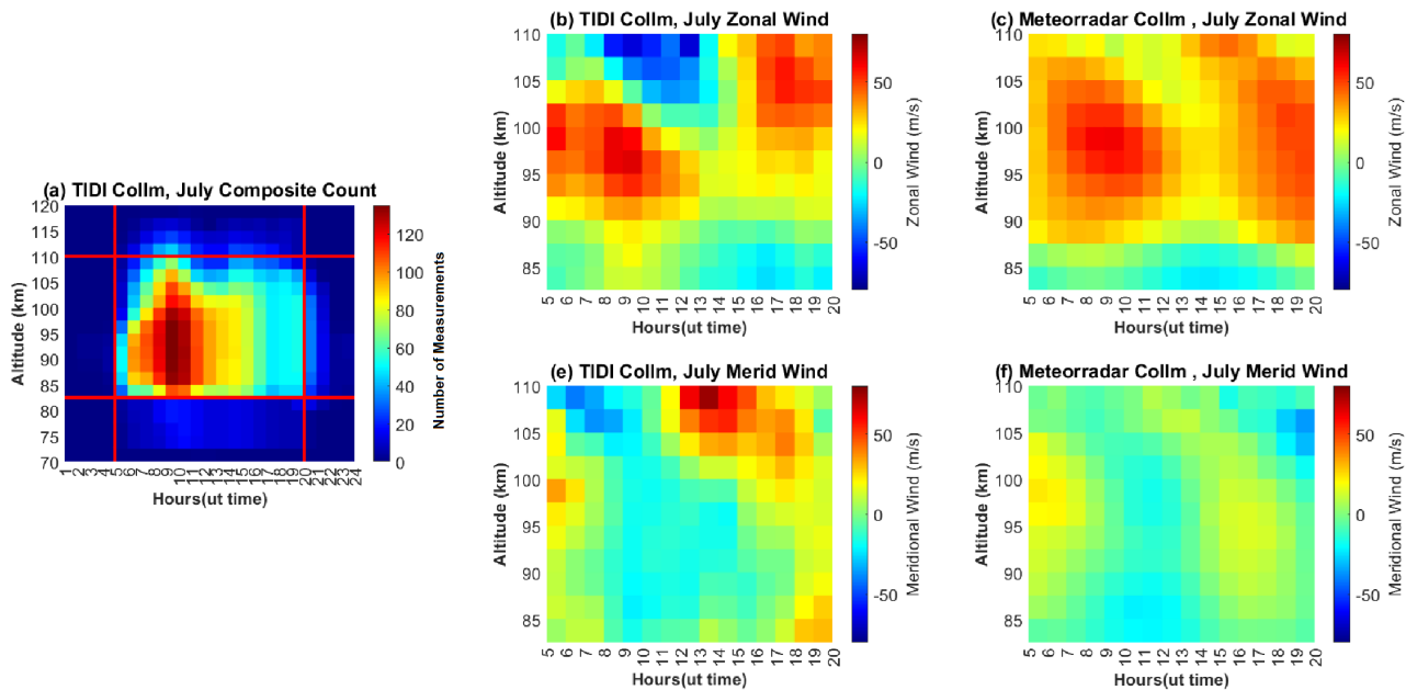
Figure 3. The same as Figure 2, but for July.
