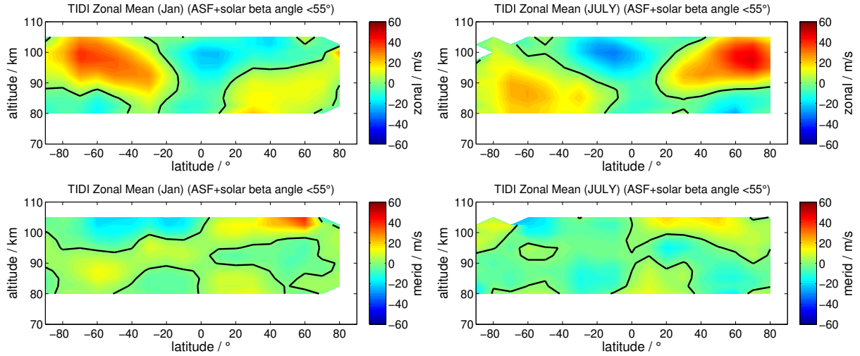
Figure 8. The same as Figure 7, but filtering the TIDI winds only for the solar beta angle (<55°).
