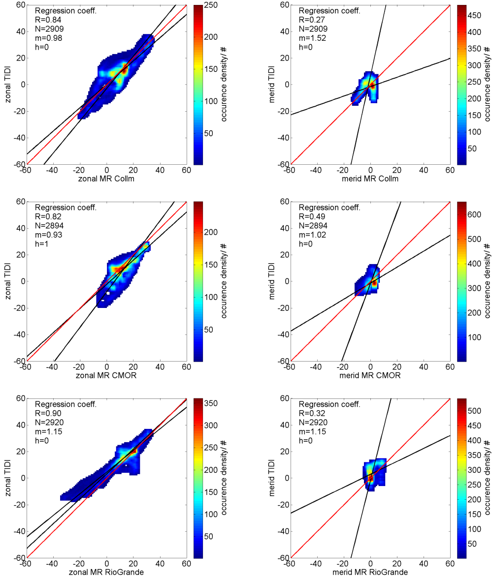
Figure 5. Correlation and density plots comparing the zonal mean zonal and meridional MR TIDI winds to the MR climatologies within the latitude bin for all mid-latitude stations COL, CMOR and TdF (RioGrande). The red line denotes the ideal correlation. There are two fitting curves included in black. The red line is just to guide the reader to the 1 to 1 correlation. The black lines are the slopes to the data for both linear fits considering always the other variable as independent. The h describes the t-test result. h=1 indicates the null-hypothesis was rejected, h=0 reflects the acceptance of the null-hypothesis.
