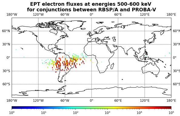
Figure 6. EPT electron differential fluxes [ \#/cm^2 s sr MeV] that follow the condition DL \leq 0.02 and DB \leq 0.01 between the L coordinates and the magnetic fields, respectively, of both satellites RBSP/A and PROBA-V. Left: 500-600 keV for the EPT and 558-639 keV for MagEIS. Right: 700-800 keV for EPT and 692-793 keV.
