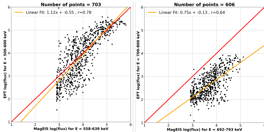
Figure 7. EPT electron differential fluxes [ \#/cm^2 s sr MeV] that follow the condition DL \leq 0.02 and DB \leq 0.01 between the L coordinates and the magnetic fields, respectively, of both satellites RBSP/A and PROBA-V.
