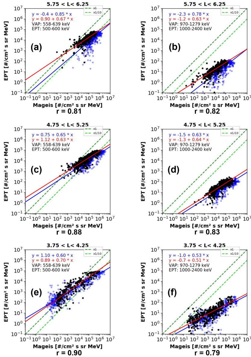
Figure 4. Scatterplot of the logarithm of the hour averaged differential electron fluxes from PROBA-V/EPT versus RBS-PB/RBSP-B /MageIS (blue dots for level 2 data and black dots for level 3 data (pitch angle of 8^\circ )) for two different energy channels (column 1: 500 keV, column 2: 1 MeV) and locations in the radiation belts (row 1: L \sim 6 \sim 6 , row 2: L \sim 5 \sim 5 , row 3: L \sim 4 \sim 4 ). Blue and red lines represent the best fit of the level 2 data and low pitch angle ( pa = 8^\circ ), respectively. The green lines show perfect linear correlation with a factor of \times 1 and \times 10^{-1} . Data represented in this graph are from January to March 2014. Pearson correlation coefficient and standard error below each panel are computed with low pitch angle values (i.e. black dot distributions).
