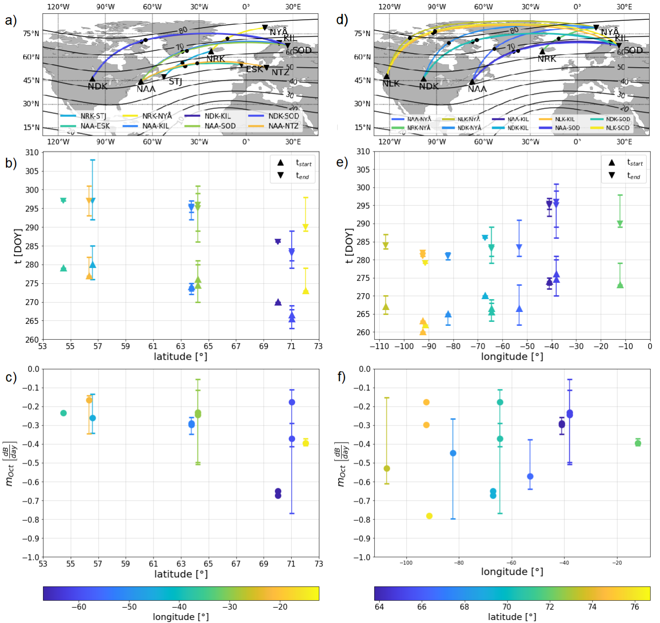
Figure 4. Latitudinal and longitudinal dependency of the October effect: a) and d) show maps with the used propagation paths. On the left (a-c) is the latitudinal dependency colour coded in longitude and on the right (d- f) the longitudinal dependency colour coded in latitude. b) and e) show the t_{start} (triangle up) and t_{end} (triangle down) of the October effect. The triangles are at the median and the lines show the spread of the values. c) and f) show the intensity m_{Oct} of the October effect.
