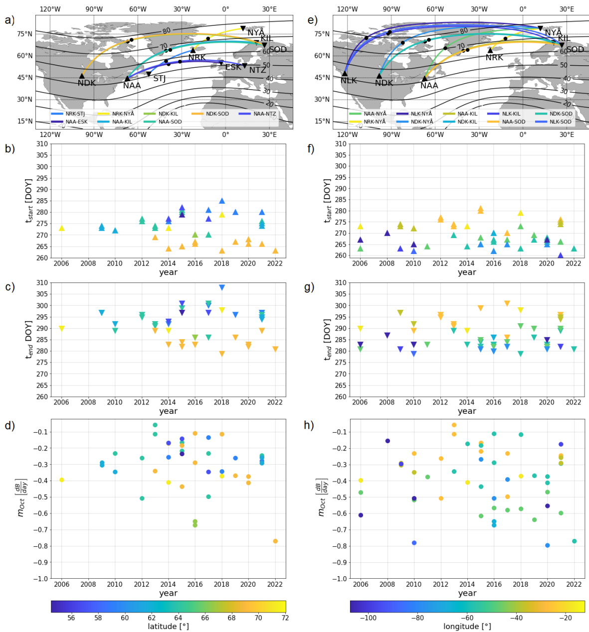
Figure 3. Yearly variations of the October effect: a) and e) show maps with the used propagation paths. On the left (a-d) is the yearly variation of the latitudinal dependency investigation colour coded in latitude and the right (e-h) the propagation paths for the longitudinal dependency investigation colour coded in longitude. b) and f) show t_{start} , c) and g) t_{end} , d) and h) the intensity m_{Oct} of the October effect.
