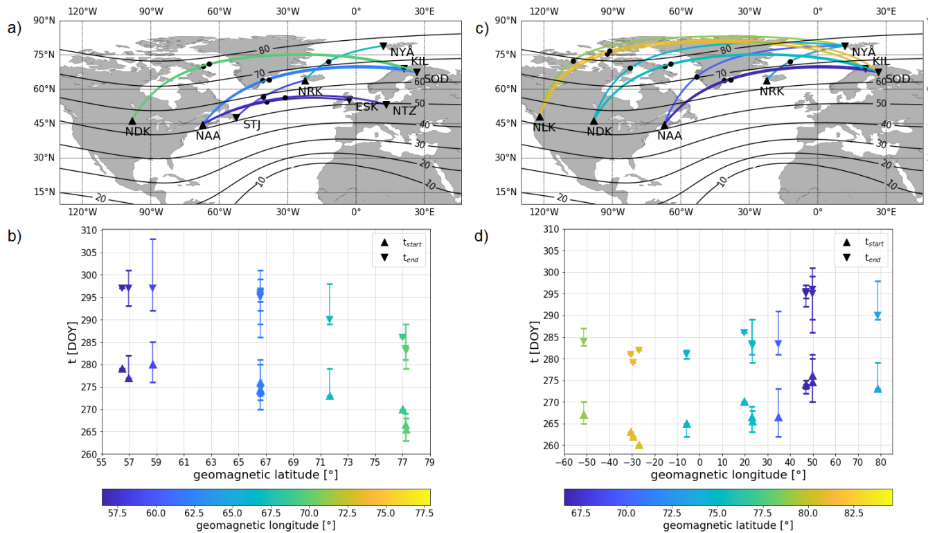
Figure 5. Dependency of the October effect on geomagnetic latitude and longitude: a) and c) show maps with the used propagation paths. On the left (a-b) is the geomagnetic latitudinal dependency colour coded in geomagnetic longitude and the right (c- d) the geomagnetic longitudinal dependency colour coded in geomagnetic latitude. b) and d) show the t_{start} (triangle up) and t_{end} (triangle down) of the October effect. The triangles are at the median and the lines show the spread of the values.
