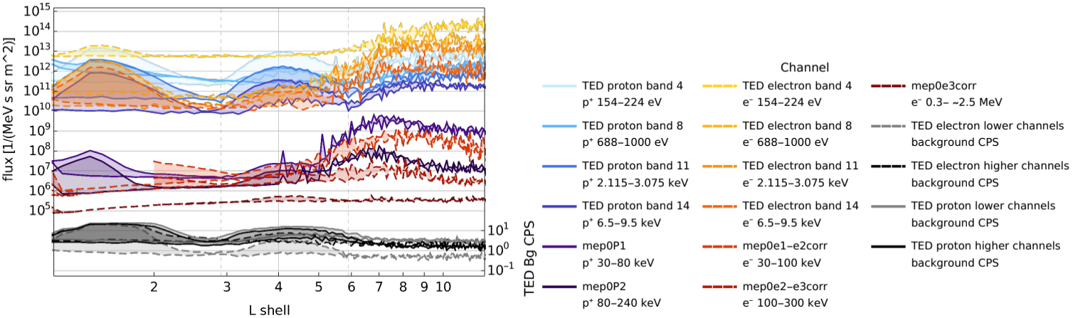
Particle flux at 60° and 160° mag. longitude FF (year 2013, Kp<=0.7)
