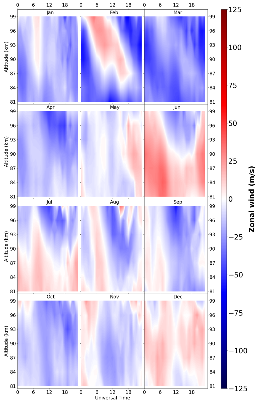
Figure 5. Monthly time variation of averaged zonal wind calculated using the meteor radar for 2006.
