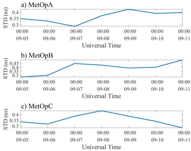
455 Figure 15. STD of DCB from LSS method for MetOpA, MetOpB and MetOpC, respectively.
