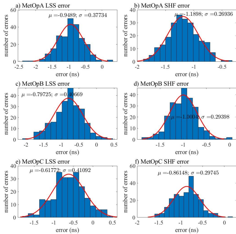
Figure 12. Frequency statistics of LSS and SHF error numbers with LSS assumption and SHF method based on MetOpA, MetOpB, and MetOpC data during 20190909-20190918, respectively.
