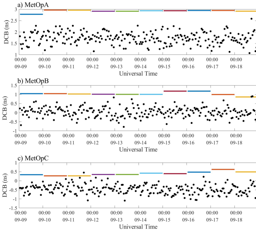
440 Figure 8. Distribution of DCB time series. The lines are the reference value of MetOpA, MetOpB, and MetOpC from CDAAC, and the scatters are the calculated value by SHF method. Different color of lines represents different days reference value from CDAAC.
