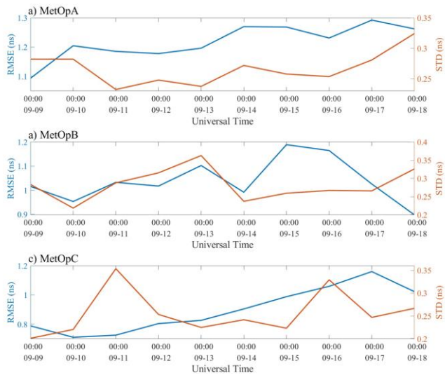
Figure 10. RMSE and STD of DCB calculated by SHF assumption for MetOpA, MetOpB and MetOpC, respectively.
