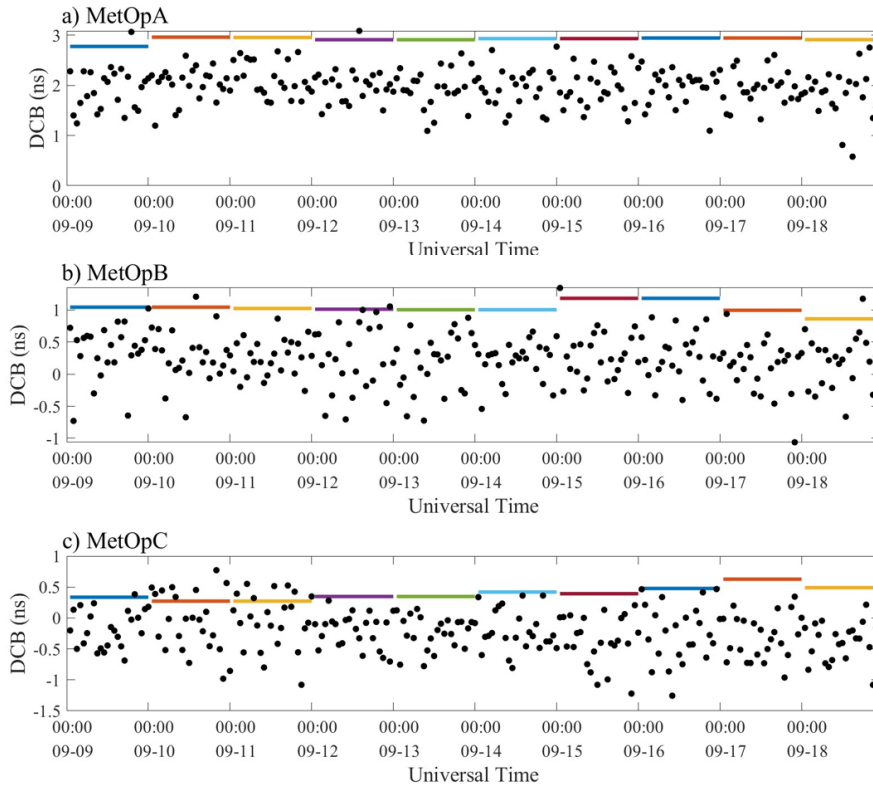
435 Figure 7. Distribution of DCB time series. The lines are the reference value of MetOpA, MetOpB, and MetOpC from CDAAC, and the scatters are the calculated DCB based on LSS method. Different colors of lines represent different days reference value from CDAAC.
