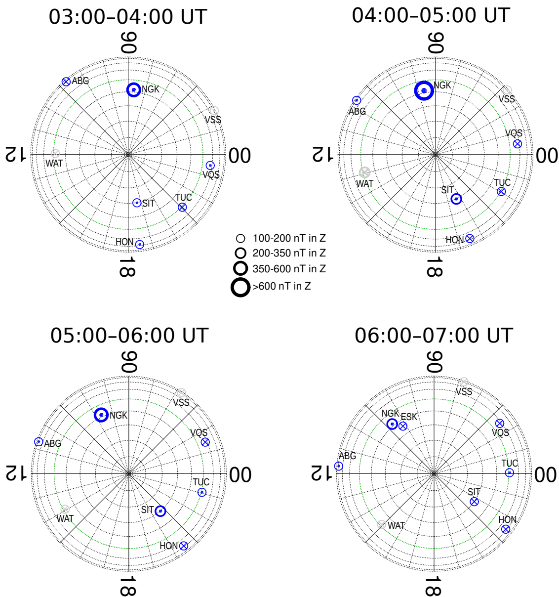
Figure 5. Evolution of variations in the vertical intensity on 15 May 1921 between 03:00 UT and 07:00 UT. A polar coordinate system is used here: the radial coordinate is the geomagnetic latitude (CGC or QDP), the distance between the individual parallels in the graphs is set to 10^\circ , and the angular coordinate is the magnetic local time. The parallel drawn in green represents the corrected geomagnetic latitude at which the most equatorward observed overhead aurora was reported during the May 1921 storm.
