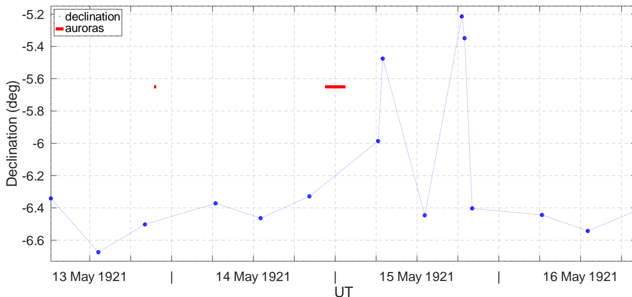
Figure 2. Geomagnetic disturbance recorded in magnetic declination on 13–16 May 1921 at observatory Clementinum in Prague. The times are also indicated when auroras were observed in former Czechoslovakia. (After the data by Swoboda, 1921).
