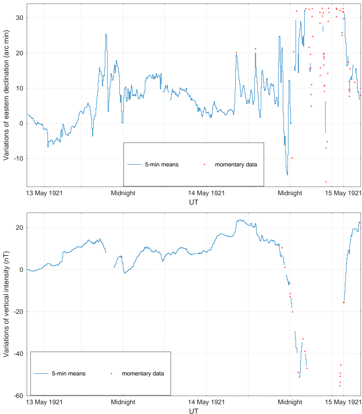
Figure 1. The records of magnetic declination and vertical intensity in Stará Ďala for the storm of 15 May 1921. The five-minute means, as well as some important momentary values are displayed.
