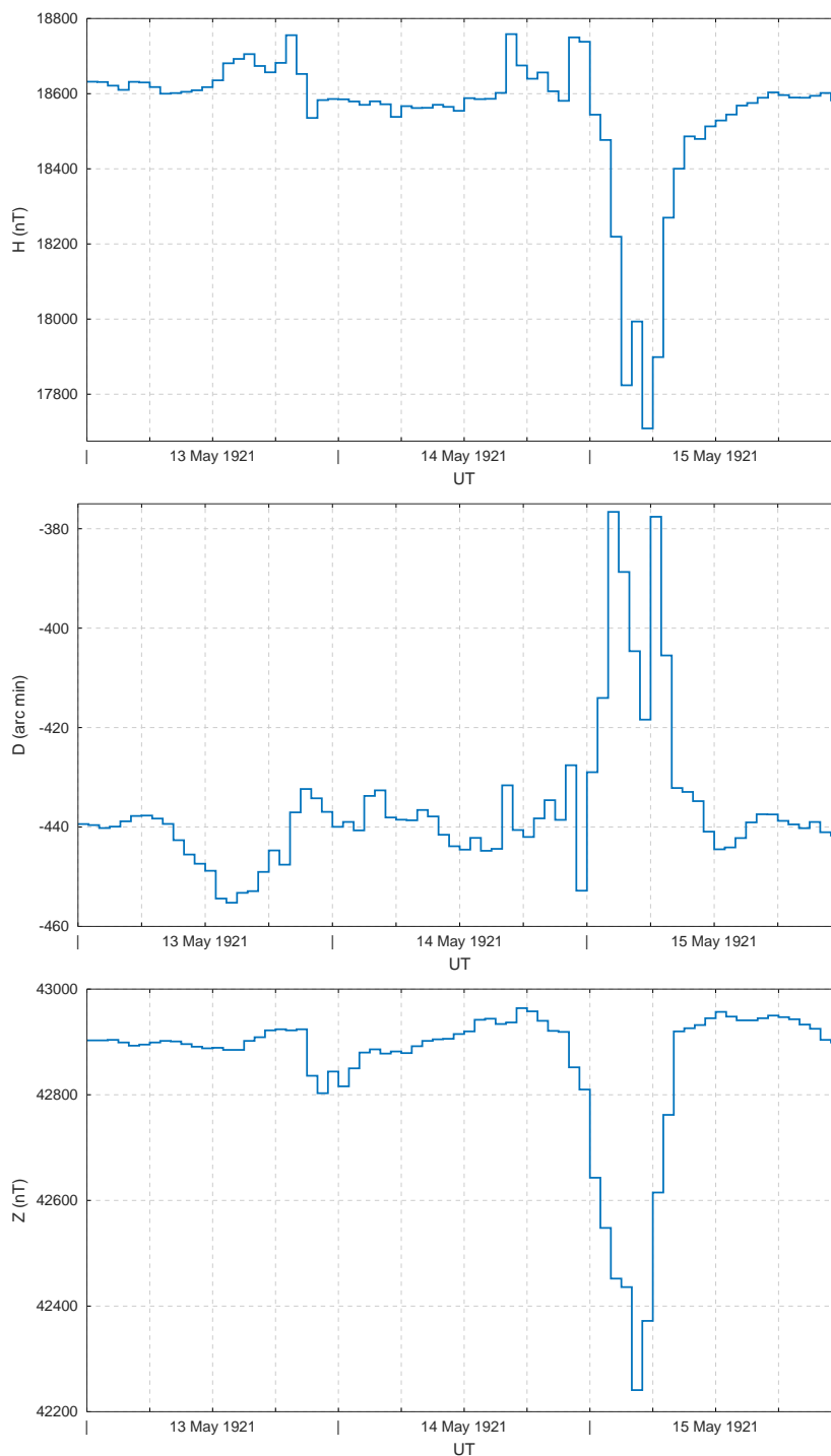
Figure 3. One-hour means of the geomagnetic elements from observatories Potsdam/Seddin for the period 13-15 May 1921. The following elements are displayed: horizontal intensity (H, upper panel), declination (D, middle panel), and vertical intensity (Z, bottom panel).
