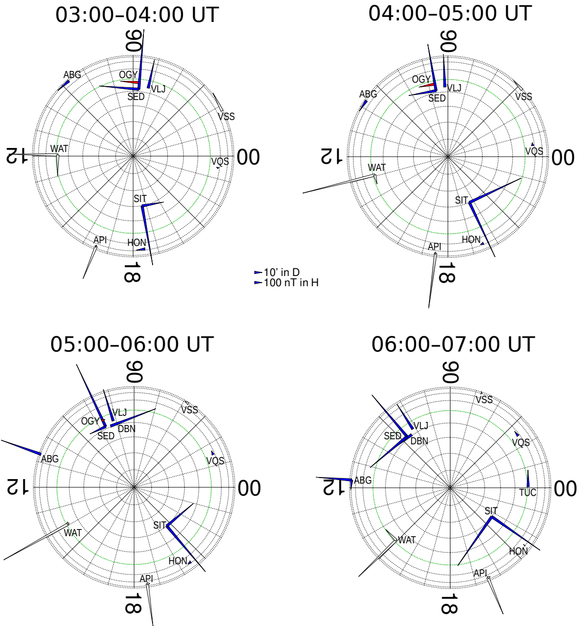
Figure 5. Evolution of variations in the horizontal intensity and magnetic declination on 15 May 1921 between 03:00 UT and 07:00 UT. A polar coordinate system is used here: the radial coordinate is the geomagnetic (QDP) latitude, the distance between the individual parallels in the graphs is set to 10^\circ , and the angular coordinate is the magnetic local time. The parallel drawn in green represents the QDP latitude at which the most equatorward observed overhead aurora was reported during the May 1921 storm.
