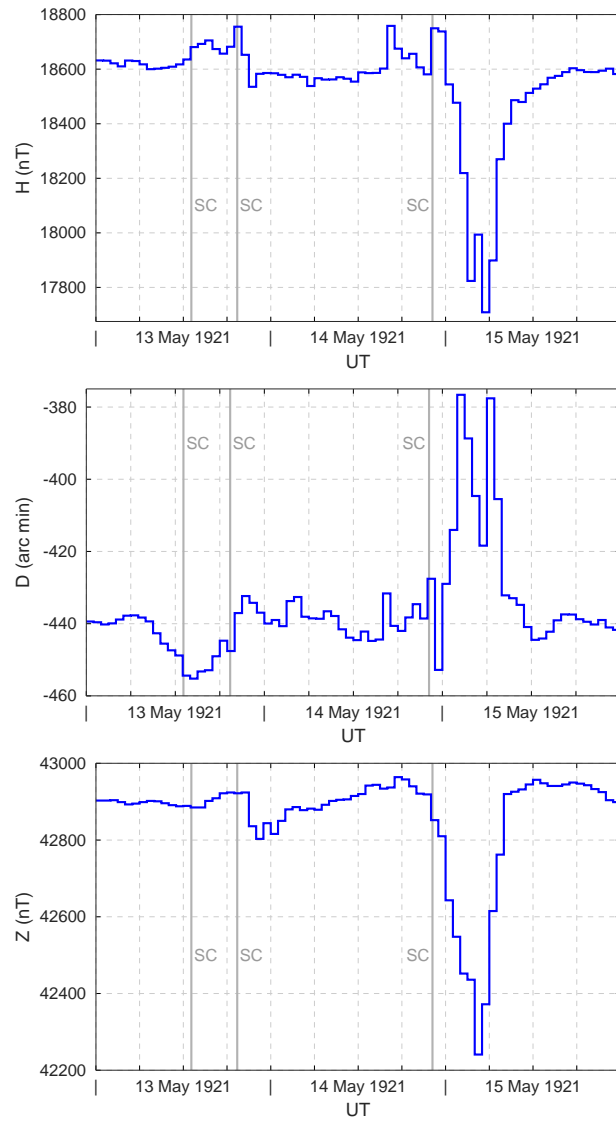
Figure 4. Hourly means of the geomagnetic elements from the observatory Seddin for the period 13-15 May 1921. The following elements are displayed: horizontal intensity ( H , upper panel), declination ( D , middle panel), and vertical intensity ( Z , bottom panel). The times of the occurrences of the sudden commencements according to Mayaud (1973) are also indicated.
