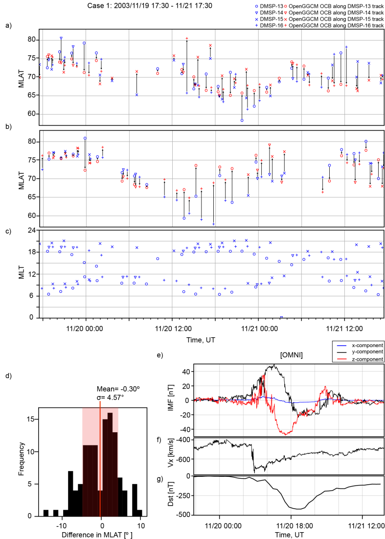
Figure 1. Comparison between the observed and simulated OCB latitudes for November 20, 2003 event. Panel a) shows the DMSP based OCB latitude in blue and corresponding OpenGGCM OCB latitude in red for all passes of the northern polar cap. Panel b) shows the DMSP based OCB latitude in blue and corresponding OpenGGCM OCB latitude in red for all passes of the southern polar cap. Panel c) indicates the coverage of the DMSP satellites for this event. A histogram of the differences between the observed and simulated OCB latitudes is shown in panel d). Panels e) and f) show the solar wind and IMF data used as input for the simulations. Panel g) shows the Dst index. The solar wind and IMF values are in GSE coordinates and were obtained from OMNIWeb.
