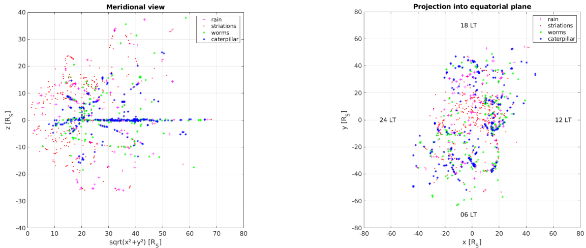
Figure 8. Meridional (left) and equatorial distribution (right) of Cassini positions from where SKR of the SPEC class (rain, striations, worms, caterpillars) was observed below 80 kHz.
