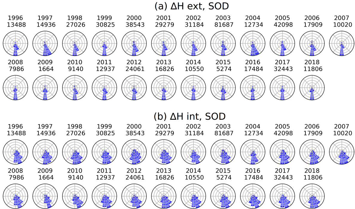
Figure 7. Directional distribution of (a) \Delta\mathbf{H}_{ext} and (b) \Delta\mathbf{H}_{int} at Sodankylä (SOD) between 1996-2018 when |\mathrm{d}\Delta\mathbf{H}/\mathrm{d}t| > 1 \text{ nTs}^{-1} . The number of data points is plotted below the year label.
