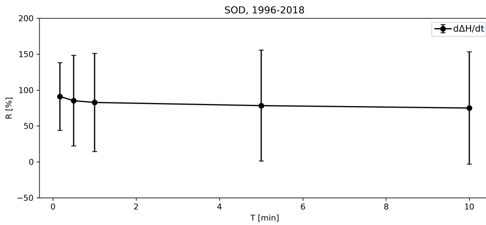
Figure B3. Mean values and standard deviation of R(T) (relative change in amplitude) for total d\Delta H/dt at SOD. Data from 1996 to 2018, and T = 10 \text{ s} \dots 10 \text{ min} .
