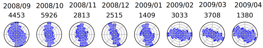
Figure A2. Monthly directional distributions of internal d\Delta\mathbf{H}/dt at Kevo (KEV), 2008/09 to 2009/04. The number of data points is plotted under the year and month label. |d\Delta\mathbf{H}/dt| > 0.5 \text{ nTs}^{-1} .
