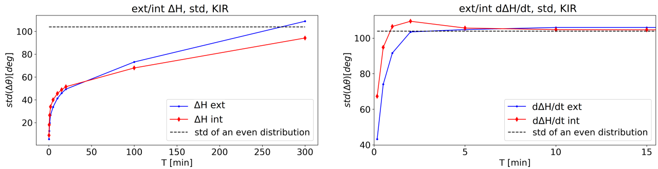
Figure B2. Standard deviation of \Delta\theta at different time periods, T , using a threshold value 0.5 \text{ nTs}^{-1} < |d\Delta H/dt| < 1 \text{ nTs}^{-1} . Left panel: external and internal \Delta H , right panel: external and internal d\Delta H/dt .
