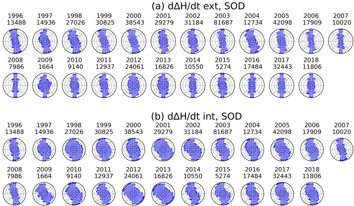
Figure 8. Directional distribution of (a) d\Delta\mathbf{H}_{ext}/dt and (b) d\Delta\mathbf{H}_{int}/dt at Sodankylä (SOD) 1996–2018 when |\Delta\mathbf{H}/dt| > 1 \text{ nTs}^{-1} . The number of data points is plotted below the year label.
