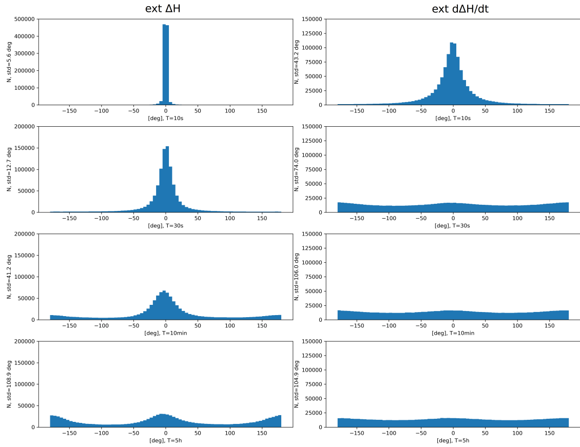
Figure B1. Histograms of \Delta\theta at KIR at different time periods, T , using a threshold value 0.5 \text{ nTs}^{-1} < |d\Delta H/dt| < 1 \text{ nTs}^{-1} . On left: external \Delta H , on right: external d\Delta H/dt .
