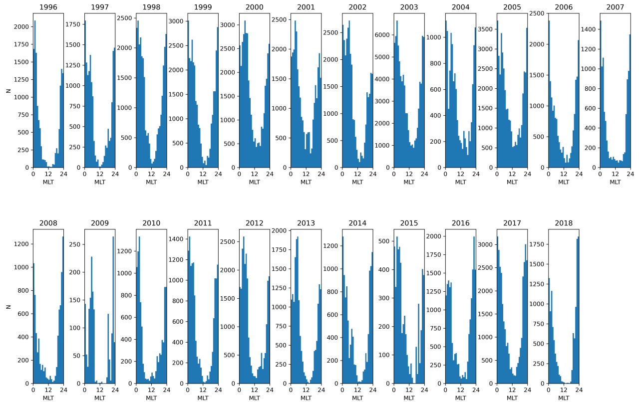
Figure 9. MLT distribution of the number of events ( N ) fitting the |\mathrm{d}\Delta\mathbf{H}/\mathrm{d}t| > 1 \text{ nTs}^{-1} criterion. Sodankylä (SOD), 1996–2018.
