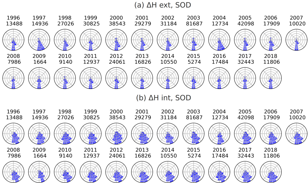
Figure 7. Directional distribution of (a) \Delta\mathbf{H}_{ext} and (b) \Delta\mathbf{H}_{int} at Sodankylä (SOD) between 1996-2018 when |\mathrm{d}\Delta\mathbf{H}/\mathrm{d}t| > 1 \text{ nTs}^{-1} . The number of data points is plotted below the year label.
