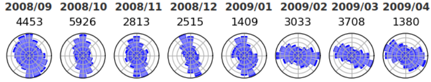
Figure A2. Monthly directional distributions of internal d\Delta\mathbf{H}/dt at Kevo (KEV), 2008/09 to 2009/04. The number of data points is plotted under the year and month label. |d\Delta\mathbf{H}/dt| > 0.5 \text{ nTs}^{-1} .
