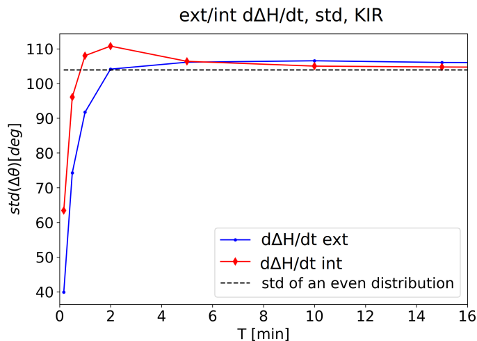
Figure 12. Standard deviations of \Delta\theta for the external (blue line with dot markers) and internal (red line with diamond markers) d\Delta\mathbf{H}/dt as a function of T at Kiruna (KIR). Threshold value for chosen events is |d\Delta\mathbf{H}/dt| > 1 \text{ nTs}^{-1} .
