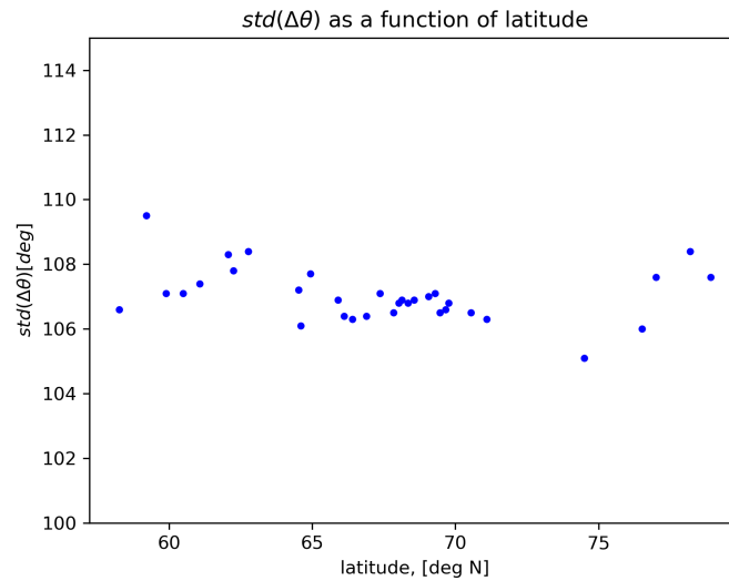
Figure 14. Standard deviation of \Delta\theta for external d\Delta\mathbf{H}/dt at IMAGE stations as a function of latitude. Data from 1996 to 2018, and T = 10 min.
