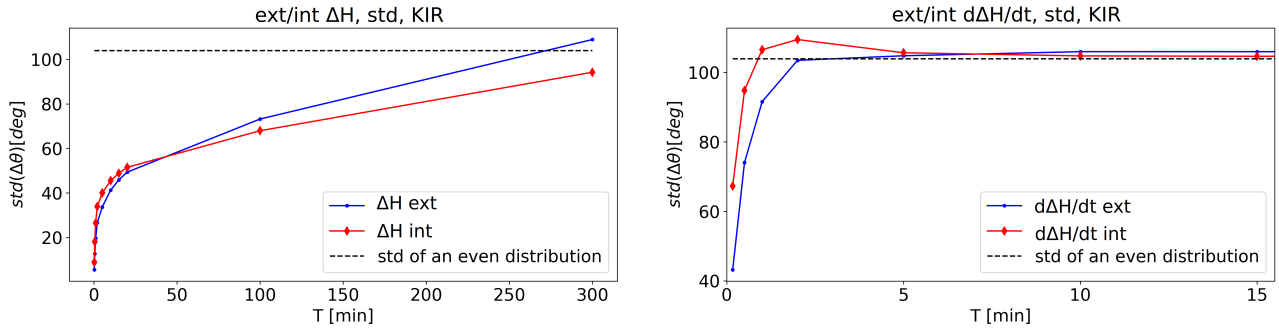
Figure B2. Standard deviation of \Delta\theta at different time periods, T , using a threshold value 0.5 \text{ nTs}^{-1} < |d\Delta\mathbf{H}/dt| < 1 \text{ nTs}^{-1} . Left panel: external and internal \Delta\mathbf{H} , right panel: external and internal d\Delta\mathbf{H}/dt .
