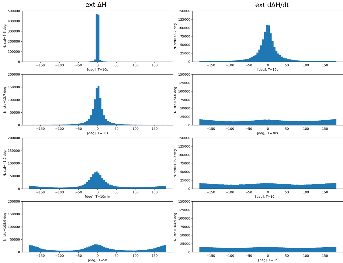
Figure B1. Histograms of \Delta\theta at KIR at different time periods, T , using a threshold value 0.5 \text{ nTs}^{-1} < |d\Delta\mathbf{H}/dt| < 1 \text{ nTs}^{-1} . On left: external \Delta\mathbf{H} , on right: external d\Delta\mathbf{H}/dt .
