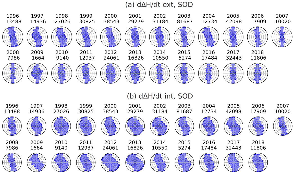
Figure 8. Directional distribution of (a) d\Delta\mathbf{H}_{ext}/dt and (b) d\Delta\mathbf{H}_{int}/dt at Sodankylä (SOD) 1996–2018 when |d\Delta\mathbf{H}/dt| > 1 \text{ nTs}^{-1} . The number of data points is plotted below the year label.
