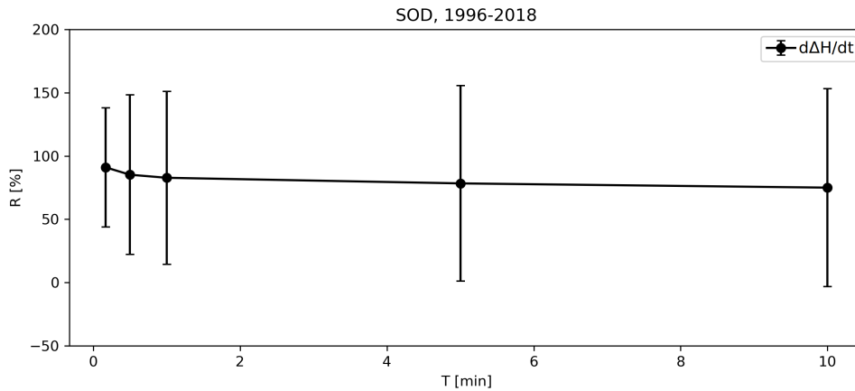
Figure B3. Mean values and standard deviation of R(T) (relative change in amplitude) for total d\Delta\mathbf{H}/dt at SOD. Data from 1996 to 2018, and T = 10 \text{ s} \dots 10 \text{ min} .
