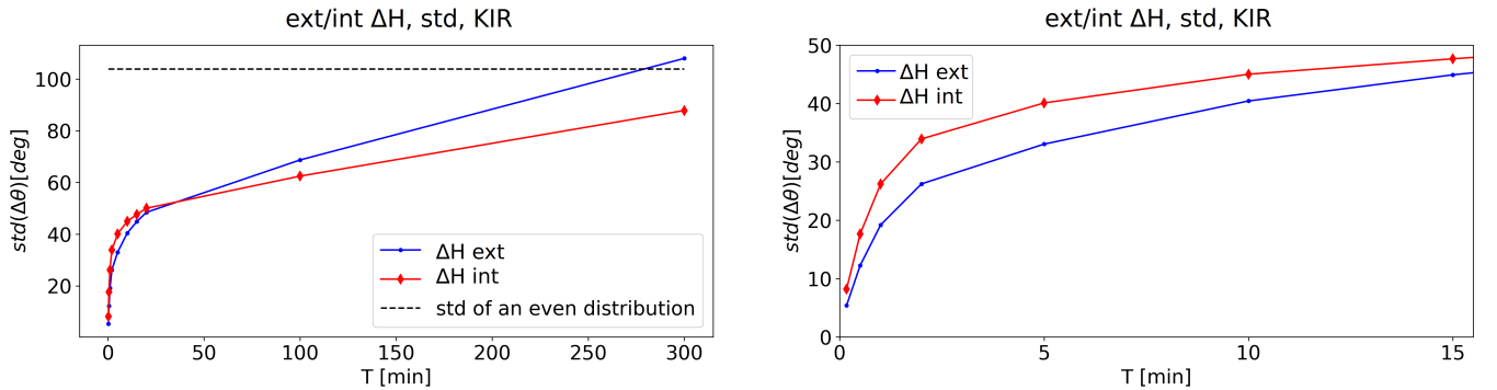
Figure 11. Standard deviations of \Delta\theta for the external (blue line with dot markers) and internal (red line with diamond markers) \Delta\mathbf{H} as a function of T at Kiruna (KIR). Threshold value for chosen events is |d\Delta\mathbf{H}/dt| > 1 \text{ nTs}^{-1} . On the left, T range is from 0 to 300 min, a closeup on the first 15 min is shown on the right.
