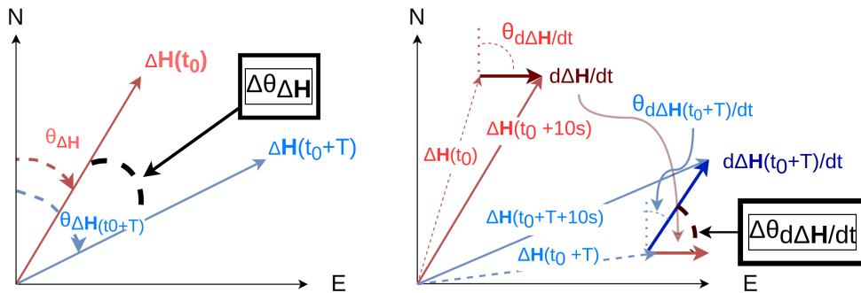
Figure 2. A schematic of the quantity \Delta\theta for \Delta\mathbf{H} , and its time derivative, d\Delta\mathbf{H}/dt used in this study. \Delta\mathbf{H}(t) refers to the baseline subtracted magnetic field vector at a specific time, t . \theta(t) refers to the angle between \Delta\mathbf{H}(t) and the geographic north. T is a multiple of the data sampling interval (10 s).
