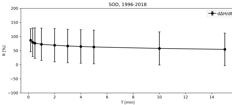
Figure 15. Mean values (black markers) and standard deviation (bars) of relative change in amplitude, R(T) , of total d\Delta\mathbf{H}/dt at SOD. Data from 1996 to 2018, and T = 10 s ... 15 min.
