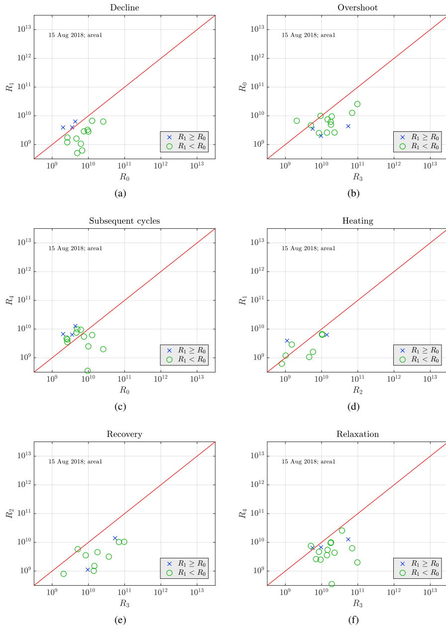
Figure S20. Comparison of the power amplitudes observed on the 15 August 2018 in Area 1.
