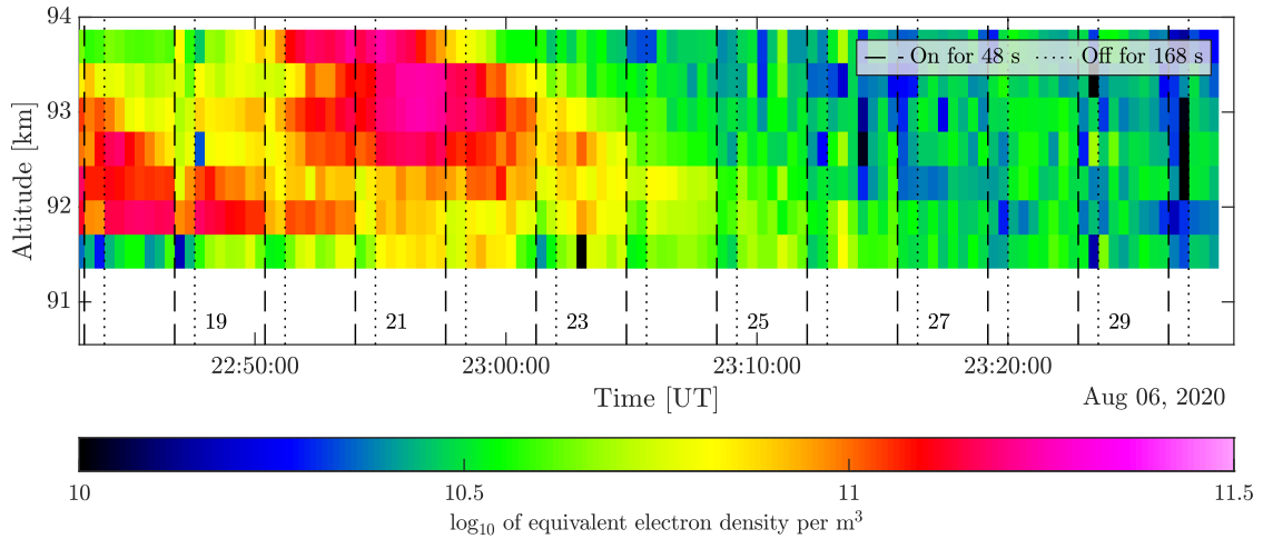
Figure S11. Back scattered power as function of altitude and heating intervals observed during the night of August 06/07, 2020 in Area 2. It should be noted that other limits of the colour scale have been chosen for this plot.
