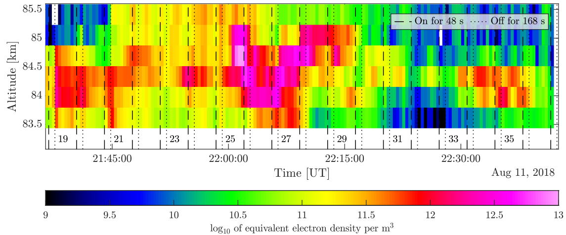
Figure S1. Back scattered power as function of altitude and heating intervals observed during the night of August 11/12, 2018 in Area 1.
