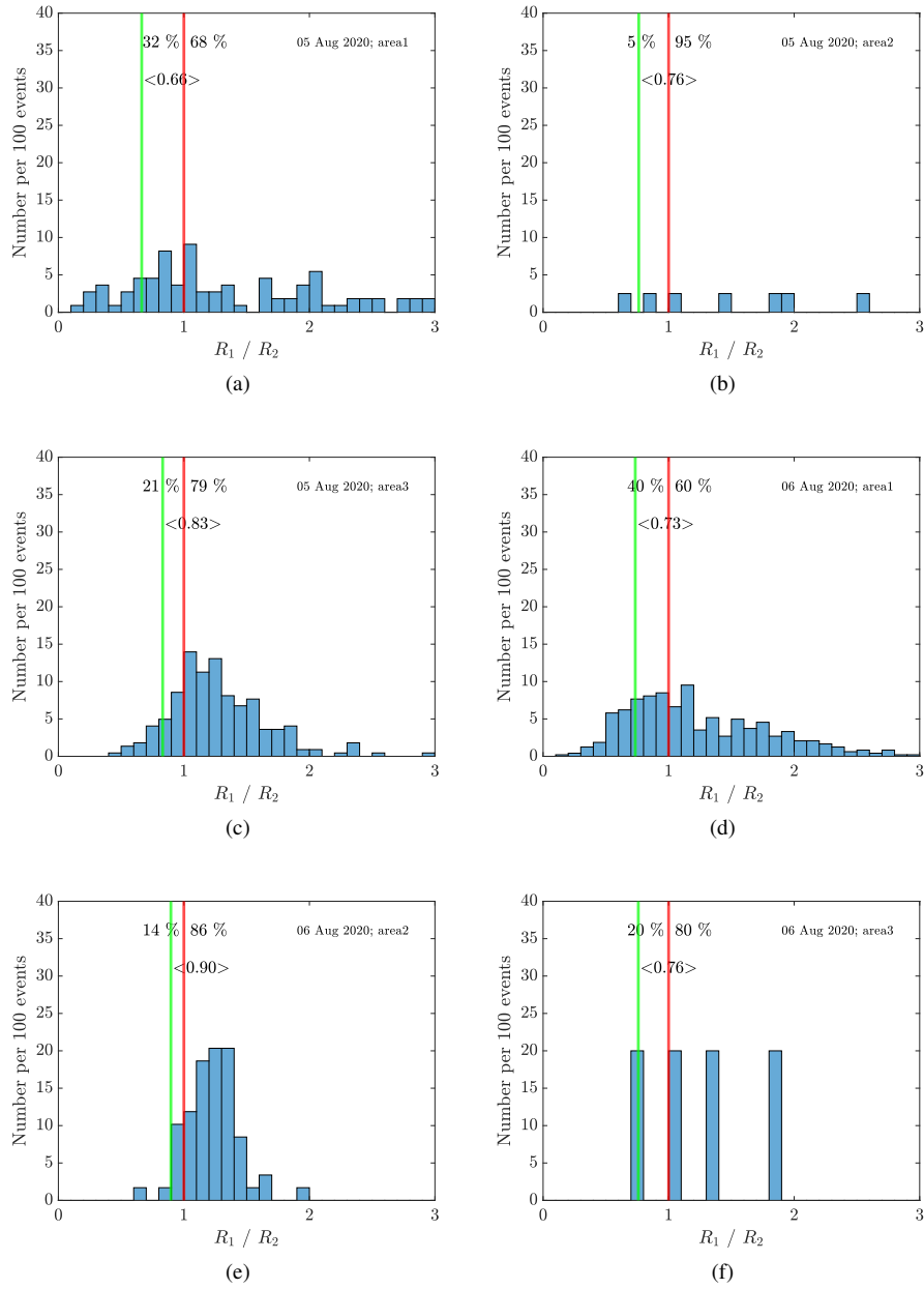
Figure S32. Average of the heating for the observed data on the 5 and 6 August 2020. Only overshoot curves with a minimal background amplitude of R_0 > 10^{10.5} are considered. The ratios are chosen in such a way, that, if we observe an overshoot curve like shown in Fig. ??, all ratios are smaller than 1. Thus, the histograms are clipped at a maximum ratio of 3. The green line and the corresponding number displays the mean for all ratios smaller than 1.
