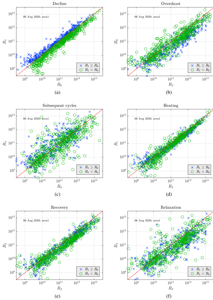
Figure S24. Comparison of the power amplitudes observed on the 6 August 2020 in Area 1.
