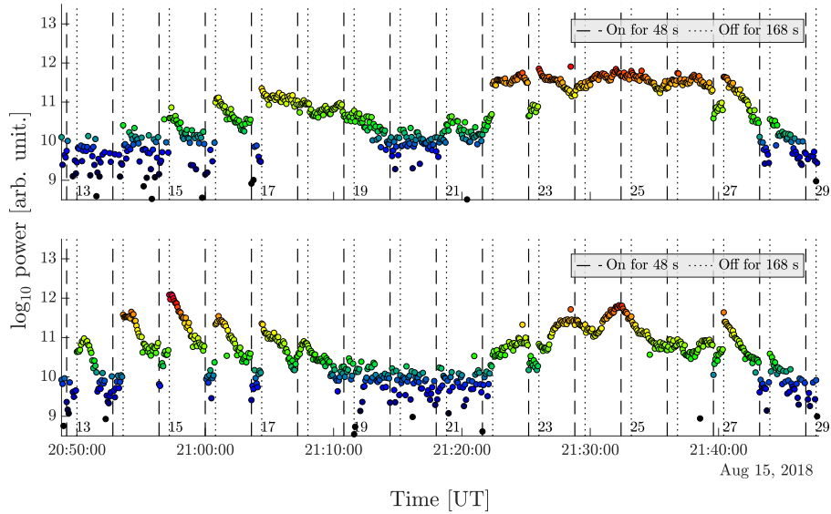
Figure S15. Back scattered power at altitude 87.4 and 87.8 km and heating intervals observed during the night of August 15/16, 2018 in area 2. Each 4.8 seconds there is a data point, usually the interval is 24 seconds. The colour of the dots follow the colour scale of Fig. S5.
