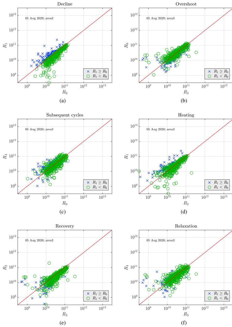
Figure S23. Comparison of the power amplitudes observed on the 5 August 2020 in Area 3.
