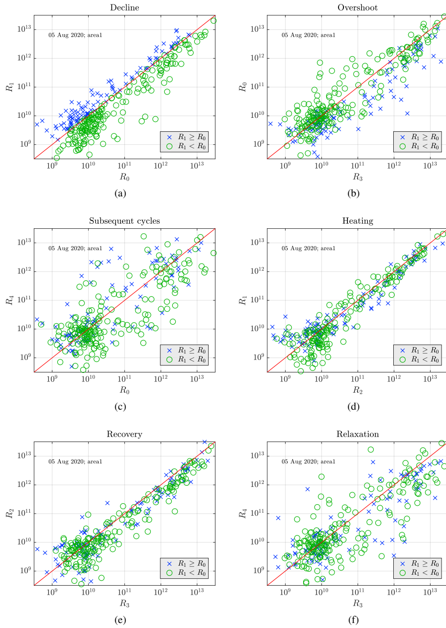
Figure S22. Comparison of the power amplitudes observed on the 5 August 2020 in Area 1.
