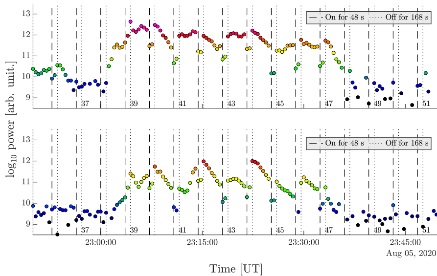
Figure S16. Back scattered power at altitude 85.2 and 85.6 km and heating intervals observed during the night of August 05/06, 2020 in area 2. The colour of the dots follow the colour scale of Fig. S8.
