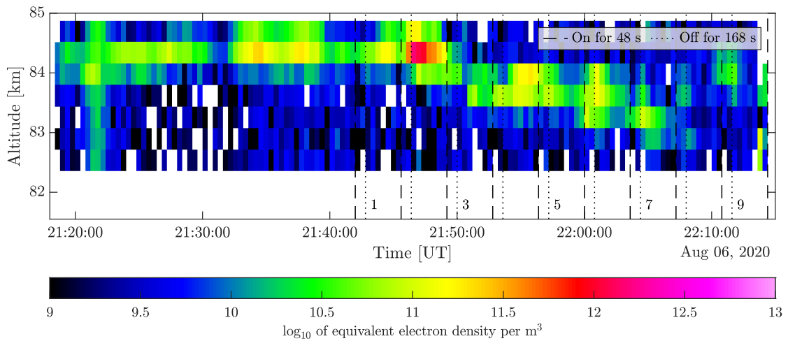
Figure S12. Back scattered power as function of altitude and heating intervals observed during the night of August 06/07, 2020 in Area 3.
