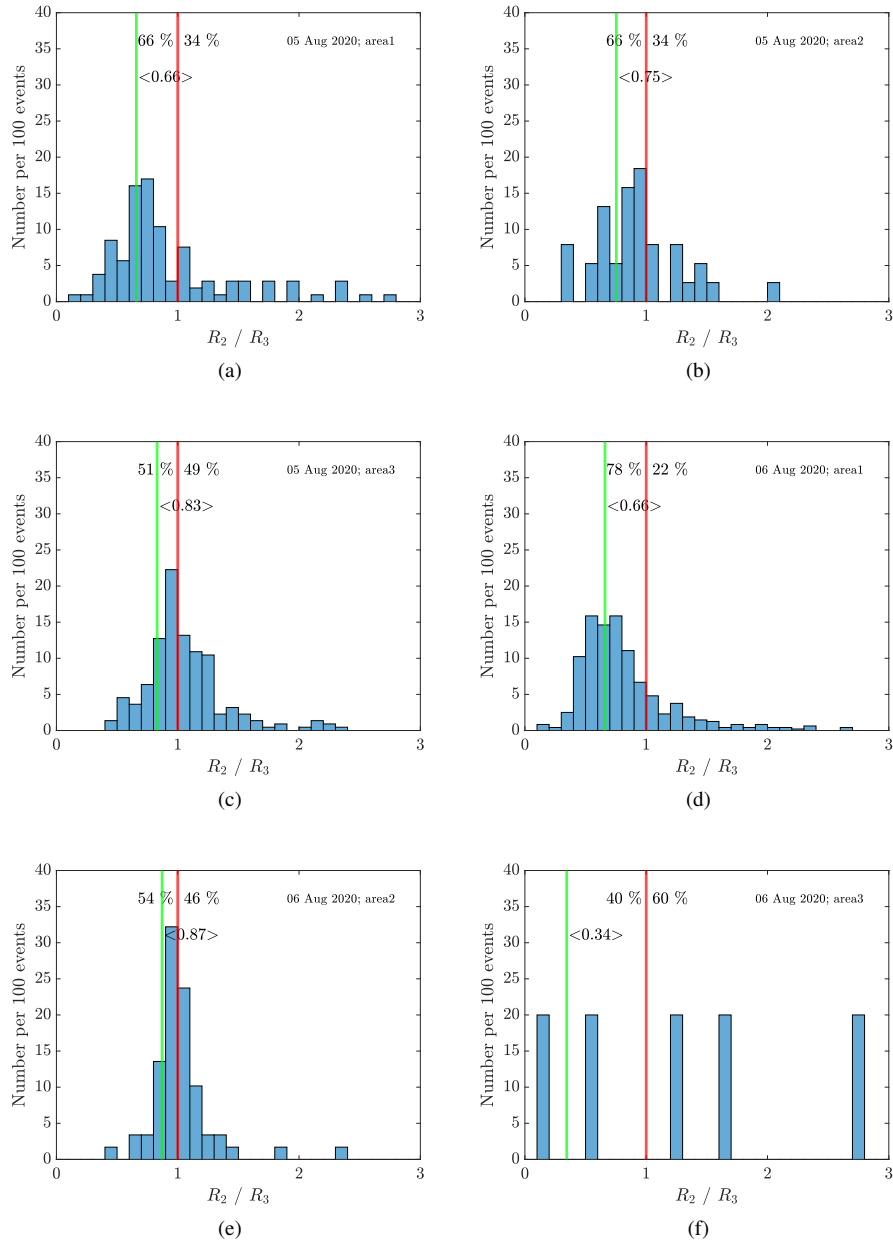
Figure S34. Average of the recovery for the observed data on the 5 and 6 August 2020. Only overshoot curves with a minimal background amplitude of R_0 > 10^{10.5} are considered. The ratios are chosen in such a way, that, if we observe an overshoot curve like shown in Fig. ??, all ratios are smaller than 1. Thus, the histograms are clipped at a maximum ratio of 3. The green line and the corresponding number displays the mean for all ratios smaller than 1.
