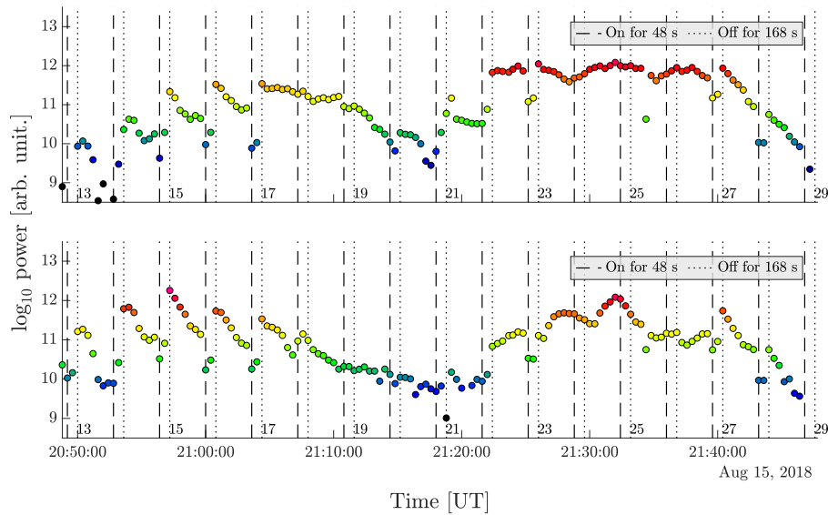
Figure S14. Back scattered power at altitude 87.4 and 87.8 km and heating intervals observed during the night of August 15/16, 2018 in area 2. The colour of the dots follow the colour scale of Fig. S5.
