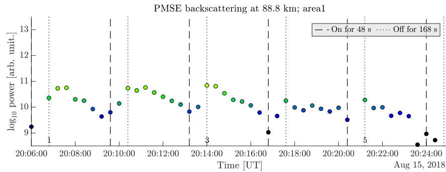
Figure S13. Back scattered power at altitude 88.8 km and heating intervals observed during the night of August 15/16, 2018 in area 1. The colour of the dots follow the colour scale of Fig. S4.
