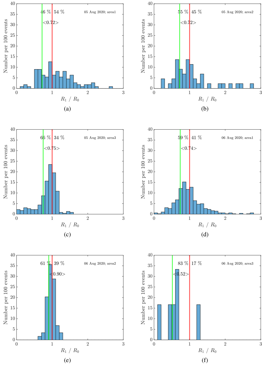
Figure S28. Average of the decline for the observed data on the 5 and 6 August 2020. Only overshoot curves with a minimal background amplitude of R_0 > 10^{10.5} are considered. The ratios are chosen in such a way, that, if we observe an overshoot curve like shown in Fig. ??, all ratios are smaller than 1. Thus, the histograms are clipped at a maximum ratio of 3. The green line and the corresponding number displays the mean for all ratios smaller than 1.
