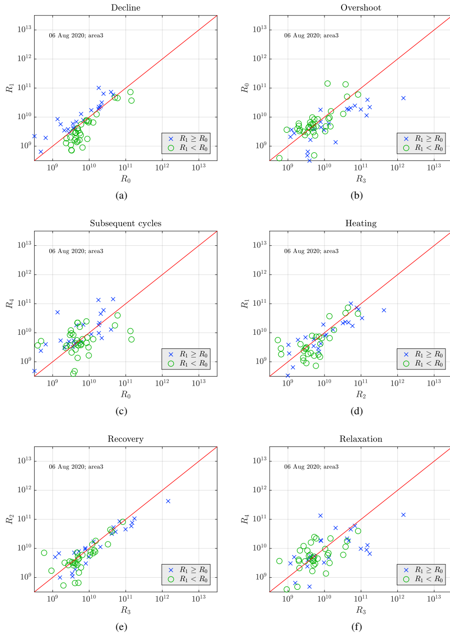
Figure S26. Comparison of the power amplitudes observed on the 6 August 2020 in Area 3.
