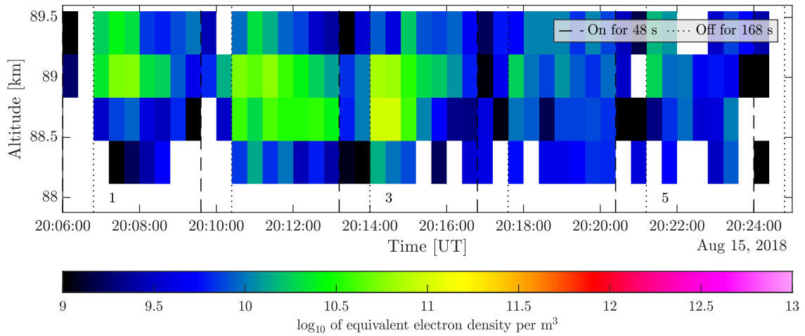
Figure S4. Back scattered power as function of altitude and heating intervals observed during the night of August 15/16, 2018 in Area 1.
