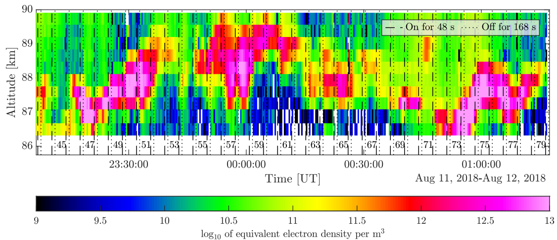
Figure S2. Back scattered power as function of altitude and heating intervals observed during the night of August 11/12, 2018 in Area 2.
