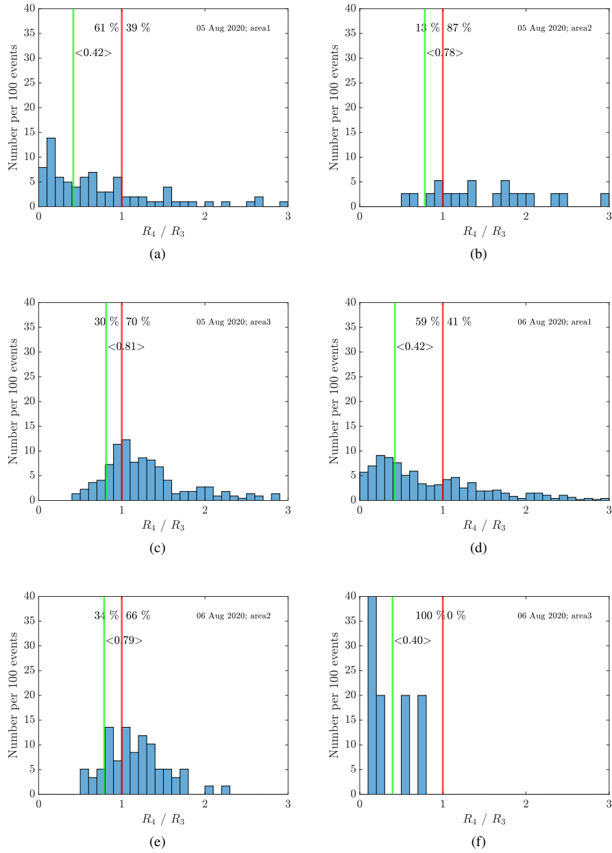
Figure S36. Average of the relaxation for the observed data on the 5 and 6 August 2020. Only overshoot curves with a minimal background amplitude of R_0 > 10^{10.5} are considered. The ratios are chosen in such a way, that, if we observe an overshoot curve like shown in Fig. ??, all ratios are smaller than 1. Thus, the histograms are clipped at a maximum ratio of 3. The green line and the corresponding number displays the mean for all ratios smaller than 1.
