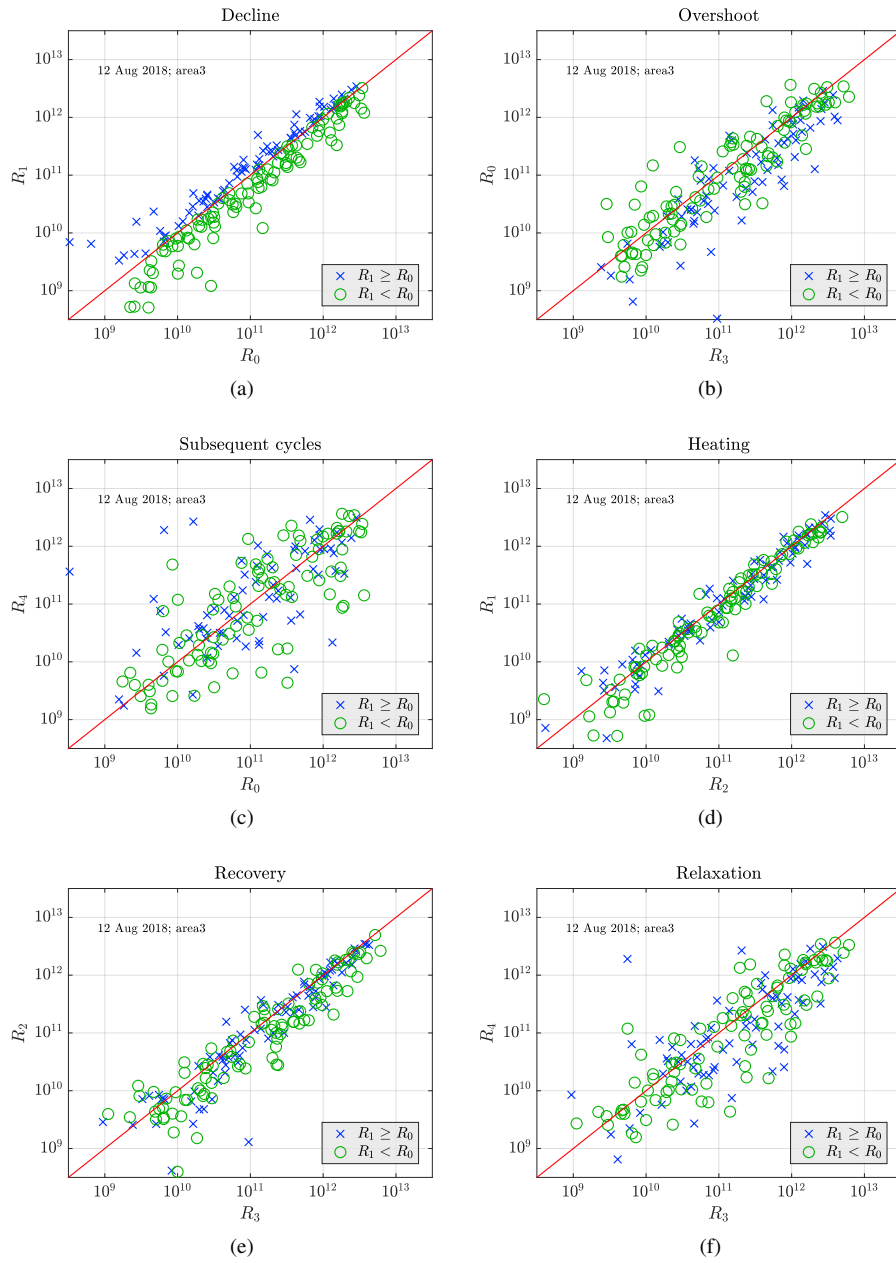
Figure S19. Comparison of the power amplitudes observed on the 11 August 2018 in Area 3.
