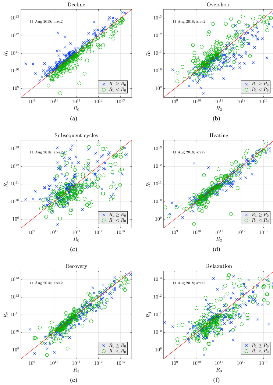
Figure S18. Comparison of the power amplitudes observed on the 11 August 2018 in Area 2.
