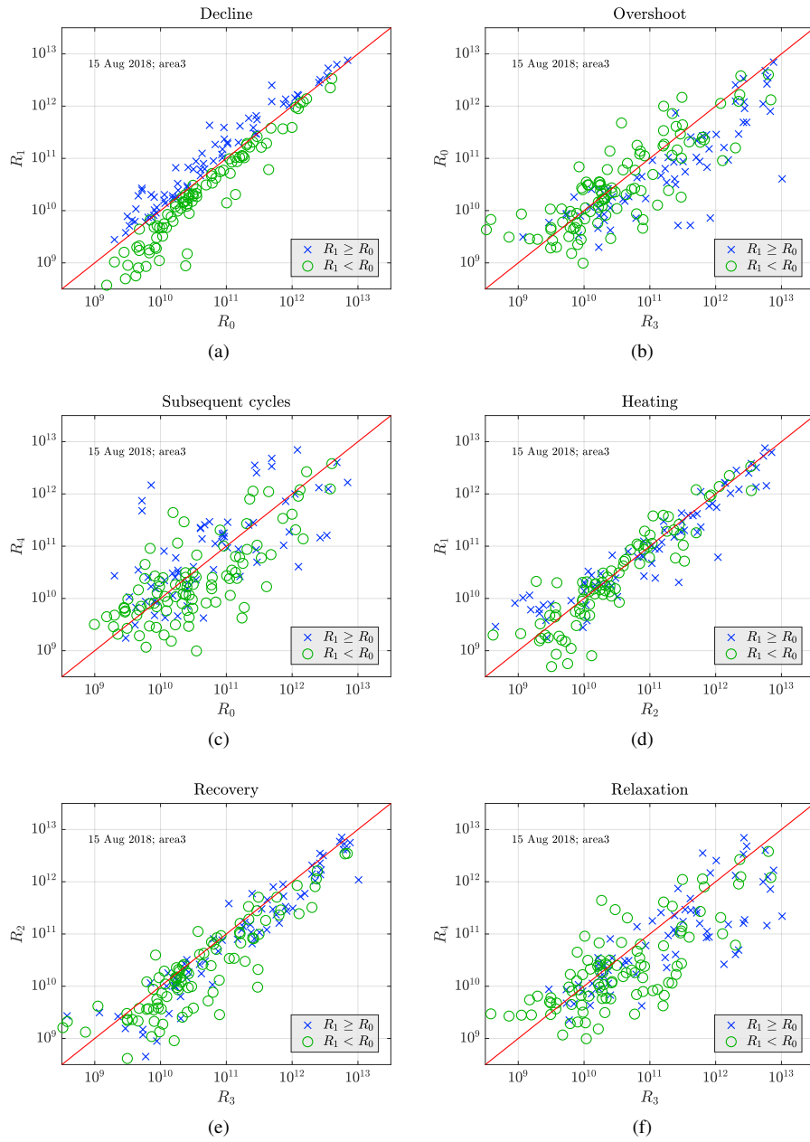
Figure S21. Comparison of the power amplitudes observed on the 15 August 2018 in Area 3.
