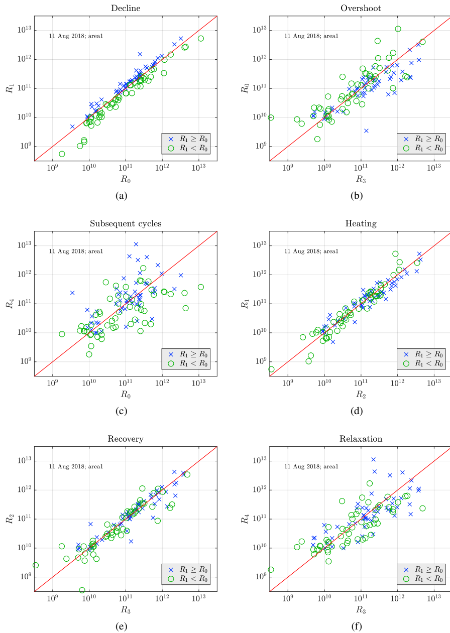
Figure S17. Comparison of the power amplitudes observed on the 11 August 2018 in Area 1.
