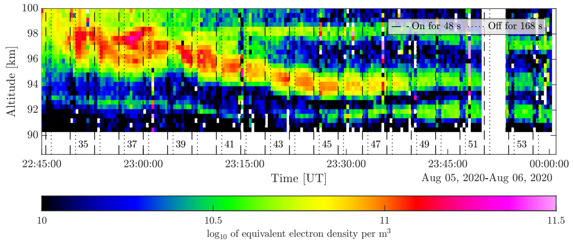
Figure S9. Back scattered power as function of altitude and heating intervals observed during the night of August 05/06, 2020 in Area 3. It should be noted that other limits of the colour scale have been chosen for this plot.
