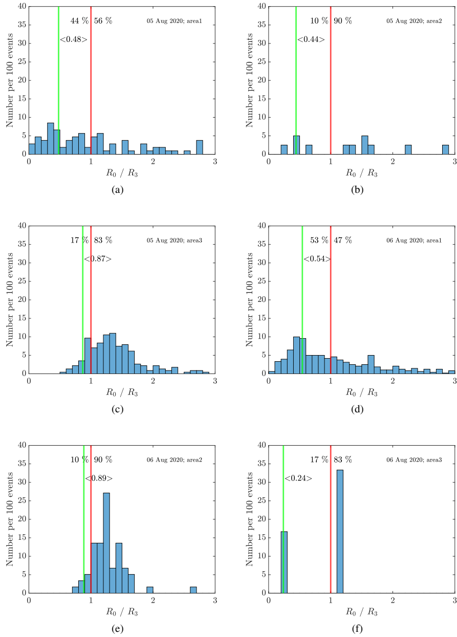
Figure S30. Average of the overshoot for the observed data on the 5 and 6 August 2020. Only overshoot curves with a minimal background amplitude of R_0 > 10^{10.5} are considered. The ratios are chosen in such a way, that, if we observe an overshoot curve like shown in Fig. ??, all ratios are smaller than 1. Thus, the histograms are clipped at a maximum ratio of 3. The green line and the corresponding number displays the mean for all ratios smaller than 1.
