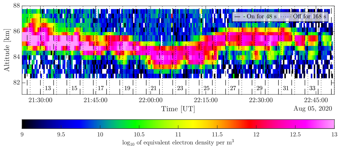
Figure S7. Back scattered power as function of altitude and heating intervals observed during the night of August 05/06, 2020 in Area 1.
