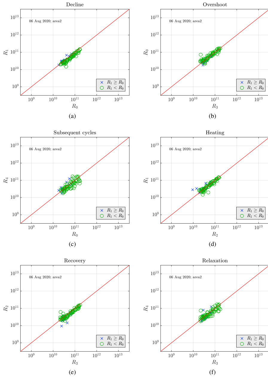
Figure S25. Comparison of the power amplitudes observed on the 6 August 2020 in Area 2.
