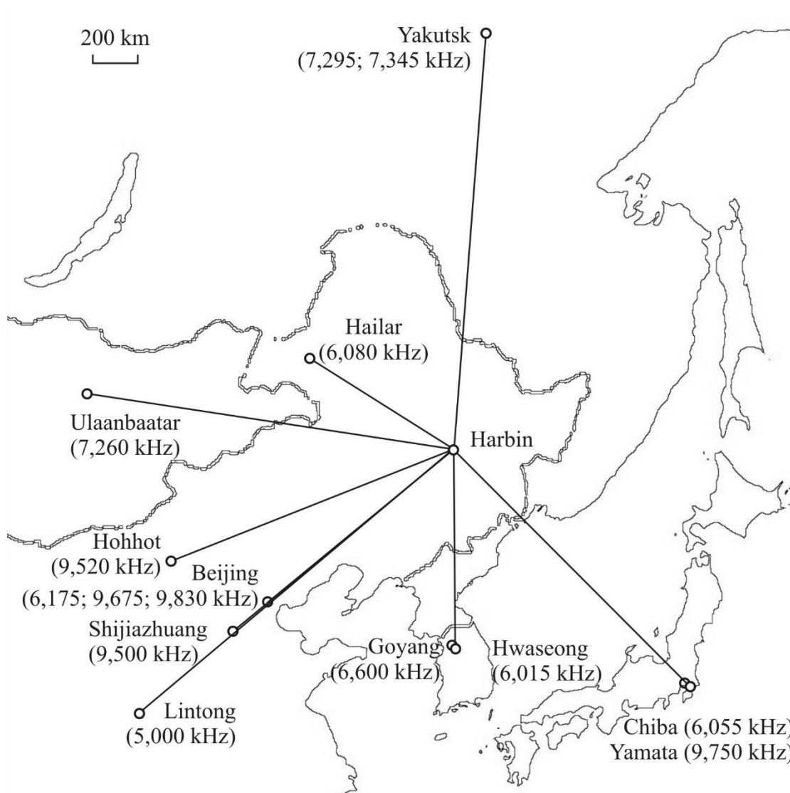
185 Figure 2: Schematic diagram showing the locations of the transmitters and the receiver (Harbin) connected by the great-circle propagation paths, which were used for the observation of solar eclipse effects.
