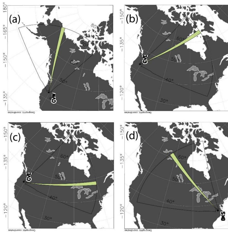
800 Figure 10: Radar FoVs and selected beams of the (a) Christmas Vallee West (CVW) radar beam 12, (b) Christmas Vallee East (CVE) radar beam 5 (c) the CVE radar beam 15, and (d) BKS radar beam 15 used in Fig. 9.
