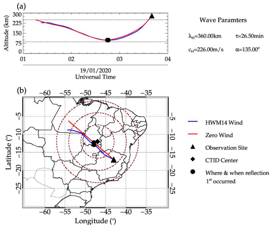
Fig. 7. Backward Ray-Tracing of the MSTID circular waves, starting from 300 km altitude at (17.0°S, 43.0°W) at 03:40 UT.
