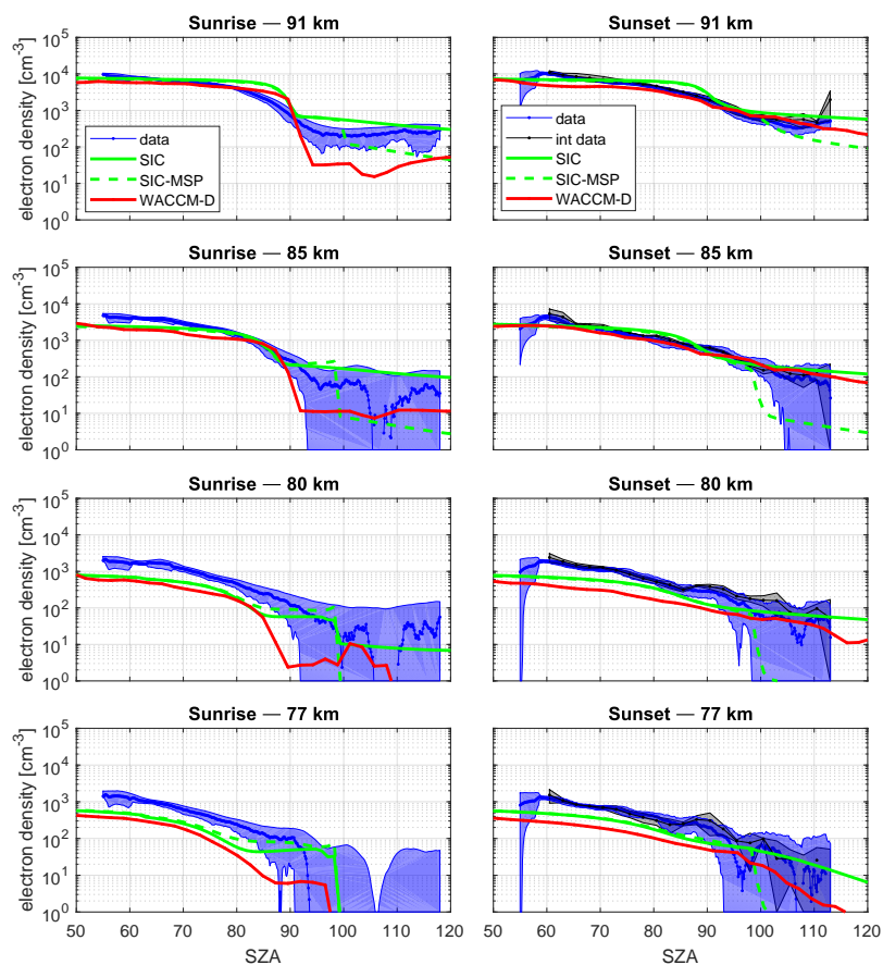
Figure 3. Comparison of measured electron densities with model results from the SIC and WACCM-D model for sunrise (left) and sunset (right) at 91 km, 85 km, 80 and 77 km altitude. The blue line is the 20 point running mean of the measurements and the blue area is the corresponding standard deviation. Green lines indicate SIC model in its standard version (solid) and with meteoric smoke particles incorporated into the ion chemistry (dashed). WACCM-D results are given in red.
