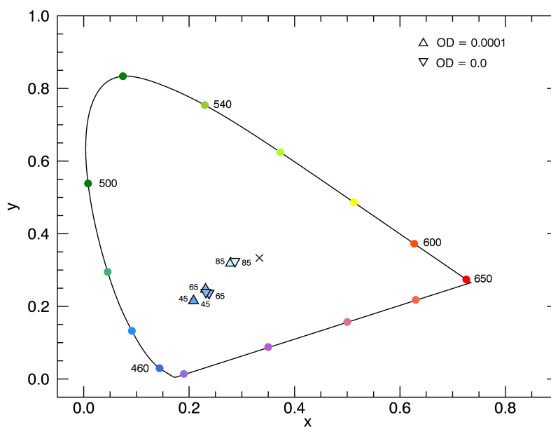
Figure 4. CIE chromaticity diagram corresponding to Fig. 3 with NLCs ( OD = 10^{-4} ) and without NLCs ( OD = 0 ). Marked at the data points: VZAs = 45^\circ , 65^\circ and 85^\circ , with SZA = 98^\circ and SAA = 0^\circ .
