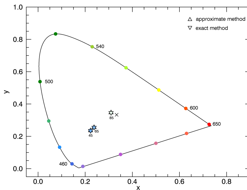
Figure 13. CIE chromaticity diagram for simulations with NLCs considering different methods for treating multiple scattering. Marked at the data points: VZAs = 45°, 65° and 85°, with SZA = 98° and SAA = 0°. The NLC parameters are: r_m = 50 nm, S = 1.4 , \tau_{\text{NLC}} = 10^{-4} and z_{\text{NLC}} = 82 km.
