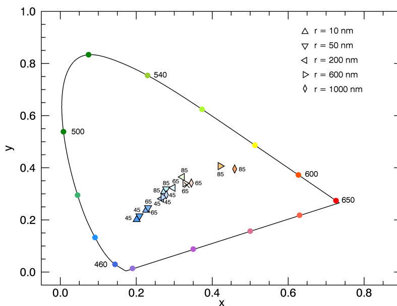
Figure 8. CIE chromaticity diagram for simulations with NLCs and different median radii of the NLC particle size distribution. Marked at the data points: VZAs = 45°, 65° and 85°, with SZA = 98° and SAA = 0°. The width parameter of the size distribution is S = 1.4 and the optical depth is \tau_{\text{NLC}} = 10^{-4} .
