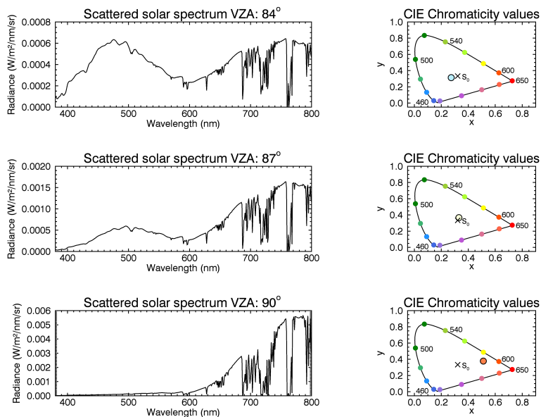
Figure 10. Solar scattering spectra (left column) and CIE chromaticity diagram (right column) for an observer on the Earth’s surface and for SA = 98^\circ , VZA = 84^\circ, 87^\circ, 90^\circ (from top to bottom) and SAA = 0^\circ . The simulations are calculated for NLCs with following parameters: r_m = 50 nm, S = 1.4 , \tau_{NLC} = 10^{-4} and z_{NLC} = 82 km.
