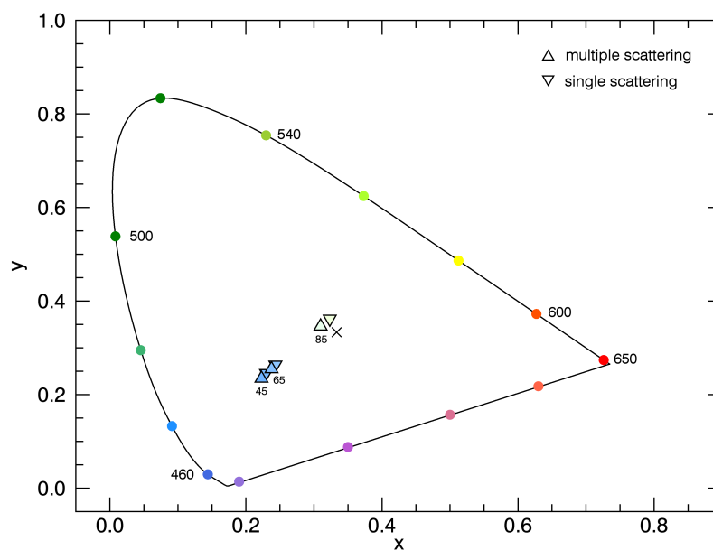
Figure 14. CIE chromaticity diagram for simulations with NLCs considering multiple scattering and single scattering only. Marked at the data points: VZAs = 45^\circ , 65^\circ and 85^\circ , with SZA = 98^\circ and SAA = 0^\circ . The NLC parameters are: r_m = 50 nm, S = 1.4 , \tau_{\text{NLC}} = 10^{-4} and z_{\text{NLC}} = 82 km.
