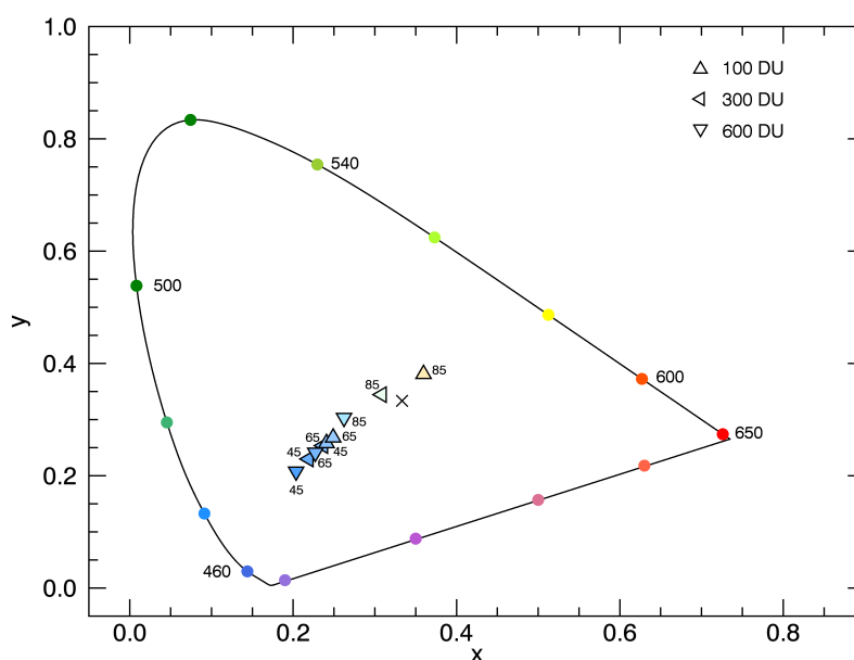
Figure 7. CIE chromaticity diagram for spectra including NLCs and different ozone column densities. Marked at the data points: VZAs = 45°, 65° and 85°, with SZA = 98° and SAA = 0°. The NLC parameters are as for the left panel of Fig. 3, i.e.: r_m = 50 nm, S = 1.4 , \tau_{\text{NLC}} = 10^{-4} and z_{\text{NLC}} = 82 km.
