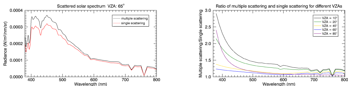
Figure 15. Solar scattering spectra for VZA = 65^\circ with the multiple scattering (black line) and without the multiple scattering contribution to the total scattered radiance (red line). Right panel: Ratio of multiple scattering and single scattering for different VZAs. For all simulations, SAZ = 98^\circ and SA = 0^\circ . The NLC parameters are: r_m = 50 nm, S = 1.4 , \tau_{NLC} = 10^{-4} and z_{NLC} = 82 km.
