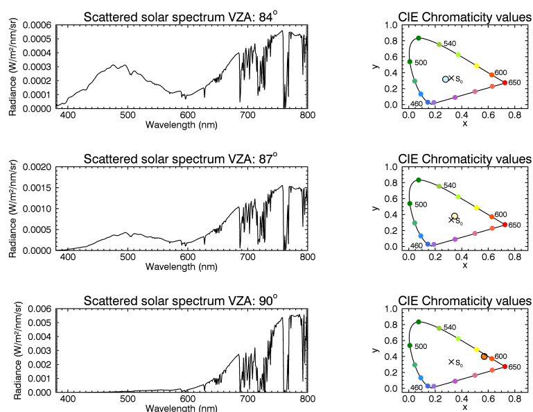
Figure 11. Solar scattering spectra (left column) and CIE chromaticity diagram (right column) for an observer on the Earth’s surface and for SA = 98^\circ , VZA = 84^\circ, 87^\circ, 90^\circ (from top to bottom) and SAA = 0^\circ . The calculated spectra show the background without NLCs.
