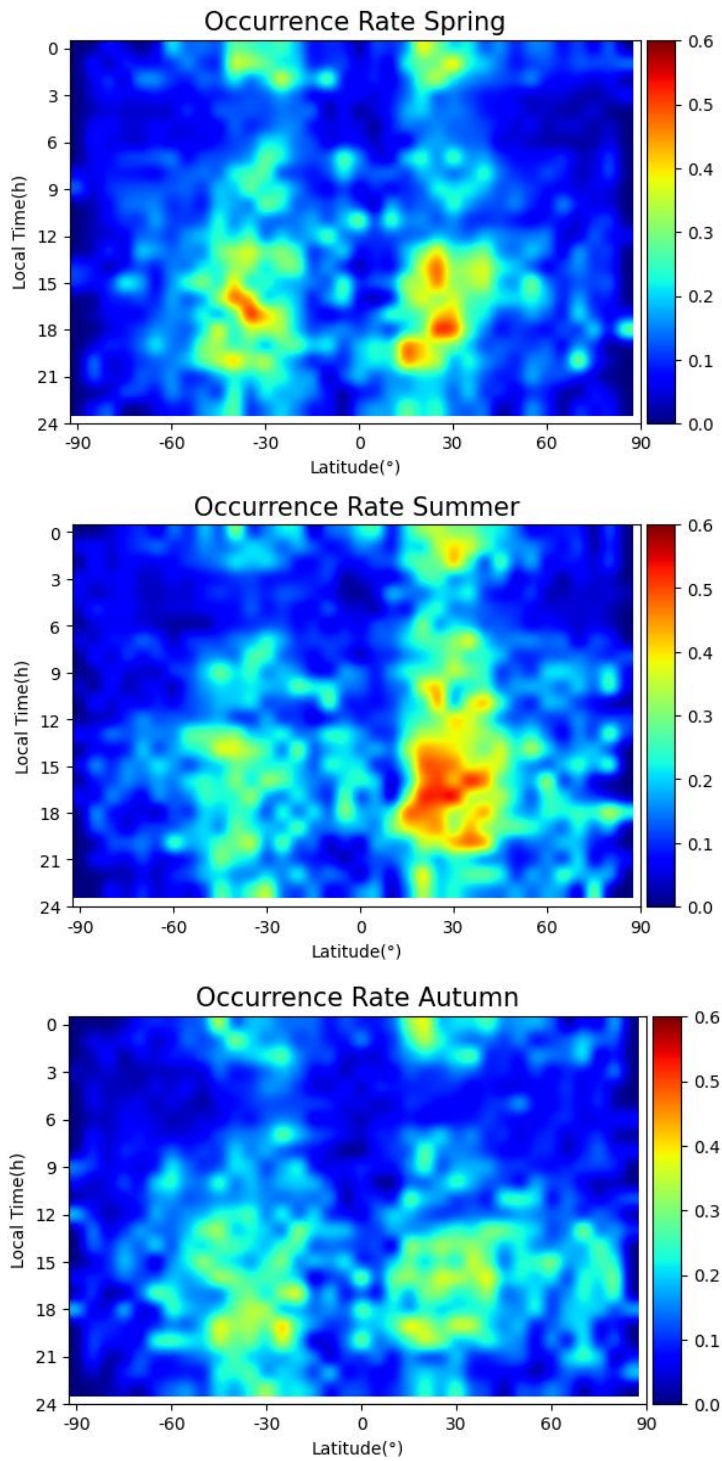
Figure 6 The distribution of Es occurrence rate for three different seasons in 1\text{h}\times 5^\circ local time/geographic latitude grid, from top to bottom are the results of spring, summer and autumn, respectively.
