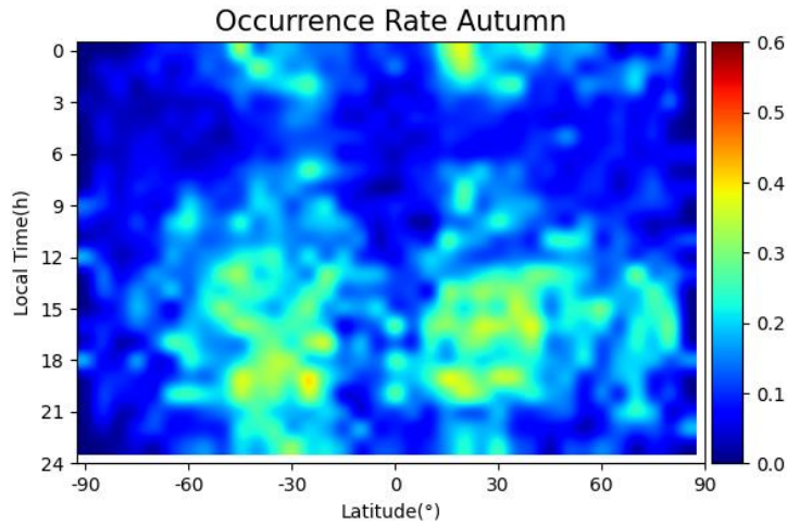
Figure 6 The distribution of Es occurrence rate for three different seasons in 1h×5° local time/geographic latitude grid, from top to bottom are the results with of spring, summer and autumn, respectively.
