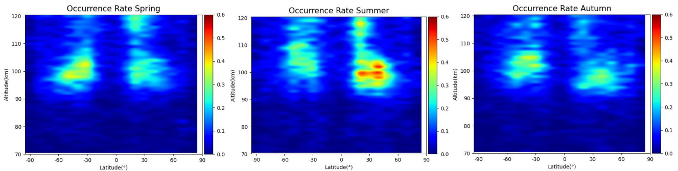
Figure 5 The distribution of Es occurrence rate for three different seasons in 10^{\circ} \times 1\text{km} geographic latitude/altitude grid, from left to right are the results with of spring, summer and autumn, respectively.
