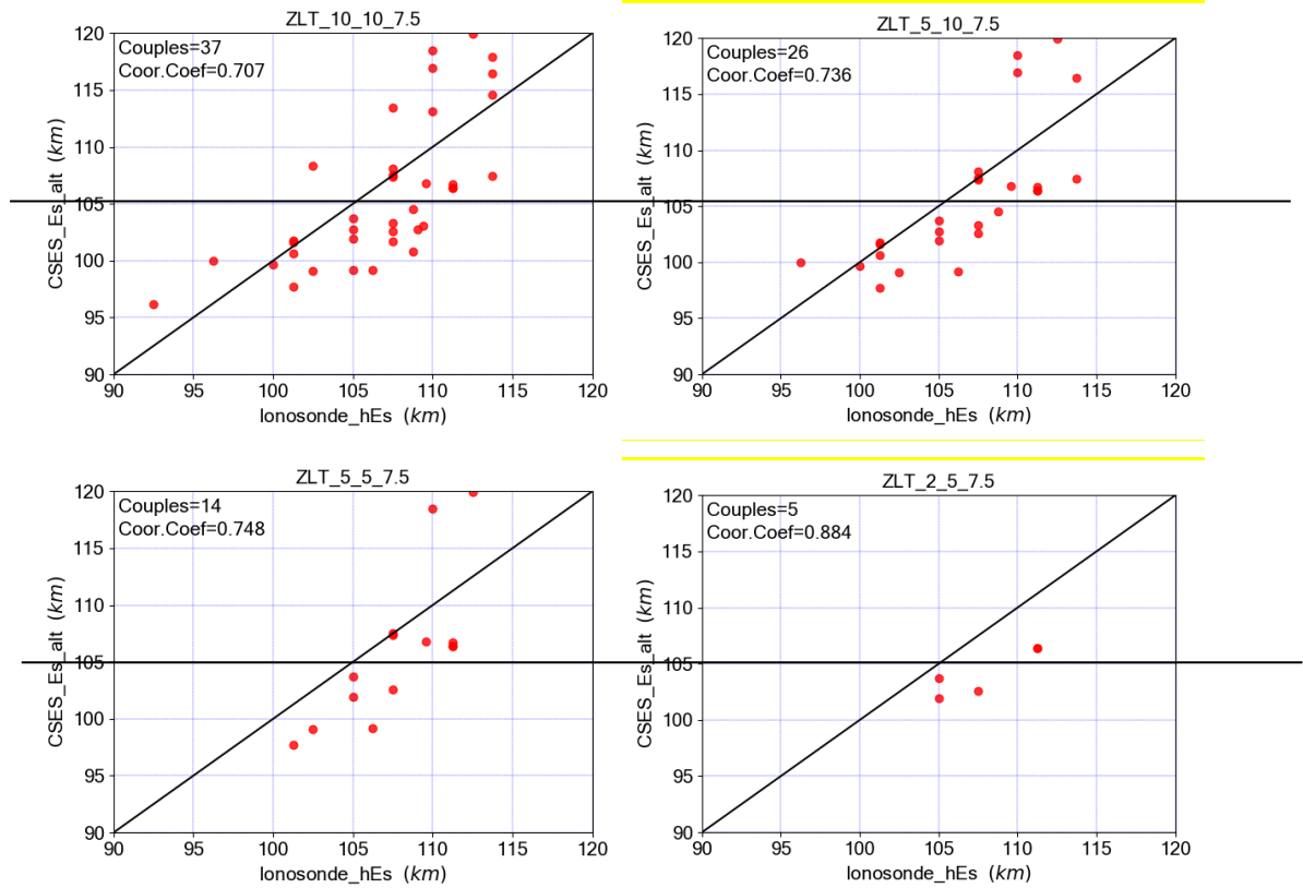
Figure 8 Comparison of the geometric altitudes of Es detected in CSES radio occultation profiles and the virtual heights of Es obtained by the ZLT ionosonde. From top to bottom and from left to right are the results with space-time matching window (10°, 10°, 7.5 min), (5°, 10°, 7.5min), (5°, 5°, 7.5min) and (2°, 5°, 7.5min), respectively.
