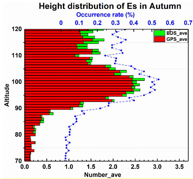
Figure 3 Height distribution of Es average daily occurrence rate for three different seasons, from top to bottom are the results of spring, summer and autumn, respectively. The blue dotted line diagram shows Es occurrence rate, the red and green bar chart shows the number of occultation events with Es events per day.
