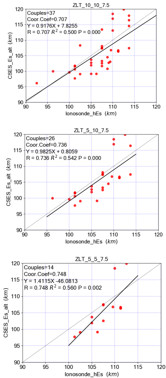
380 Figure 8 Comparison of the geometric altitudes of Es detected in CSES radio occultation profiles and the virtual heights of Es obtained by the ZLT ionosonde. From top to bottom are the results of space-time matching window (10°, 10°, 7.5 min), (5°, 10°, 7.5min) and (5°, 5°, 7.5min), respectively. The black solid line is the regression line.
