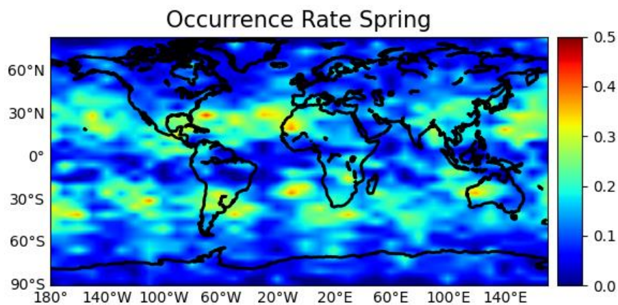
Figure 4 The geographical distribution of Es occurrence rate for three different seasons in 5^{\circ} \times 5^{\circ} geographic latitude/longitude grid, from top to bottom are the results of spring, summer and autumn, respectively.
