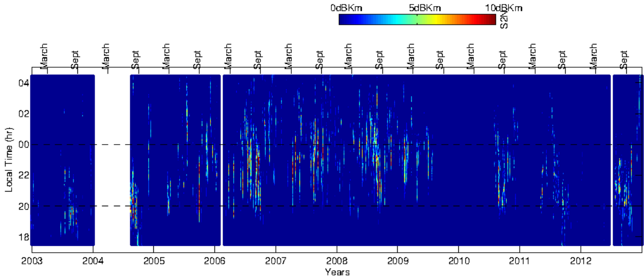
425 Figure 2: VHF radar data is presented as altitude integration from 200 km to 1000 km height as function of signal to noise ratio (dBKm), the horizontal lines represent local sunset and local midnight to help observation of echoes distribution.
