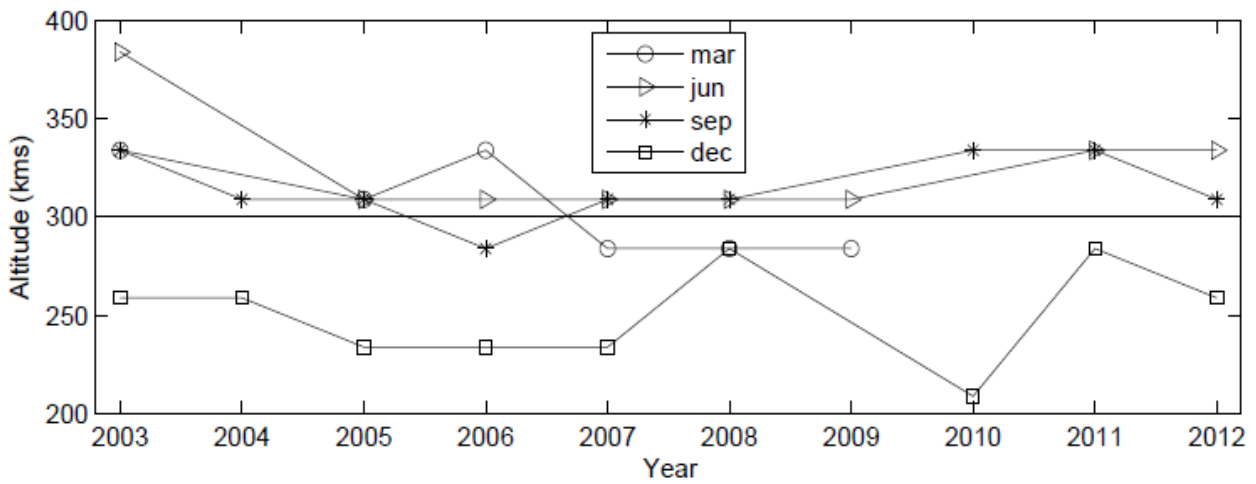
Figure 4: Top Panel: Peak time echoes occurrences along solar cycle and divided by seasons. Bottom panel: Peak altitude echoes occurrences along solar cycle and divided by seasons.
