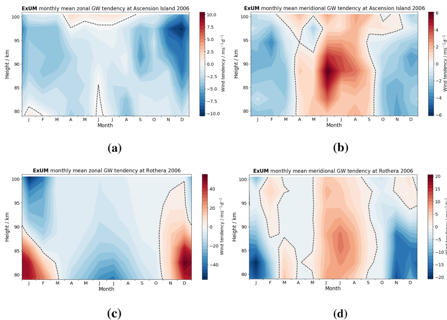
Figure 16. ExUM time-height gravity wave tendency contours in 2006. At Ascension Island for the (a) zonal and (b) meridional components. Similarly at Rothera for the (c) zonal and (d) meridional components.
