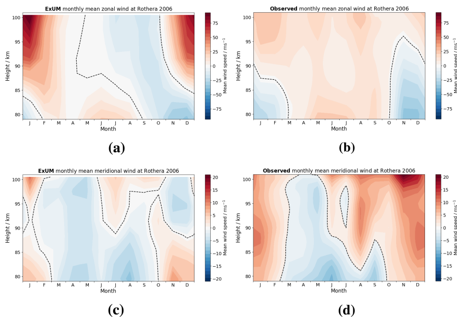
Figure 7. Time-height monthly mean wind contours at Rothera in 2006 comparing (a) ExUM zonal wind with (b) observed zonal wind and (c) ExUM meridional wind with (d) observed meridional wind. The dashed black line represents the zero-wind line. Colour bars are kept consistent left to right for comparison.
