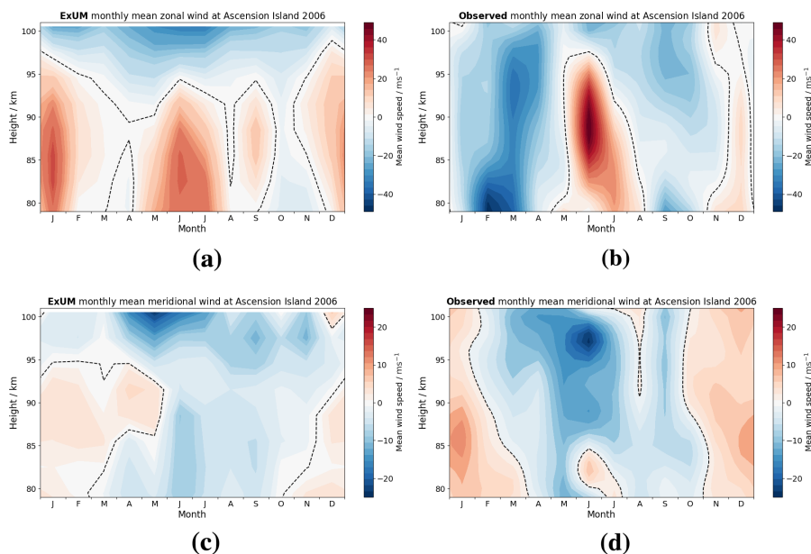
Figure 6. Time-height monthly mean wind contours at Ascension Island in 2006 comparing (a) ExUM zonal wind with (b) observed zonal wind and (c) ExUM meridional wind with (d) observed meridional wind. The dashed black line represents the zero-wind line. Colour bars are kept consistent left to right for comparison.
