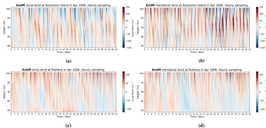
Figure 5. ExUM time-height wind contours from the 94-level model configuration in April 2006. At Ascension Island for the (a) zonal ( u ) and (b) meridional ( v ) components. Similarly at Rothera for the (c) zonal ( u ) and (d) meridional ( v ) components.
