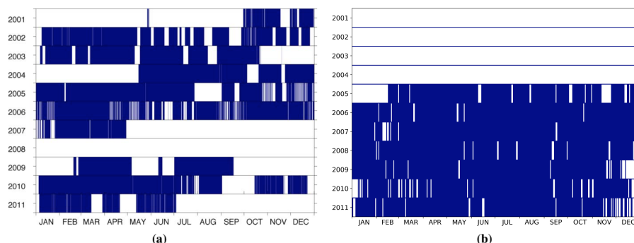
Figure 4. Availability of meteor radar observations for (a) Ascension Island (from Davis et al., 2013) and (b) Rothera. This motivates the choice of 2006 as the year for comparison.
