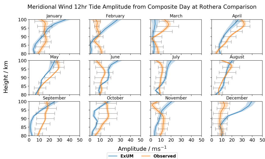
Figure 13. Amplitudes of the (a) zonal ( u ) and (b) meridional ( v ) semi-diurnal tides at Rothera as a function of time and height. The shaded regions denote the standard deviation from the curve fitting algorithm, and the black bars indicate the standard deviation from the mean of the measured amplitudes across the month. Both the amplitudes from the model (blue) and meteor radar (orange) are plotted.
