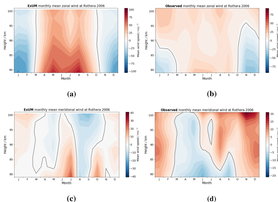
Figure 17. Time-height monthly mean wind contours at Rothera in 2006 comparing (a) ExUM zonal wind without the USSP with (b) observed zonal wind and (c) ExUM meridional wind without the USSP with (d) observed meridional wind. The dashed black line represents the zero-wind line. Colour bars are kept consistent left to right for comparison.
