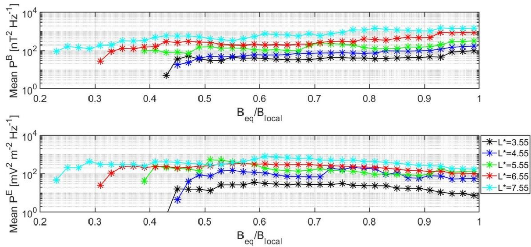
Figure 1: Logarithms of the mean ULF power with 1-min as a function of B_{eq}/B_{local} ( dB=0.05 ) for 5 L^* bins with dL^*=0.1 .
