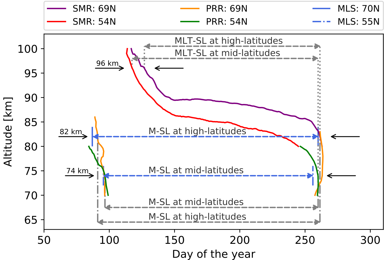
Figure 2. Mean zonal wind reversal comparison and summer length definitions (MLT-SL and M-SL) at high- and mid-latitudes. The mean zonal wind reversal (0 m/s) extracted from the climatologies from: SMRs (purple) and PRR (orange) at 69 N, SMRs (red) and PRR (green) at 54 N. In addition, the specific geopotential heights with the zero zonal mean geostrophic zonal winds values from MLS (blue) are shown at 70 N (solid line) and at 55 N (dash-dotted line). The black arrows indicate the altitude taken for the mean zonal wind reversal used in the individual definitions.
