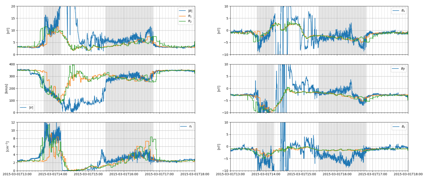
Figure 2. A comparison of MAVEN observations (blue) with two O^+ model runs ( R_1 in orange and R_2 in green) at 490 s. In the left column, from the top, we have magnetic field magnitude, proton velocity, and proton number density. In the right column we have the three magnetic field components ( B_x , B_y , and B_z ) in MSO coordinates. Indicated in gray is also the location of the magnetosheath as seen from the observations. The induced magnetosphere is thus between the two gray regions.
