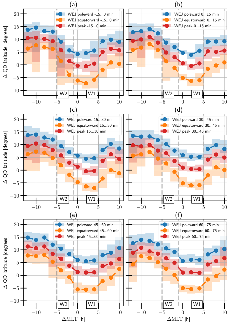
Figure 7. The evolution of the WEJ maxima-peak location and extent for the time period of 15 minutes before to 75 minutes after the onset. \Delta QD is the latitude relative to the onset latitude. The lines show the median and the shadings show the range covered by the second and third quartiles.
