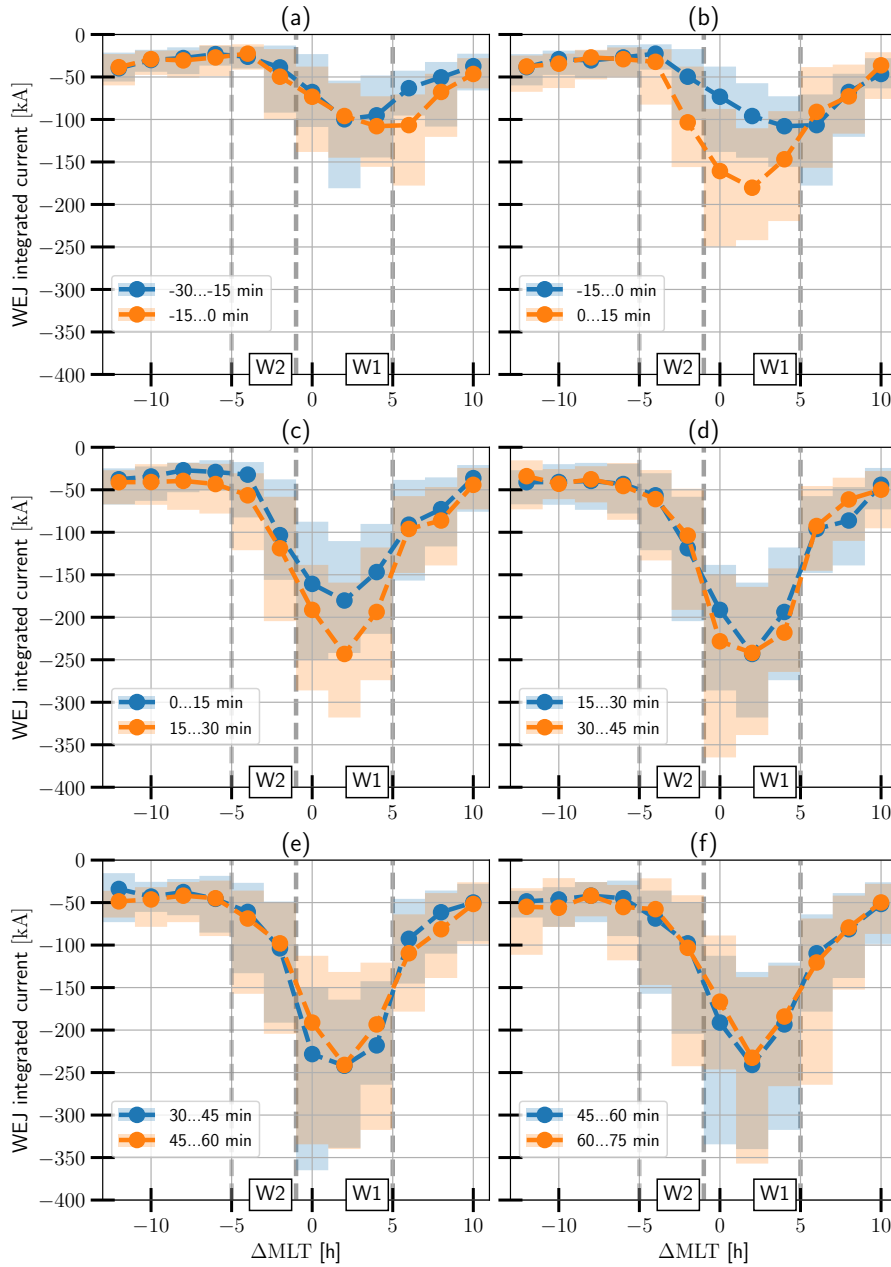
Figure 5. The evolution of the westward electrojet-WEJ compared to the previous time step for the time period of 30 minutes before to 75 minutes after the onset. The lines show the medians and 50 % of the values are contained within the bars in each bin.
