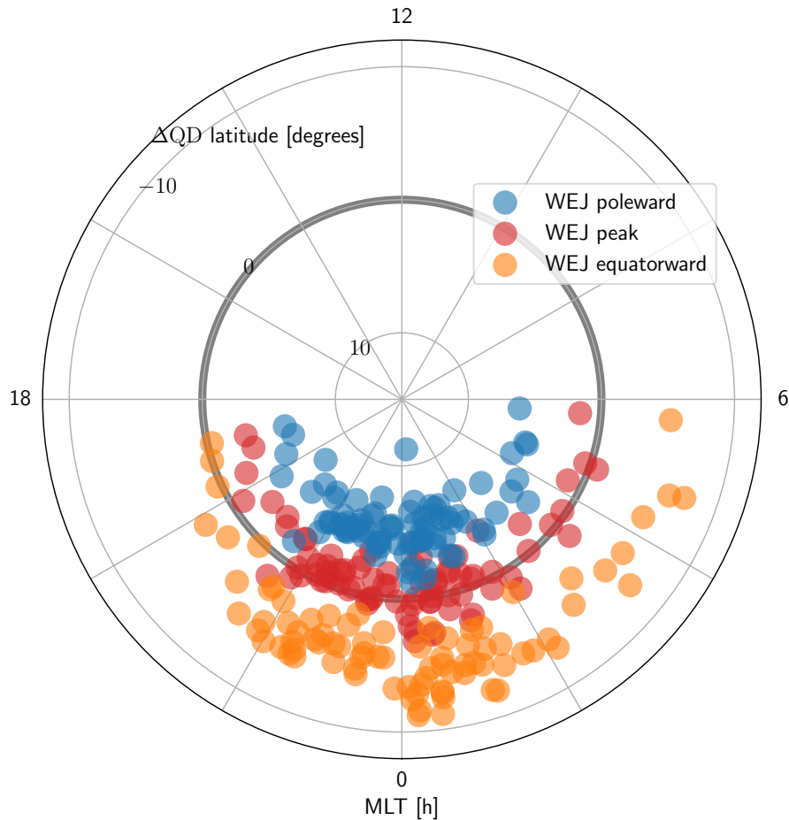
Figure 10. The MLT and \Delta QD latitude locations of the WEJ peaks and northern-southern poleward and equatorward borders in the 2 hour MLT bin centered around the onset location 0...15 0 to 15 minutes after the onset. \Delta QD is the latitude relative to the onset latitude.
