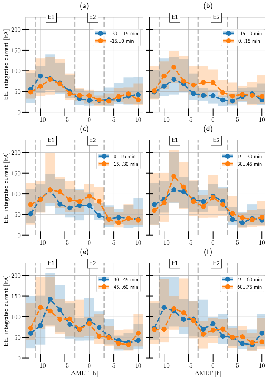
Figure 6. The evolution of the eastward electrojet-EEJ compared to the previous time step for the time period of 30 minutes before to 75 minutes after the onset. The lines show the medians and 50 % of the values are contained within the bars in each bin.
