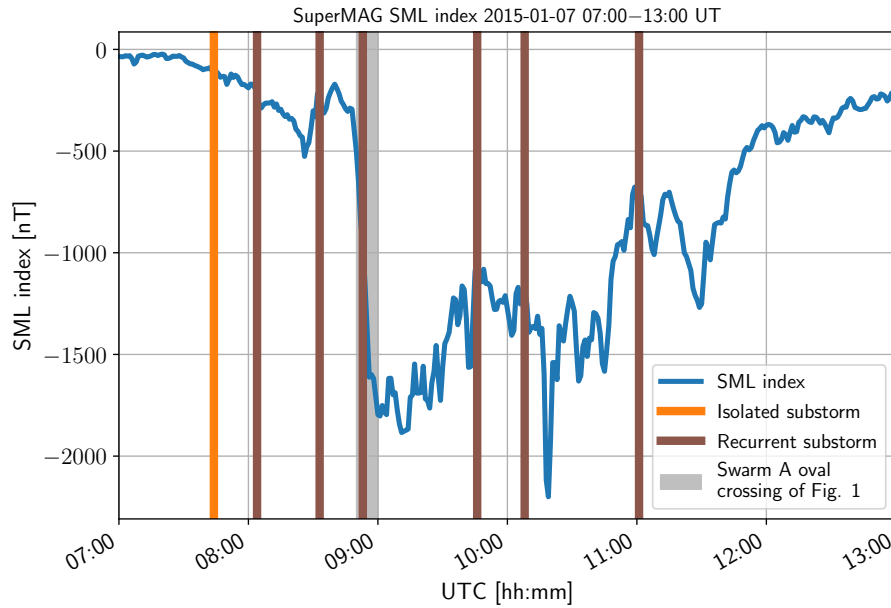
Figure 2. An example timeseries of the SuperMAG-SML index with the isolated and recurrent substorm onsets marked with vertical lines. The grey shading shows the relation of the oval crossing of Fig. 1 to the SML timeseries.
