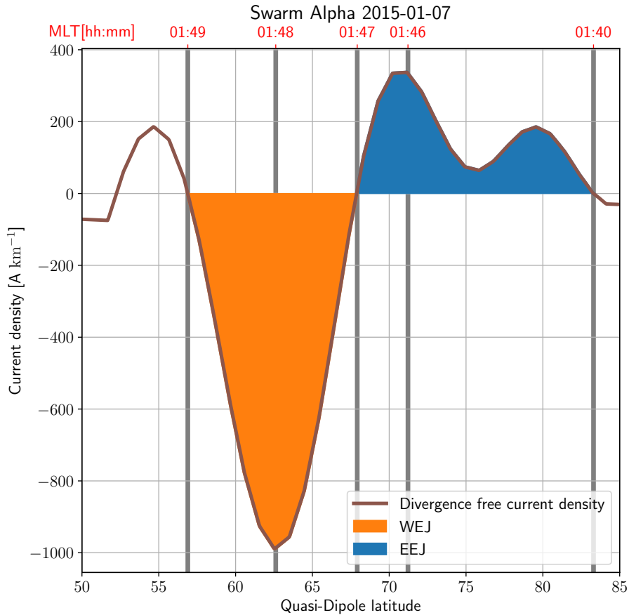
Figure 1. An example of the divergence free current derived from Swarm Alpha data with the 1-D SECS method and the identified electrojets from the AEBS-Swarm-AEBS data set. The location of the boundaries and maxima have been marked with vertical lines. The colored sections show the area corresponding to the integrated currents.
