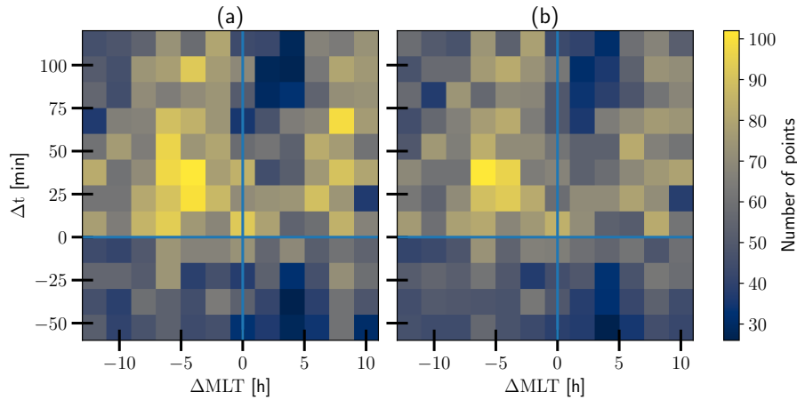
Figure 3. The number of Swarm oval crossings in each bin for westward-electrojets-WEJ (a) (corresponding to panel-panels (a) and (c) in Fig. 4) and eastward-electrojets-EEJ (b) (corresponding to panel-panels (ab) and (d) in Fig. 4). \Delta\text{MLT} is the magnetic local time distance to the onset and \Delta t is the temporal distance to the onset.
