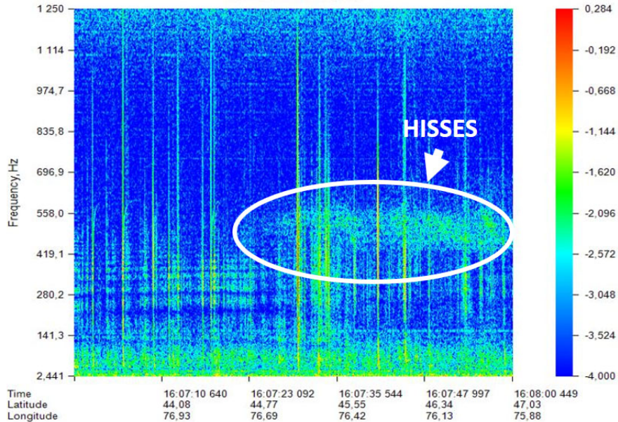
Figure 9. Graph and spectrum of electric field strength in the ELF band for the ascending half-orbit No.29720.
