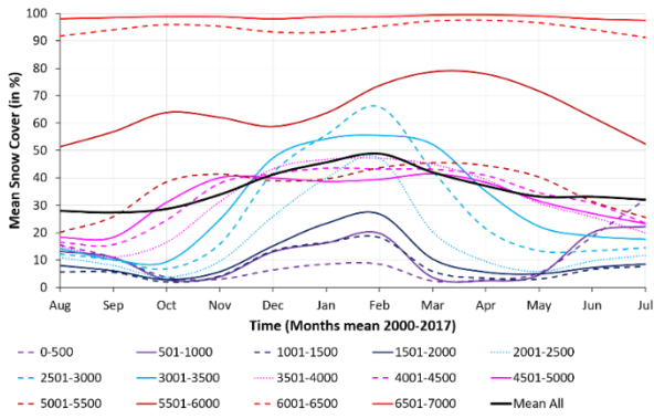
495 Fig. 4. (a) The mean snow cover hypsographic curves during 2000 to 2017 over HKH region: (a) seasonal curves for accumulating season (red line), melting season (blue line) and all season (black line), (b) monthly composites (in percent) during the snow melting and accumulating seasons. (c) The variability of mean snow cover over months (at different altitudes, <5500m) show starting of decline in snow-cover from the month of March onwards (black line is average).
