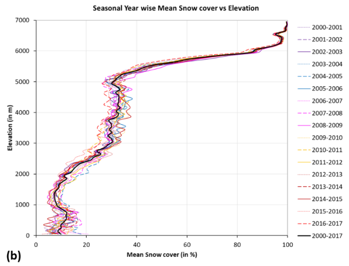
Fig. 3. The hypsographic curves of (a) year-wise mean snow cover (in percent) for 2000-2016 and (b) Seasonal year-wise (March to Feb) snow cover (in percent) for 2000-2017, respectively, over HKH region. Note, the seasonal average of snow cover for year 2016 is lower because of missing data for the months of January and February.
