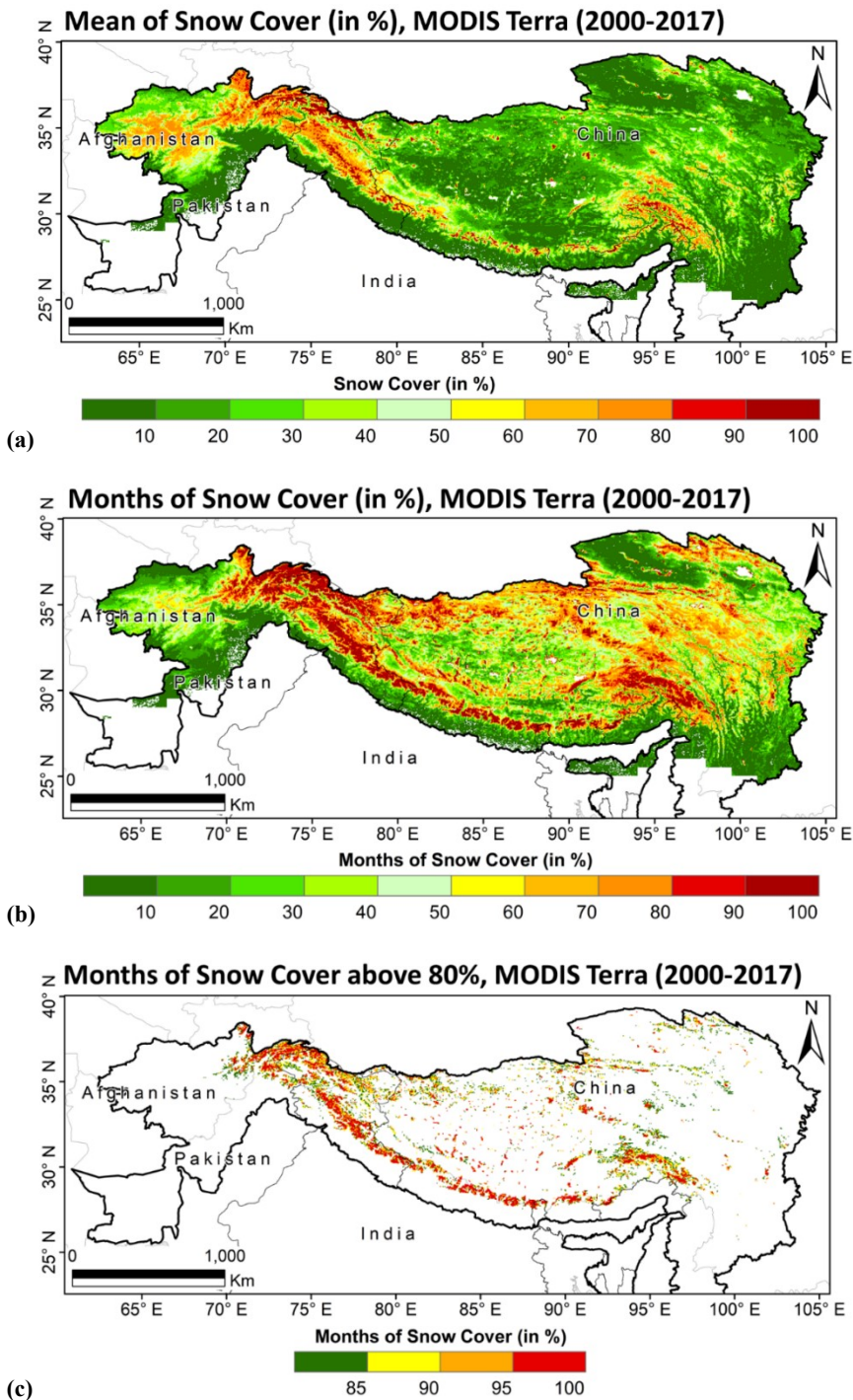
465 Fig. 1. The spatial distribution of MODIS Terra derived (a) monthly mean snow cover (in percent), (b) the total duration of the presence of snow cover (in percent) out of 204 months, and (c) the presence of snow cover above 80% (total months out of 204 months) during March 2000 to February 2017 over the HKH region
