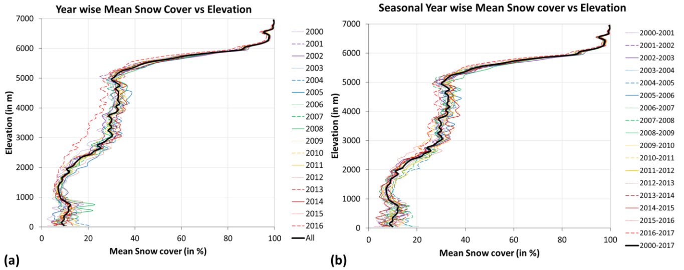
475 Fig. 3. The hypsographic curves of (a) year-wise mean snow cover (in percent) for 2000-2016 and (b) Seasonal year-wise (March to Feb) snow cover (in percent) for 2000-2017, respectively, over HKH region. Note, the seasonal average of snow cover for year 2016 is lower because of missing data for the months of January and February.
