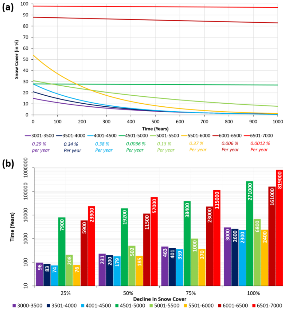
510 Fig. 7. The results from linear trend analysis of Snow Cover change (mainly reduction) during 2000-2017, and in subsequent years, over the HKH region and where the trend was found to be statistically significant (95% CI).
