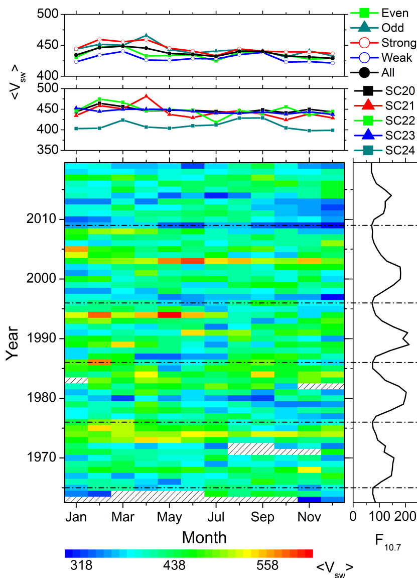
Figure 10. Solar wind speed V_{sw} ( \text{km s}^{-1} ) variation from 1963 through 2019. The panels are in the same format as in Figure 7.
