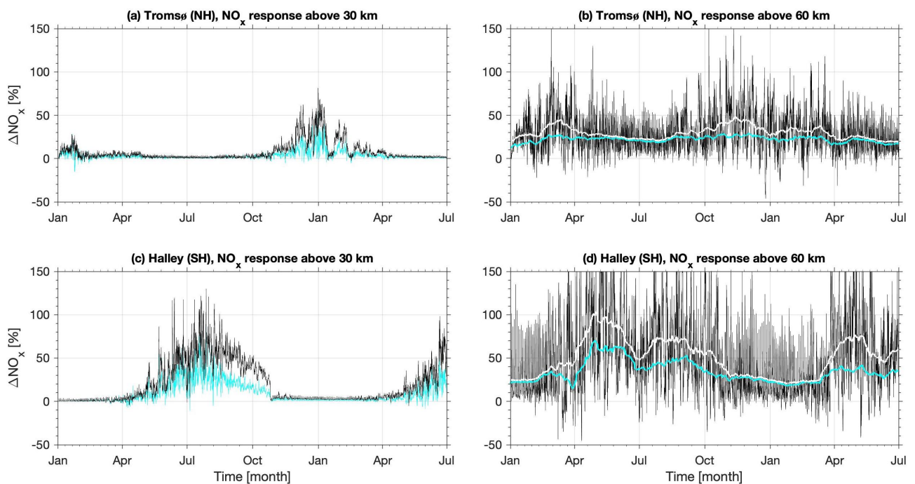
Figure 5. Height-integrated NO x response to PsA-EEP at the Tromsø and Halley stations. See Figure 4 caption for explanations.
