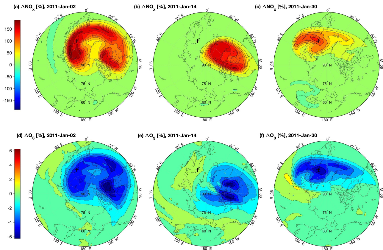
Figure 7. (top row) Relative NO x differences between the full-PsA and no-PsA simulations at ≈40 km altitude, at 12 UT on (a) 2011-Jan-02, (b) 2011-Jan-14, and (c) 2011-Jan-30. The black cross indicates the Tromsø station location. Latitudes from 45°N to 90°N are displayed. (bottom row) As the top row, but for O 3 .
