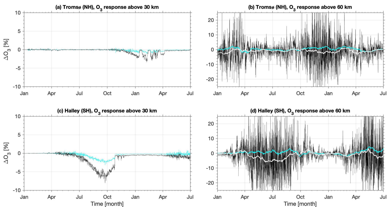
Figure 6. Height-integrated O 3 response to PsA-EEP at the Tromsø and Halley stations. See Figure 4 caption for explanations.
