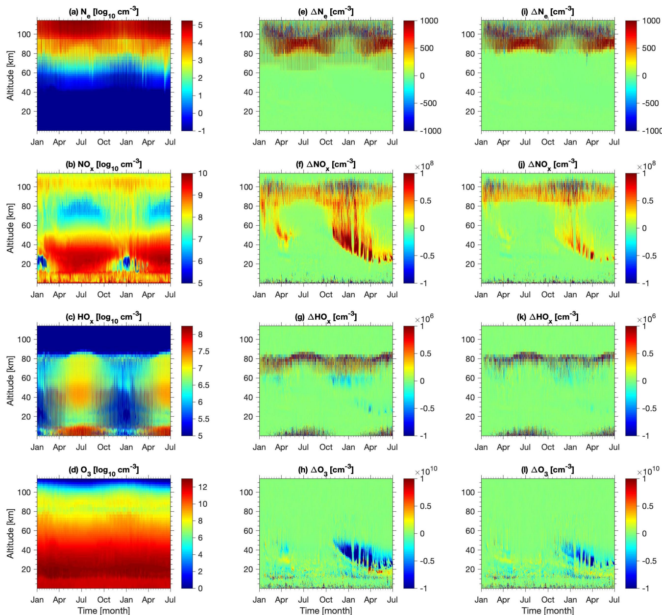
Figure 2. Simulation results for a selected location in the Northern Hemisphere, namely the Tromsø radar site (69.6°N, 19.2°E). Leftmost column: (a) electron concentration N_e , (b) \text{NO}_x , (c) \text{HO}_x , and (d) \text{O}_3 from the full-PsA simulation. Center column: Absolute differences in (e) N_e , (f) \text{NO}_x , (g) \text{HO}_x , and (h) \text{O}_3 between the full-PsA and no-PsA simulation. Rightmost column, panels (i) to (l): as the center column, but showing differences between the thermo-PsA and no-PsA simulation.
