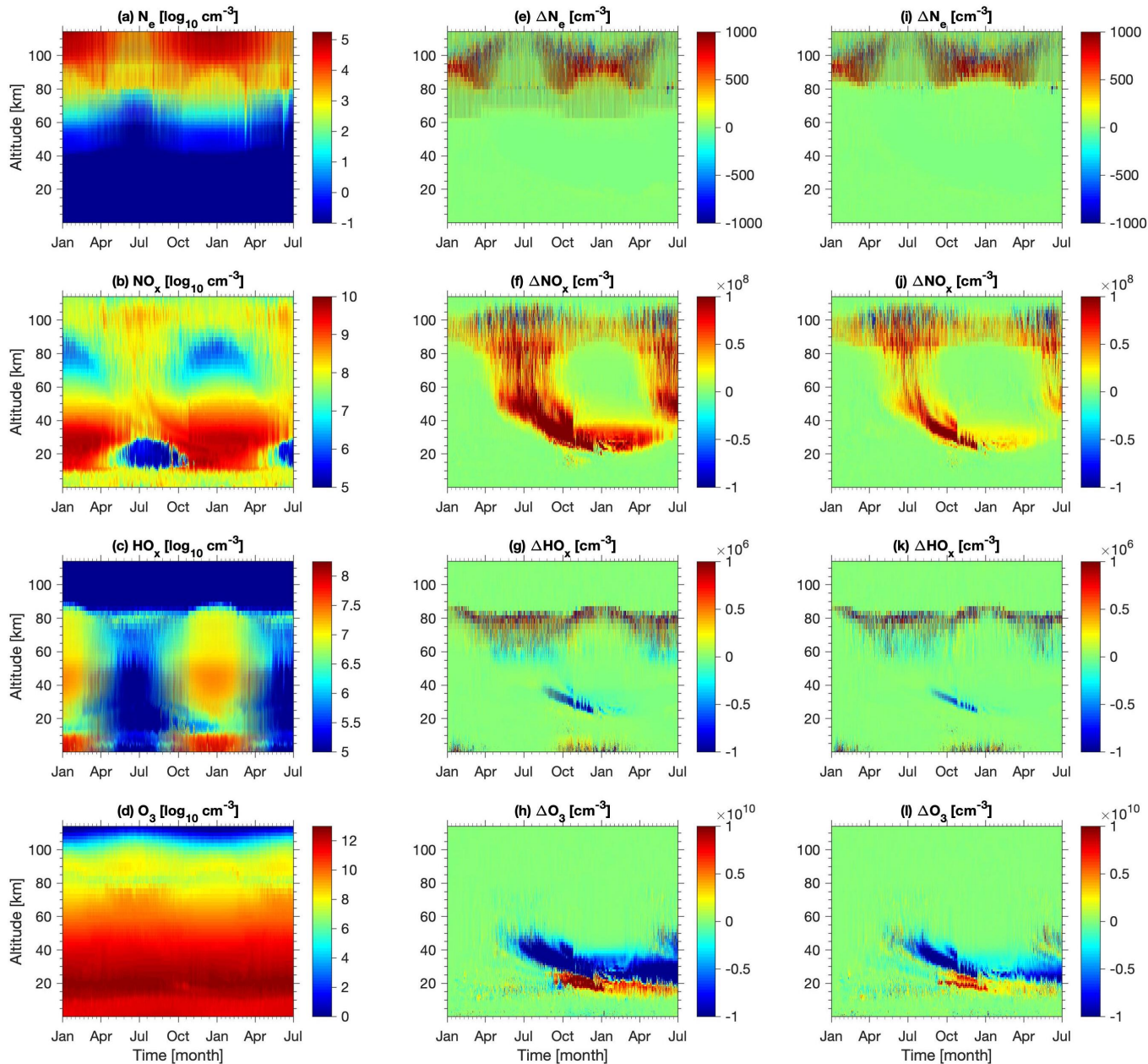
Figure 3. Model results for a selected location in the Southern Hemisphere; Halley Station in Antarctica (75.6°S, 26.6°W). For a description of the panels, see the caption of Figure 2.
