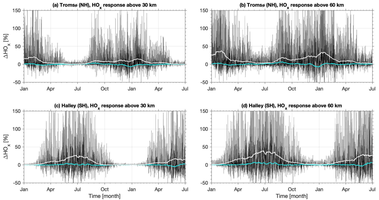
Figure 4. Height-integrated \text{HO}_x response to PsA-EEP at the Tromsø and Halley stations. (black line) The difference between the full-PsA and no-PsA simulations in one-hour resolution. (white line) The 30-day running mean of the black line. (cyan line) The 30-day running mean of the difference between thermo-PsA and no-PsA simulations.
