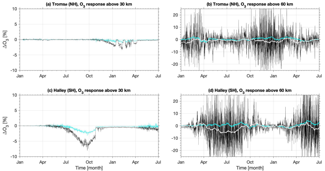
Figure 6. Height-integrated O 3 response to PsA-EEP at the Tromsø and Halley stations. See Figure 4-5 caption for explanations.
