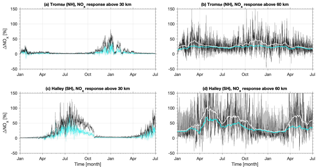
Figure 5. Height-integrated \text{NO}_x response to PsA-EEP at the Tromsø and Halley stations. See Figure (black line, all panels) 4-caption for explanations. The difference between the full-PsA and no-PsA simulations in one-hour resolution. (cyan line, panels a and c) The difference between the thermo-PsA and no-PsA simulations in one-hour resolution. (white line, panels b and d) The 30-day running mean of the black line. (cyan line, panels b and d) The 30-day running mean of the difference between thermo-PsA and no-PsA simulations.
