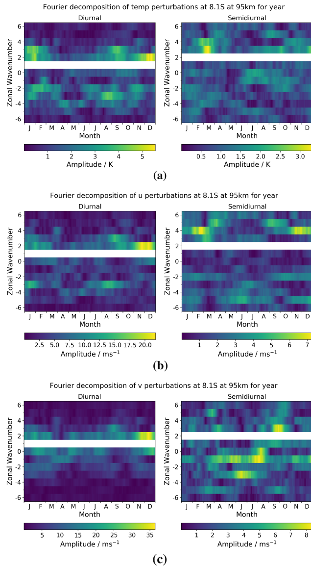
Figure 9. Diurnal and semidiurnal tidal amplitudes as a function of month and zonal wavenumber at the equatorial latitude of Ascension Island ( 8^\circ\text{S} ) for (a) temperature, (b) zonal ( u ) winds and (c) meridional ( v ) winds. The dominant migrating tidal component is removed in each case for clarity.
