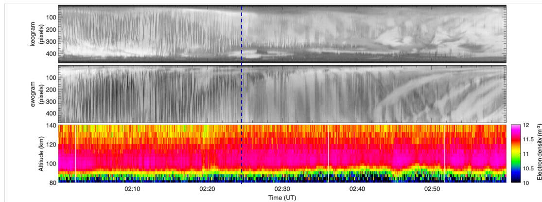
Figure 4. Keogram (top), ewogram (middle), and EISCAT electron density (bottom) from UHF radar at Tromsø-Tromsø on November 09, 2015 between 2 and 3 UT. EISCAT beam points to the centre of the keogram at 235 pixel and in the ewogram at 230 pixel. The electron density is displayed in a logarithmic color scale. The blue dashed vertical line is the separation between APA and PPA.
