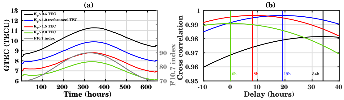
Figure 5. (a) Time series of modeled TEC for the different diffusion conditions K_T \times 0.5 , K_T \times 1.0 (reference), K_T \times 1.5 and K_T \times 2.0 . F10.7 is added as a gray line. (b) Cross-correlation, and the delay between global mean TEC and F10.7 for the different diffusion conditions.
