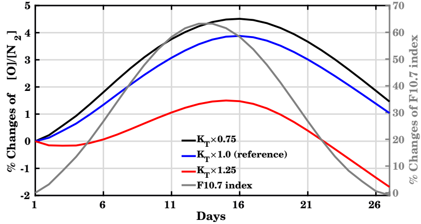
Figure 12. Percentage change of [O]/[N_2] ratio for different diffusion conditions K_T \times 0.75 , K_T \times 1.0 (reference), and K_T \times 1.25 at pressure level 12 at geographic coordinates 40^\circ N/18^\circ E . The right y-axis refers to the percentage change of the F10.7 index (gray curve).
