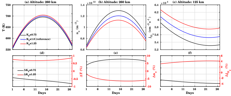
Figure 9. Same as Figure 8 for (a) T , (b) n_e for the pressure level 12 ( \sim 260 km), and (c) j_{O_2} for pressure level 7 ( \sim 125 km).
