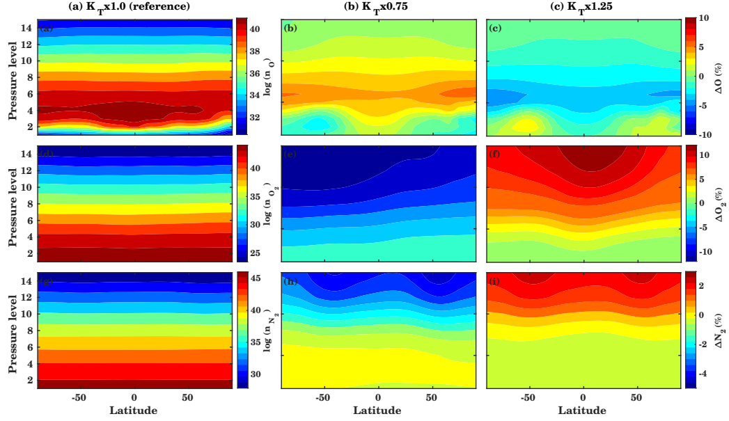
Figure 11. Same as Figure 10, but, for n_O , n_{O_2} , and n_{N_2} .
