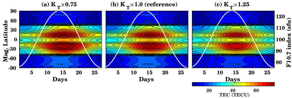
Figure 2. CTIPe simulated daily mean zonal mean TEC for the runs (a) K_T \times 0.75 , (b) K_T \times 1.0 (reference), and (c) K_T \times 1.25 . The white curves show the input F10.7 index.
