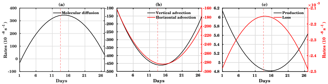
Figure 1. Time series of different terms: (a) molecular diffusion, (b) horizontal advection and vertical advection, and (c) production and loss for atomic oxygen mass mixing ratio. Both the y-axis marked with the corresponding color. The vertical red dashed line represents the middle of the 13 th model day. All the parameters are plotted for pressure level 12 (260 km) for noontime at 40^\circ N/18^\circ E .
