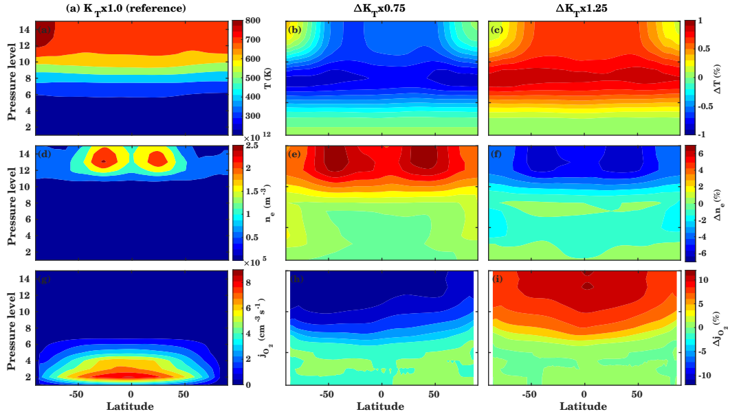
Figure 10. (a) CTIpe simulated T (upper row), n_e (middle row), and j_{O_2} (bottom row), for the 14 th model day. The other columns show the percentage difference between the K_T \times 1.0 simulation and those with modified eddy diffusion conditions: (b) K_T \times 0.75 and (c) K_T \times 1.25 .
