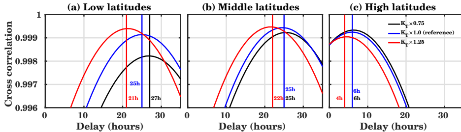
Figure 4. Cross-correlation and delay between regional mean TEC and the F10.7 index at low (a), middle (b), and high (c) geomagnetic latitudes for different runs.
