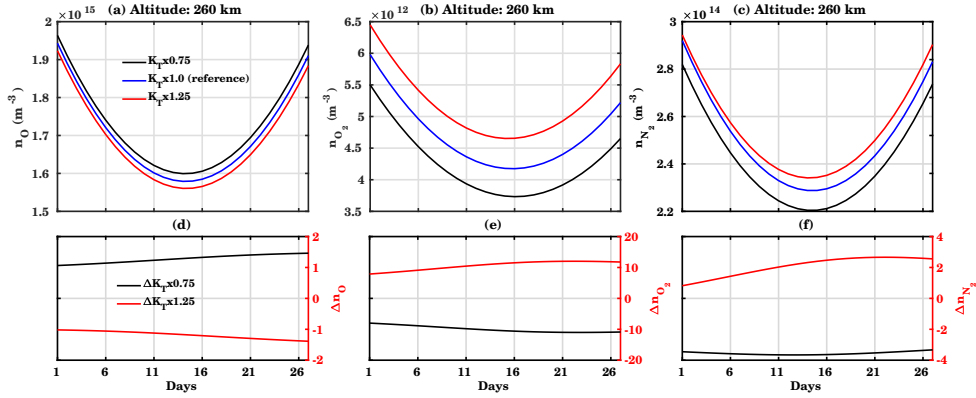
Figure 8. Variation of the CTIpe simulated (a) n_O , (b) n_{O_2} , and (c) n_{N_2} for different diffusion conditions K_T \times 0.75 (black), K_T \times 1.0 (blue) and K_T \times 1.25 (red) (upper panel) for the pressure level 12 (260 km). The percentage difference between the run K_T \times 1.0 (blue curve) and those with modified eddy diffusion conditions K_T \times 0.75 (black), and K_T \times 1.25 (red) are shown in the lower parts of the panels.
