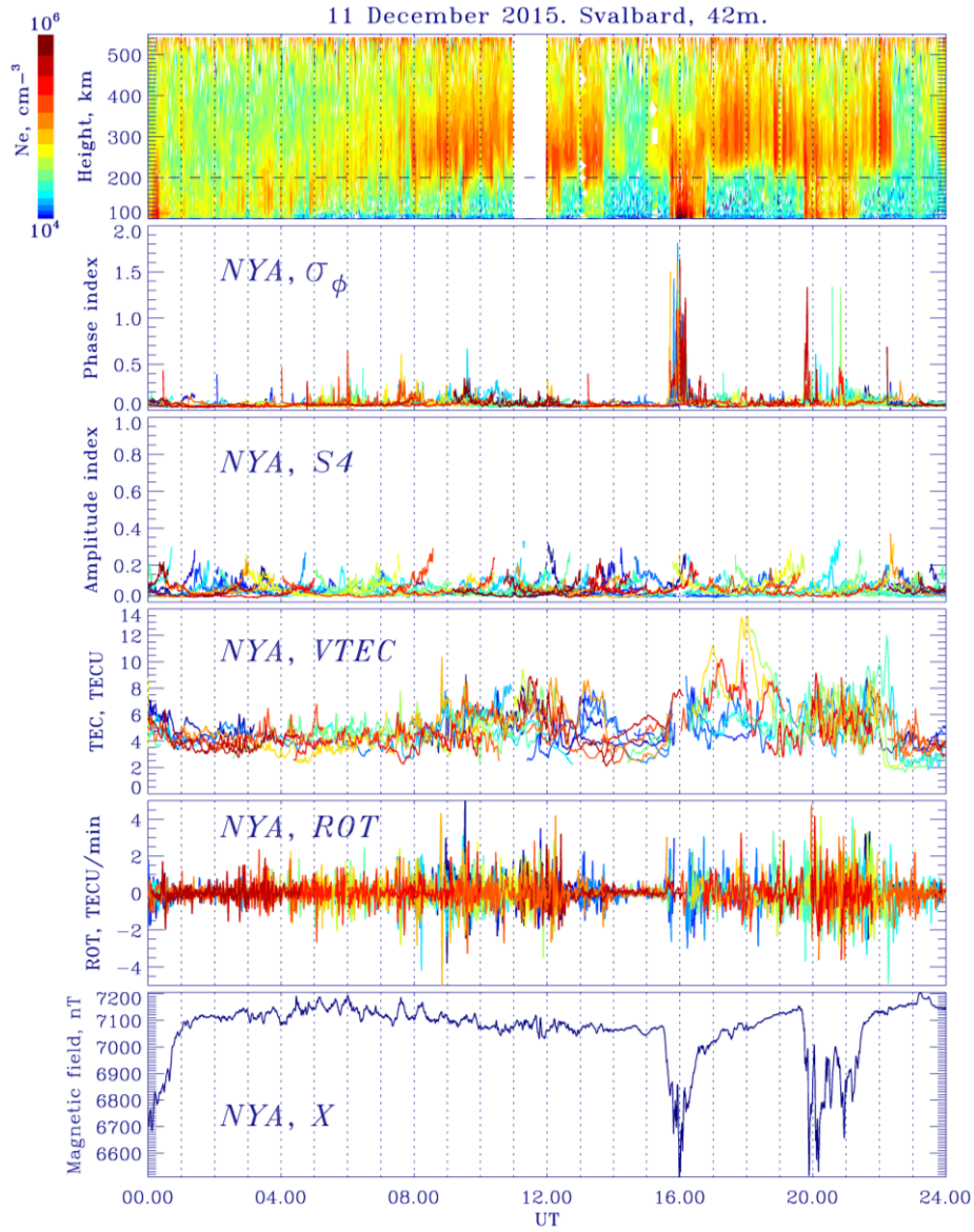
530 Figure 3: Ionosphere plasma density according to the EISCAT 42m radar data; phase scintillation index and amplitude scintillation index according to the GPS receiver at NYA station; TEC and ROT variations according to the GPS receiver at NYA station; geomagnetic field variations (X-component) at NYA station for the 11 December 2015.
