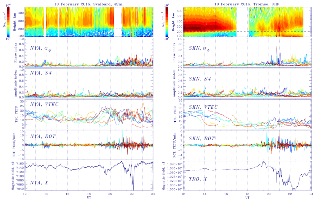
Figure 7: Ionosphere plasma density according to the EISCAT 42m data; phase, amplitude scintillation indexes, TEC and ROT variations according to the GPS receiver at NYA station; X-component of the geomagnetic field at NYA station (left panel). Ionosphere plasma density according to the UHF EISCAT data; phase and amplitude scintillation indexes, TEC and ROT variations according to the GPS receiver at SKN station; X-component of the geomagnetic field at TRO station (right panel) for the 10 February 2015.
