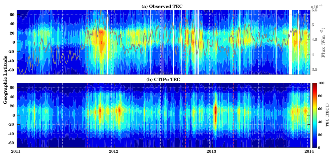
Figure 2. Latitudinal variation of (a) observed TEC and (b) model simulated TEC around noon (11:00-13:00 LT) at 15°E longitude. The gray curve in panel (a) represents the SDO EVE integrated flux (1-120 nm).
