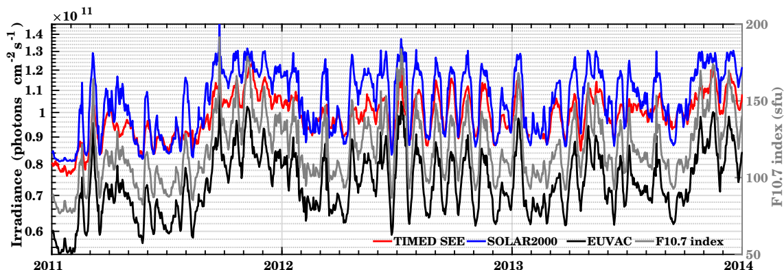
Figure 1. Time series of 0.5 to 105 nm integrated daily irradiance from 2011 to 2013 estimated from TIMED SEE observations, SOLAR2000, and EUVAC. The right y-axis represents the F10.7 index.
