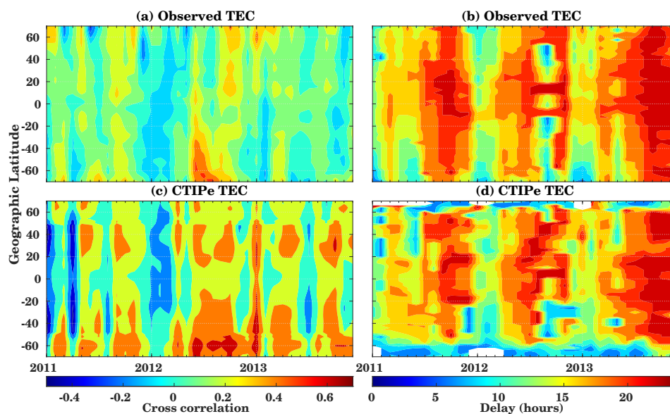
Figure 5. Correlation coefficient (a,c, left panels) and delay estimation (b,d, right panels) using observed (upper panels) and model simulated (lower panels) hourly TEC and SDO EVE integrated flux (1-120 nm).
