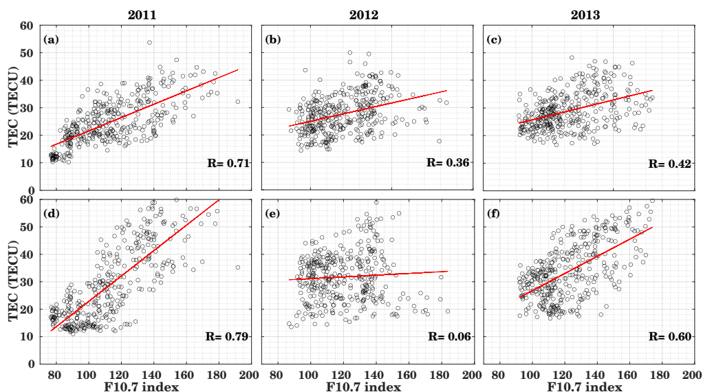
Figure 4. Relation between F10.7 index and mid-day observed TEC (11:00-13:00 LT) at 40^\circ\text{N}/15^\circ\text{E} (upper panel) and 40^\circ\text{S}/15^\circ\text{E} (lower panel) for 2011, 2012 and 2013. The red line is the linear fit.
