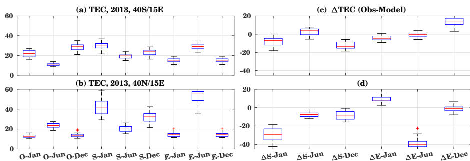
Figure 8. Boxplots of observed daily TEC and model simulated TEC using F10.7A as solar input for 40°S and 40°N during January, June, and December months for the year 2013.
