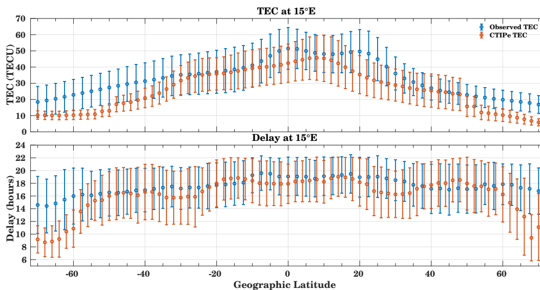
Figure 6. (a) Daily mean TEC variations and (b) delay estimation using observed (blue) and model simulated (red) hourly TEC and SDO EVE integrated flux. The error bars show standard deviations of mean values.
