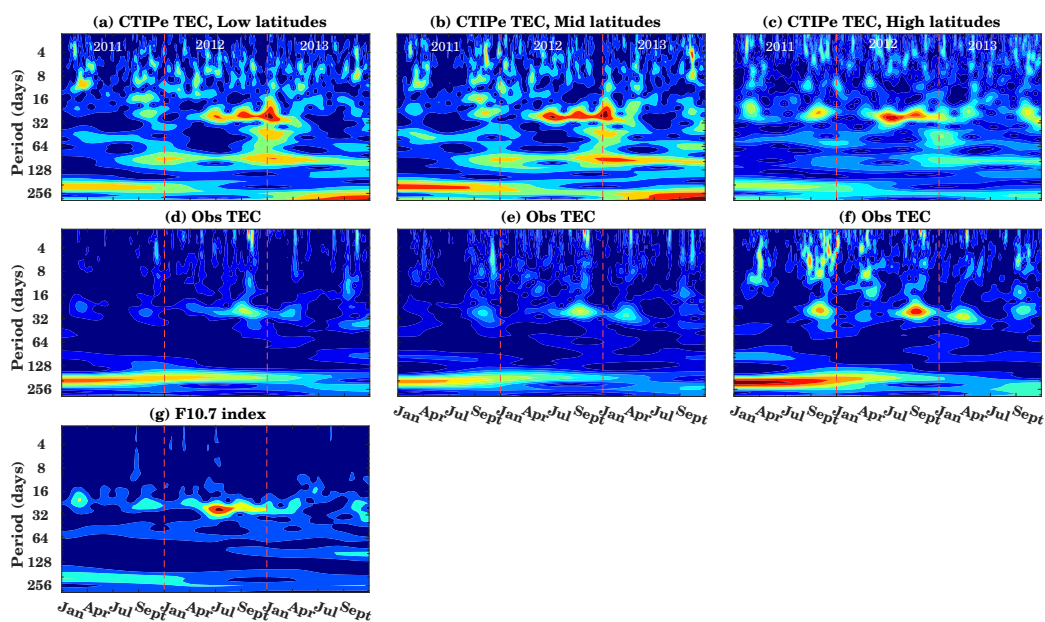
Figure 3. Wavelet continuous spectra of daily model TEC (a-c), observed TEC (d-f) for different low [ \pm 30^\circ ], mid [ \pm(30^\circ - 60^\circ) ], and high [ \pm(60^\circ - 70^\circ) ], and (g) F10.7 index.
