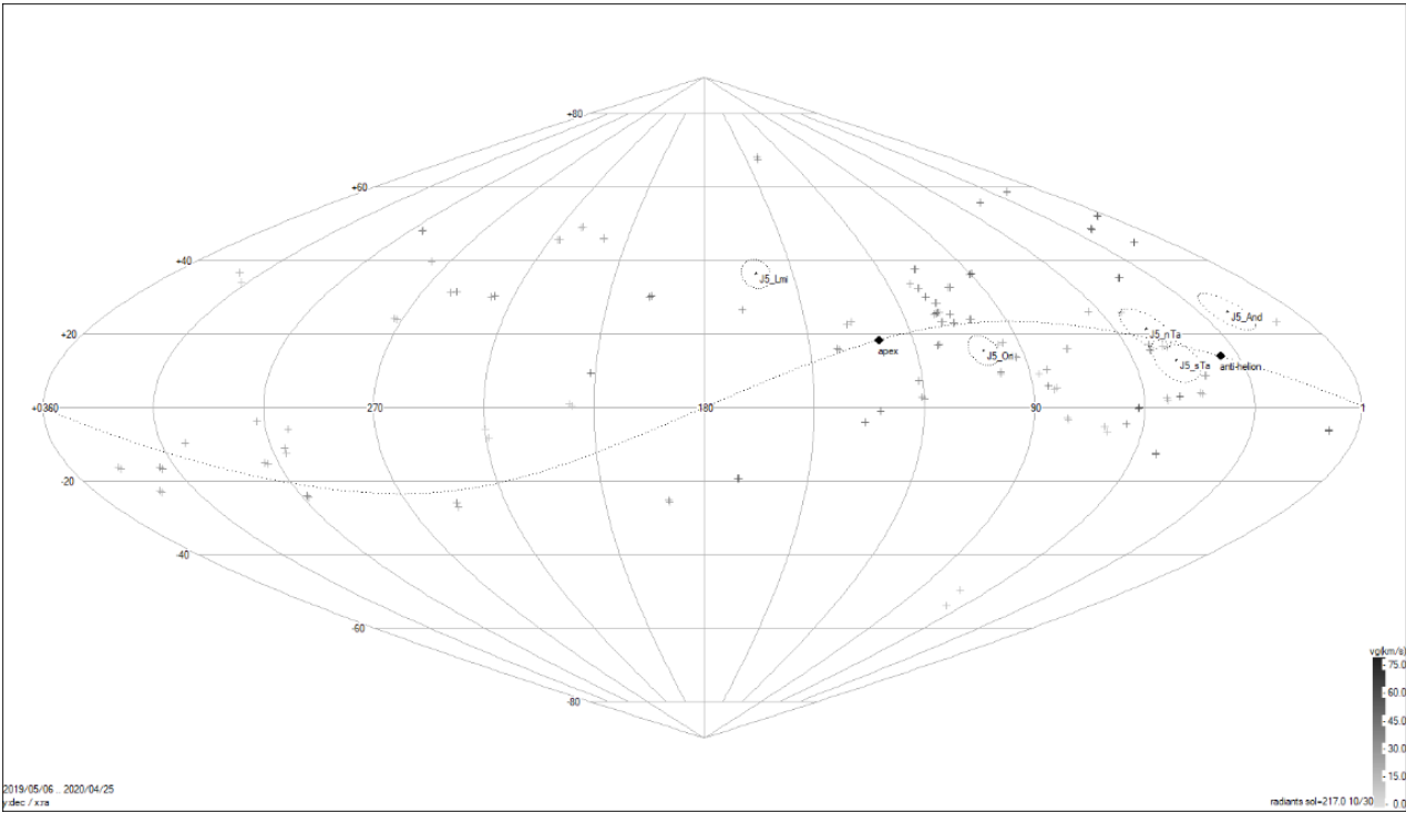
105 Figure 2: A radiant map of meteor observations by the Sharjah and Al-Yahar stations during the period May 2019 – April 2020
