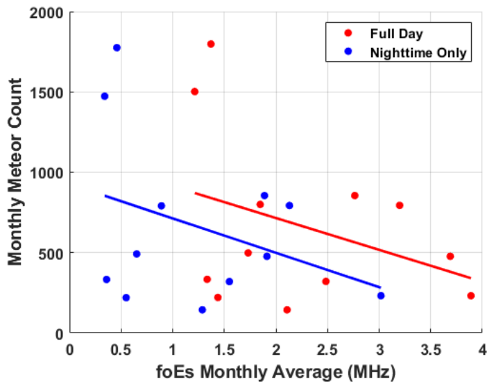
160 Figure 5: Relationship between foEs monthly averages and monthly meteor count observed at Sharjah.
