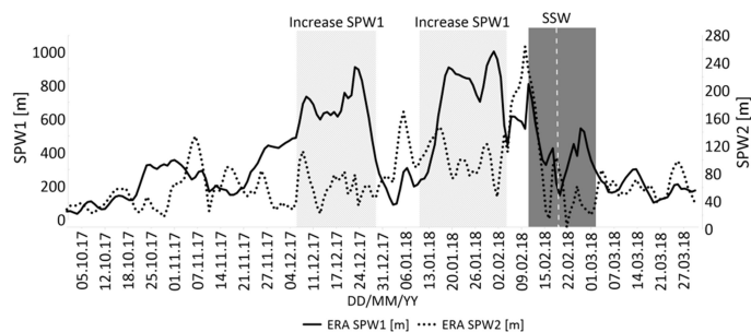
Figure 6: Same as Figure 3, but Oct 2017 through Mar 2018.
