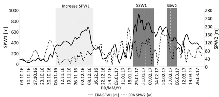
Figure 3: Amplitude of stationary planetary wave 1 at 10 hPa (solid line), and SPW2 amplitude at 10 hPa (dotted line) Oct 2016 through Mar 2017.
