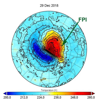
Figure 9: Same as Figure 3, but Oct 2018 through Mar 2019.
