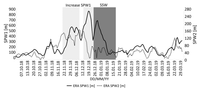
Figure 9: Same as Figure 3, but Oct 2018 through Mar 2019.
