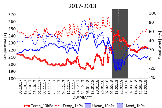
Figure 5: Same as Figure 2, but Oct 2017 through Mar 2018.
