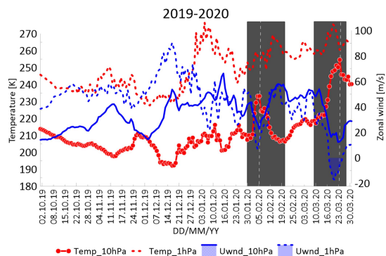
155 Figure 11: Same as Figure 2, but Oct 2019 through Mar 2020.
