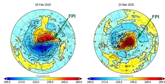
Figure 12: Same as Figure 3, but Oct 2019 through Mar 2020.
