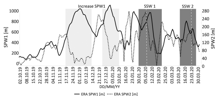
Figure 12: Same as Figure 3, but Oct 2019 through Mar 2020.
