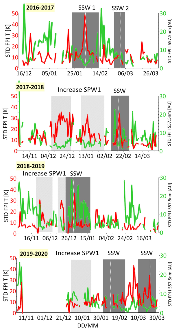
235 Figure 17: FPI-measured standard deviation of the 557.7-nm emission (green line), of the temperature (red line), the period of the SPW1 amplitude increase (light grey rectangle), the SSW periods (grey rectangle), and the day of the SSW maximal temperature (dotted white vertical line).
