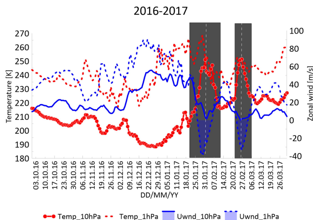
Figure 2: Zonal mean of the zonal wind at 10 hPa (blue solid line) and 1 hPa (blue dotted line), and zonal mean temperature at 10 hPa (red solid line) and 1 hPa (red dotted line) obtained from ERA5 reanalysis dataset Oct 2016 through Mar 2017.
