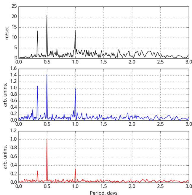
Figure 16: LS periodogram of zonal wind (U) from the 2017-2018 FPI measurements.
