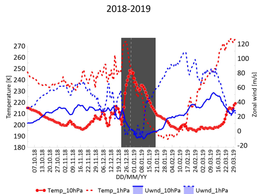
140 Figure 8: Same as Figure 2, but Oct 2018 through Mar 2019.
