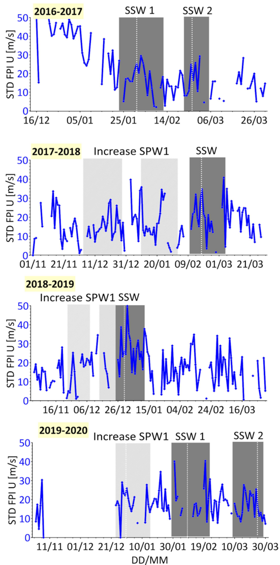
240 Figure 18: FPI-measured standard deviation of zonal wind, the period of the SPW1 amplitude increase (light grey rectangle), the SSW periods (grey rectangle), and the day of the SSW maximal temperature (dotted white vertical line).
