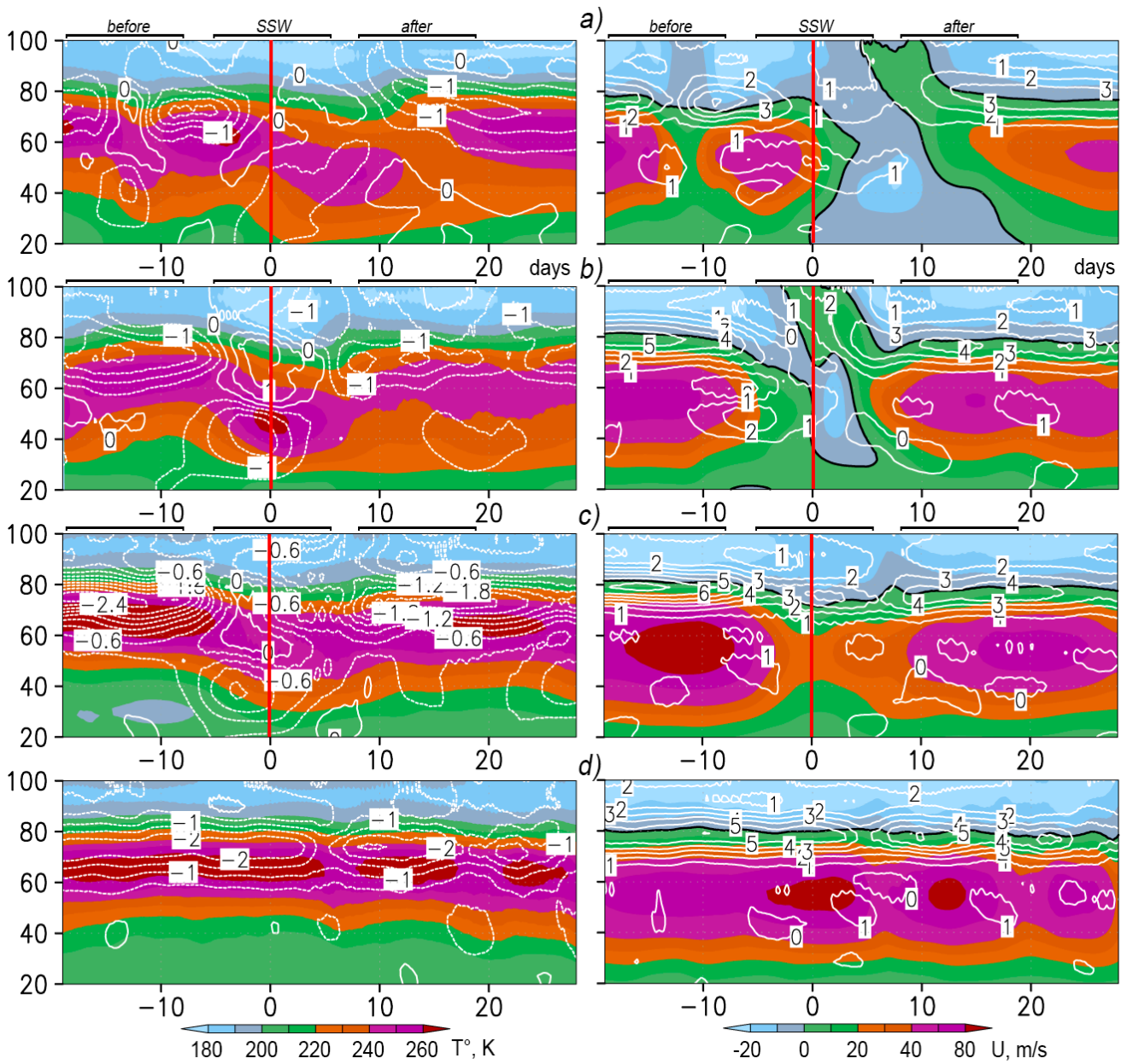
Figure 1: Examples of simulated zonal-mean temperature in K averaged over latitudinal band of 82 – 87° N (shaded left) and zonal-mean zonal wind in m/s at 62° N (shaded right) for MUAM runs with different phases of stratospheric vacillations. Panels a – d show, respectively, major SSW, HSW, minor SSW and a MUAM run without stratospheric warming. Contours show residual vertical velocity in cm/s (left) and residual meridional velocity in m/s (right) at respective latitudes (negative - dashed). Zero days correspond to the respective SSW onset dates. Horizontal lines above the plots show time intervals before, during and after SSW.
