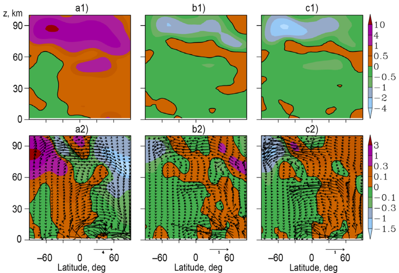
Figure 3: Zonal-mean residual meridional velocity in m/s (a1) and vertical velocity in cm/s (a2) averaged over 19 MUAM runs for 11-day intervals before the composite SSW and add-ons of respective quantities at the time intervals during SSW (b) and after SSW (c). Arrows show vectors with components r \cdot F_x^* and 100 \cdot r \cdot F_z^* in \text{kg} \cdot \text{m}^{-2} \cdot \text{s}^{-1} , which schematically
