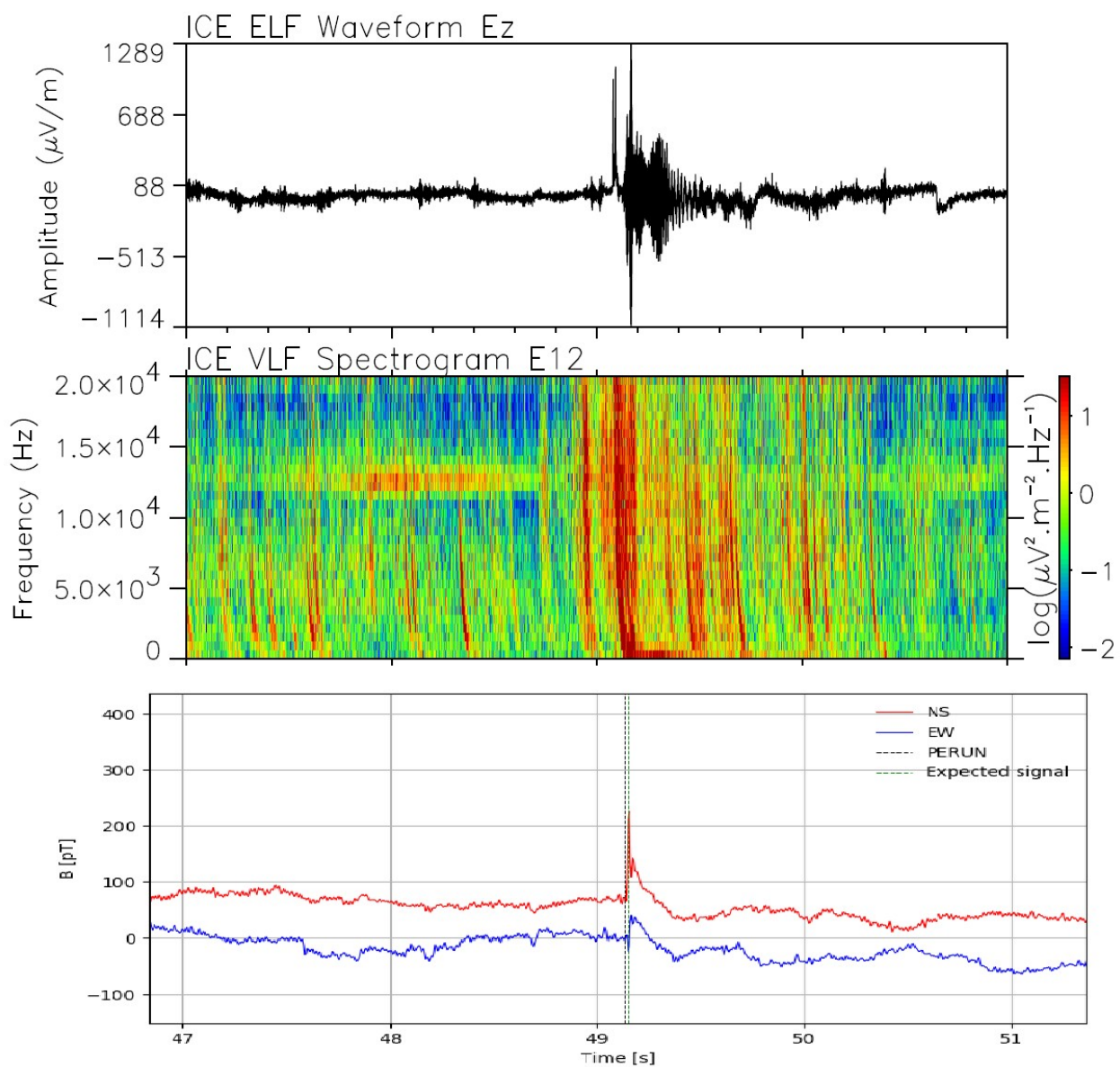
150 Figure 3 Comparison of DEMETER and Hylaty results. Top panel presents the waveform of the electric field in the ELF range, the middle panel shows a spectrogram of the electric field in VLF range both registered by DEMETER and the bottom panel presents the magnetic field in the ELF range in time interval 20:05:47-20:05:51 - 23 July 2009.
