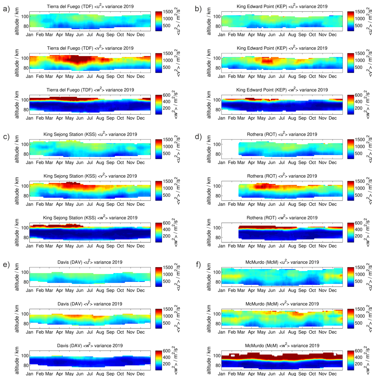
Figure 9. Same as Figure 8, but for the zonal, meridional and vertical wind variances.
