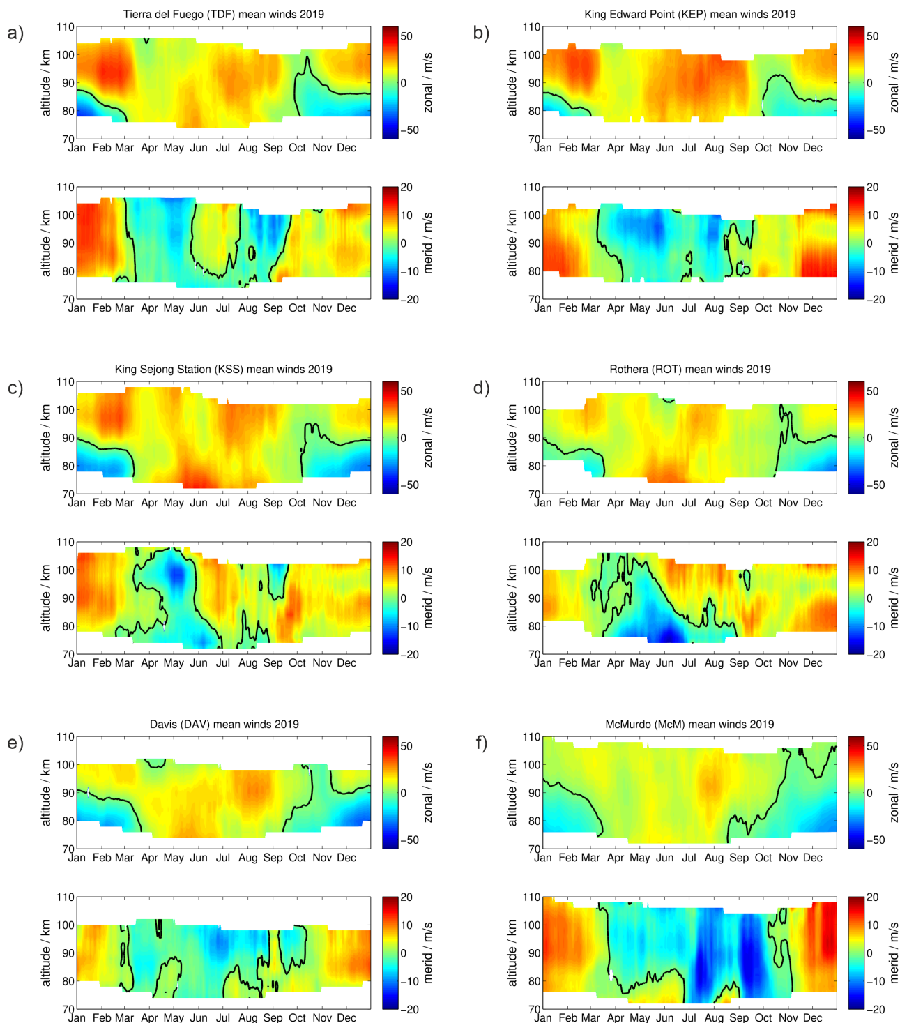
Figure 2. Comparison of zonal and meridional mean winds for each station during the year 2019 for a) TDF, b) KEP, c) KSS, d) ROT, e) DAV and f) MCM.
