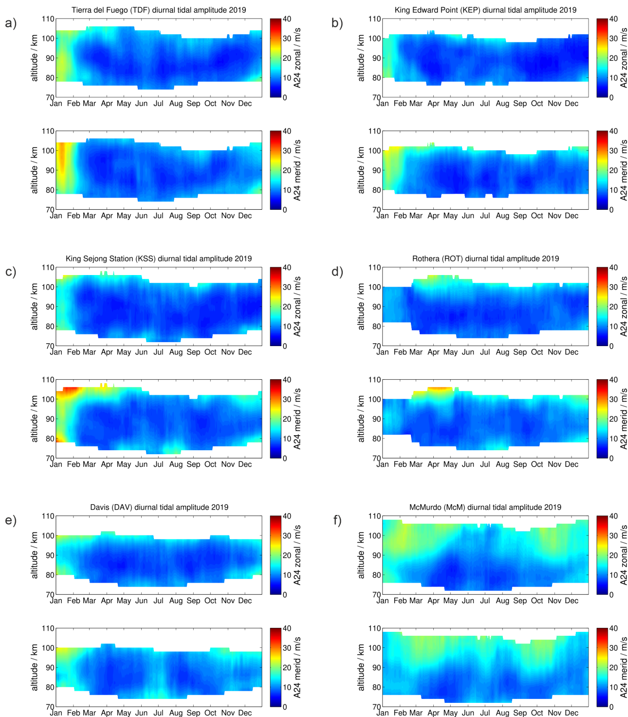
Figure 3. Same as Figure 2 but for the diurnal tidal amplitudes.
