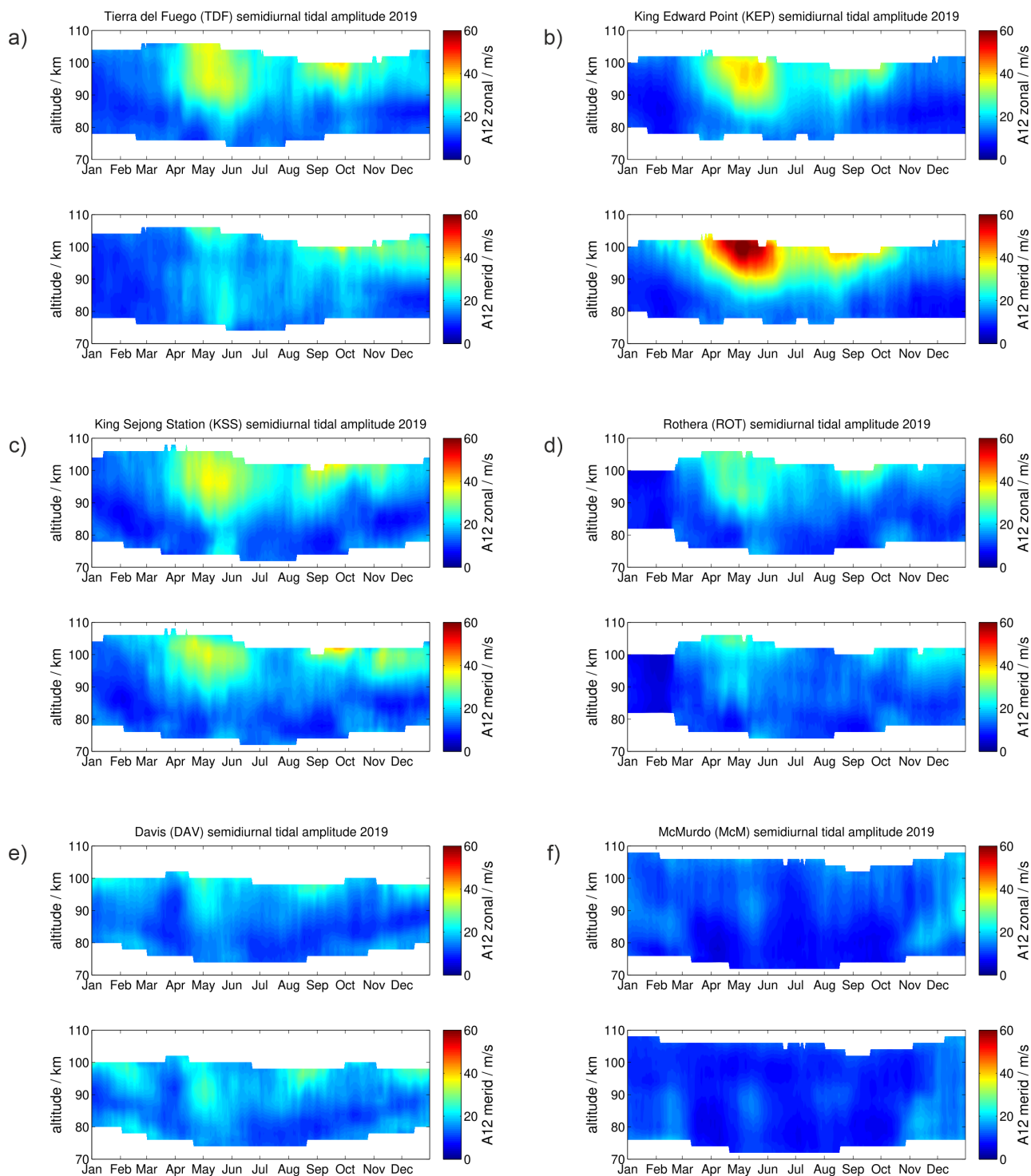
Figure 5. Same as Figure 2 but for the semidiurnal tidal amplitudes.
