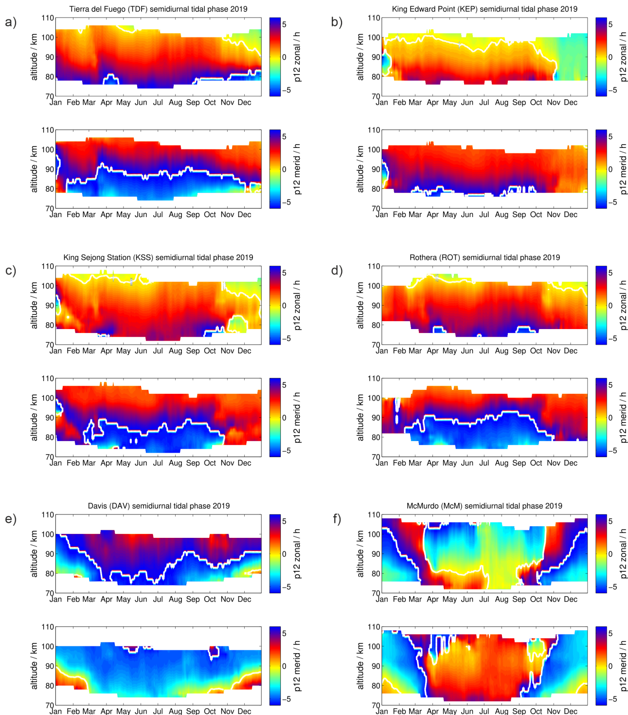
Figure 6. Same as Figure 2 but for the semidiurnal tidal phases.
