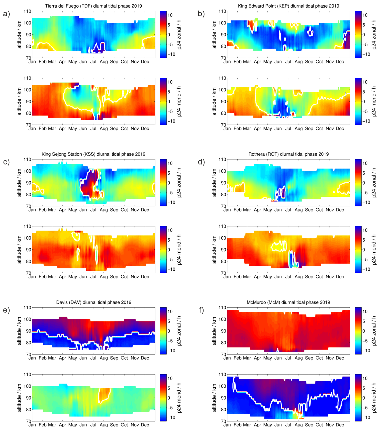
Figure 4. Same as Figure 2 but for the diurnal tidal phases.
