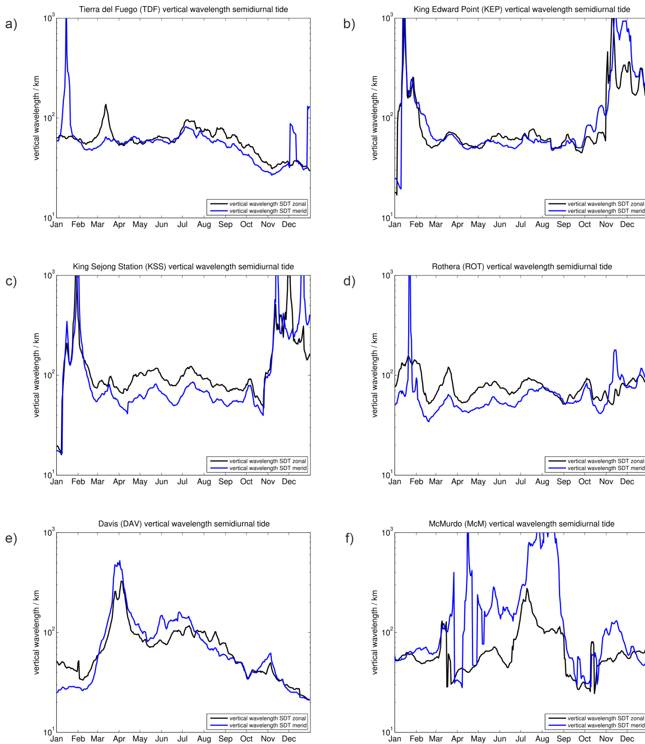
Figure 7. Same as Figure 2 but for the semidiurnal tidal vertical wavelengths.
