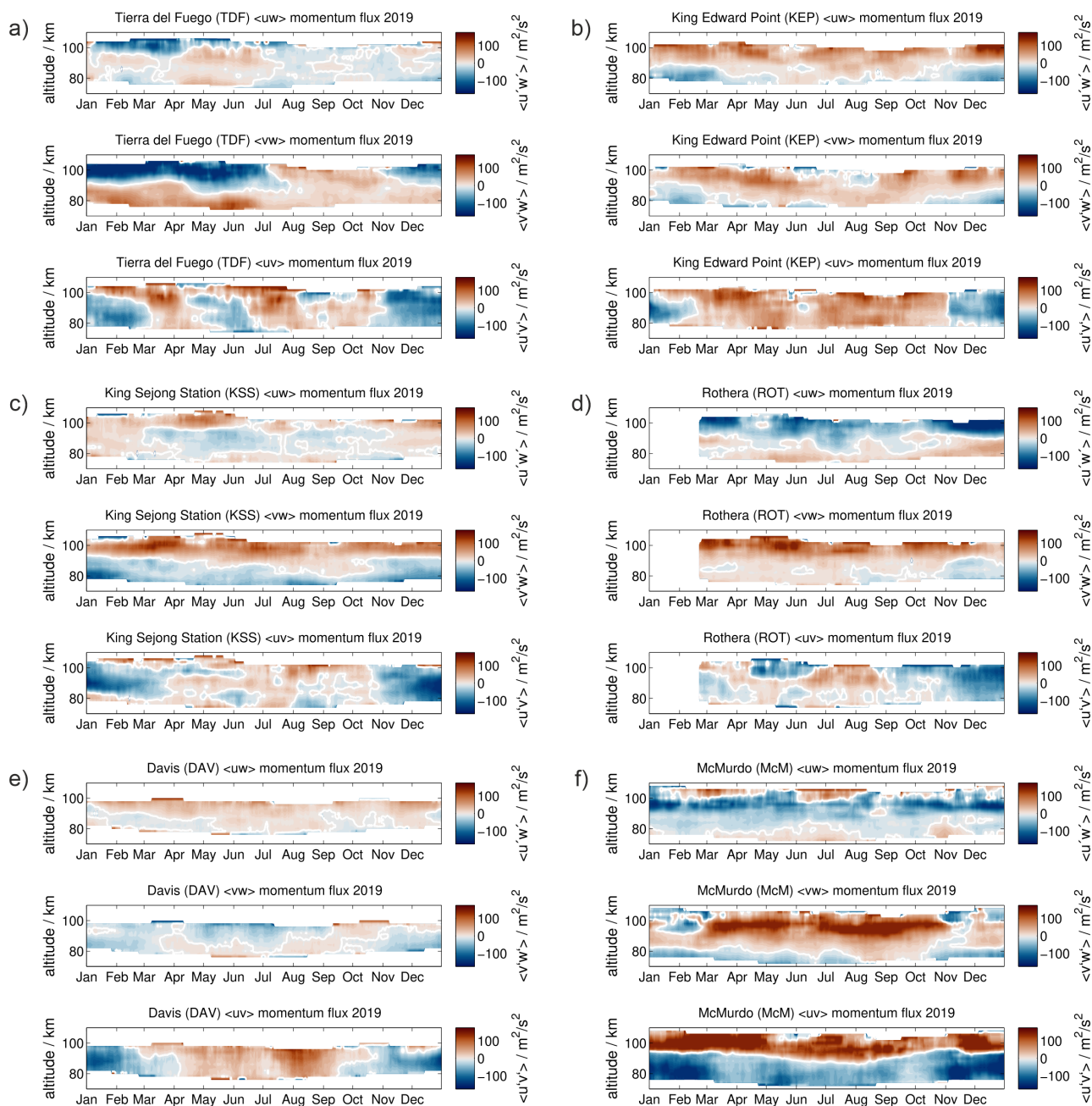
Figure 8. Comparison of vertical flux of zonal and meridional momentum and horizontal momentum flux for each station during the year 2019 for a) TDF, b) KEP, c) KSS, d) ROT, e) DAV and f) MCM.
