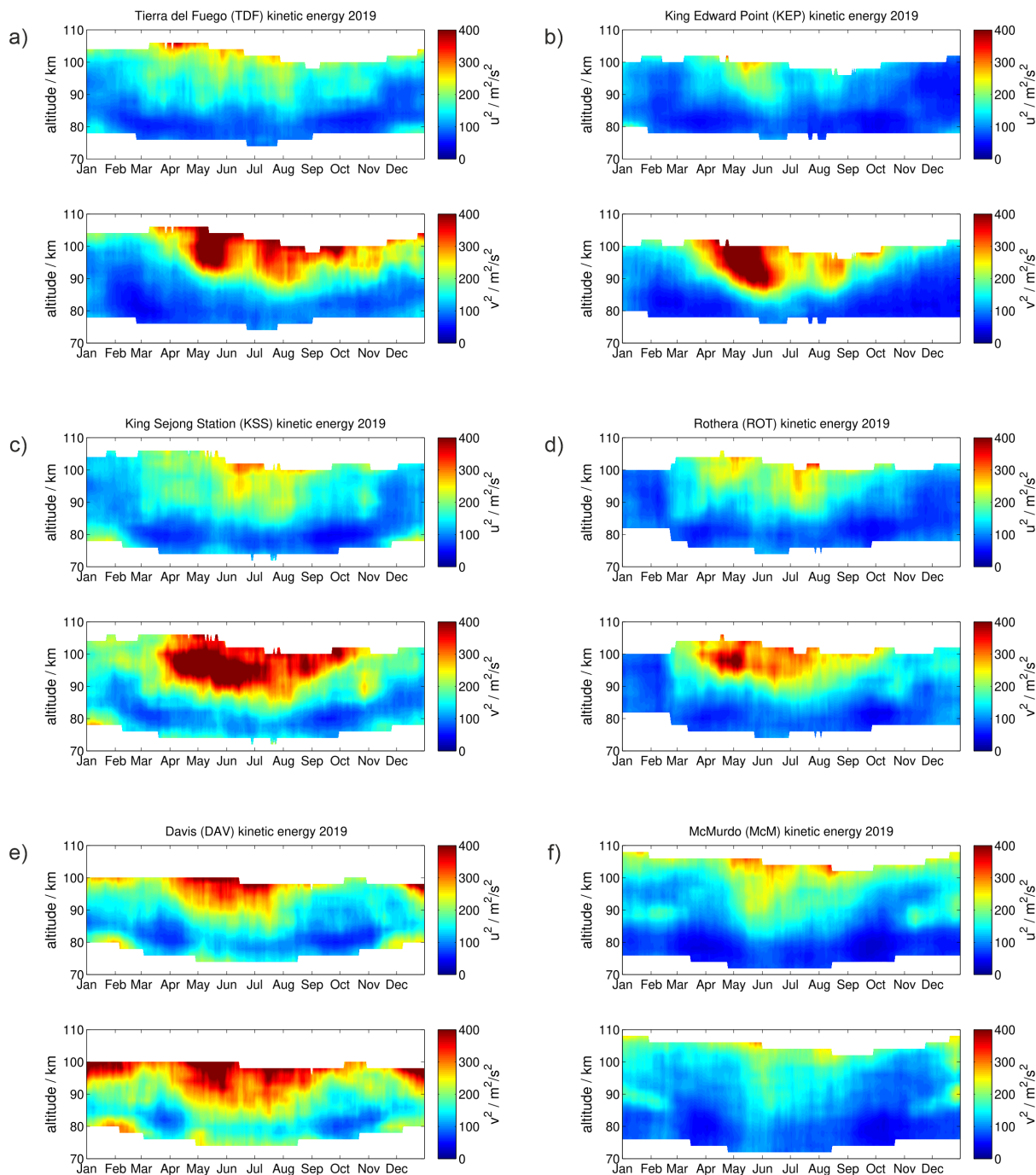
Figure A2. Kinetic gravity wave energy as determined for the resolved waves from the ASF for each station during the year 2019 for a) TDF, b) KEP, c) KSS, d) ROT, e) DAV and f) MCM.
