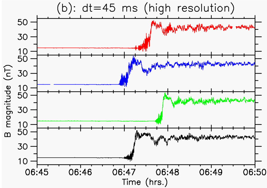
165 Figure 1. Total magnetic field amplitude measured versus time during the same shock crossing by each of the 4 Cluster satellites on 04/22/2001 around 0647 UT ( M_A = 3.8 ; \beta_i = 0.04 so that v_{sh}/v_{thi} \gg 1 , \theta_{Bn} = 89^\circ ). The same measurement is performed at low time resolution ( dt=4s in panel (a)) and high time resolution ( dt=45 ms in panel (b)).
