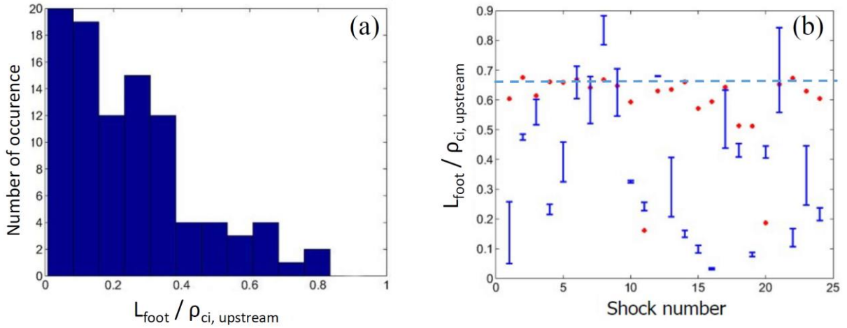
Figure 9: (a) Distribution of the 96 shock crossings versus the foot thickness (normalized versus the upstream ion gyroradius \rho_{ci, \text{upstream}} ); (b) Distribution of the largest experimental foot thickness (normalized versus the upstream ion gyroradius \rho_{ci, \text{upstream}} ) for every shock event; the vertical bars correspond to the error estimate made on the measured values in blue, and the red dots correspond to the upper bound values i.e. the theoretical values obtained from Eq. (1-3) of Sect. 4.3 (i.e., Eq. 3 of Gosling and Robson, 1985). For reference, the value L_{\text{foot}} / \rho_{ci, \text{upstream}} = 0.68 defined for \theta_{Bn} = 90^\circ (Woods, 1971) is indicated by the light blue horizontal dashed line in panel (b).
