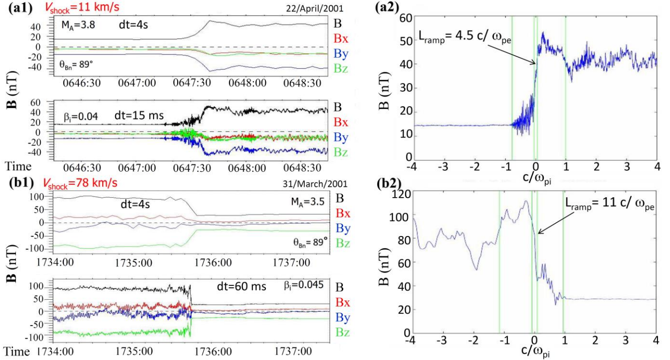
Figure 6: Comparison of a slow moving shock (panels (a1) and (a2), where v_{sh} = 11 km/s, M_A = 3.8 , \theta_{Bn} = 89^\circ , and \beta_i = 0.04 ) and a rapid shock (panels (b1) and (b2), where v_{sh} = 78 km/sec, M_A = 3.5 , \theta_{Bn} = 89^\circ , and \beta_i = 0.045 ) defined for low ( dt=4 s) and high resolution rates ( dt=15 or 60 ms). Panels (a1) and (b1) provide the temporal profiles of the total magnetic field amplitude (defined respectively for C1 and C3, while panels (a2) and (b2) provide correspondingly the spatial profiles of the measured magnetic field (the distance is normalized with respect to the ion inertial length defined upstream). The spatial origin corresponds to the location at the middle time of the ramp crossing interval for each satellite.
